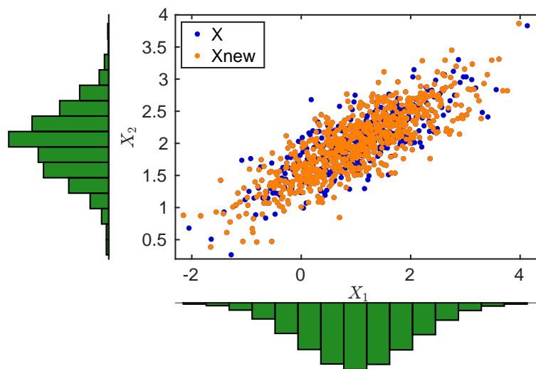
Figure 19: Enrichment of the LHS samples drawn from a 2-D Gaussian distribution with a Gaussian copula using uq_enrichLHS . The initial sample set is shown in Figure 18.
