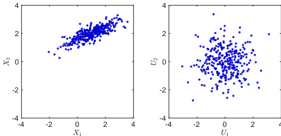
Figure 20: An isoprobabilistic transform from some physical space (2D Gaussian) to the standard normal space.
