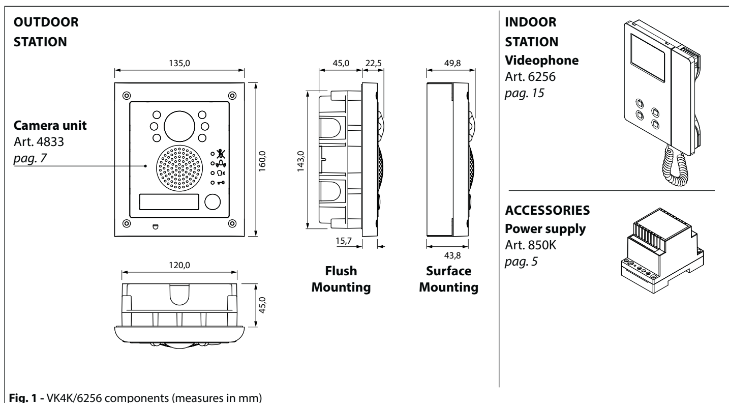
Fig. 1 - VK4K/6256 components (measures in mm)
