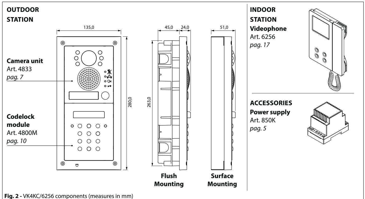
Fig. 2 - VK4KC/6256 components (measures in mm)
