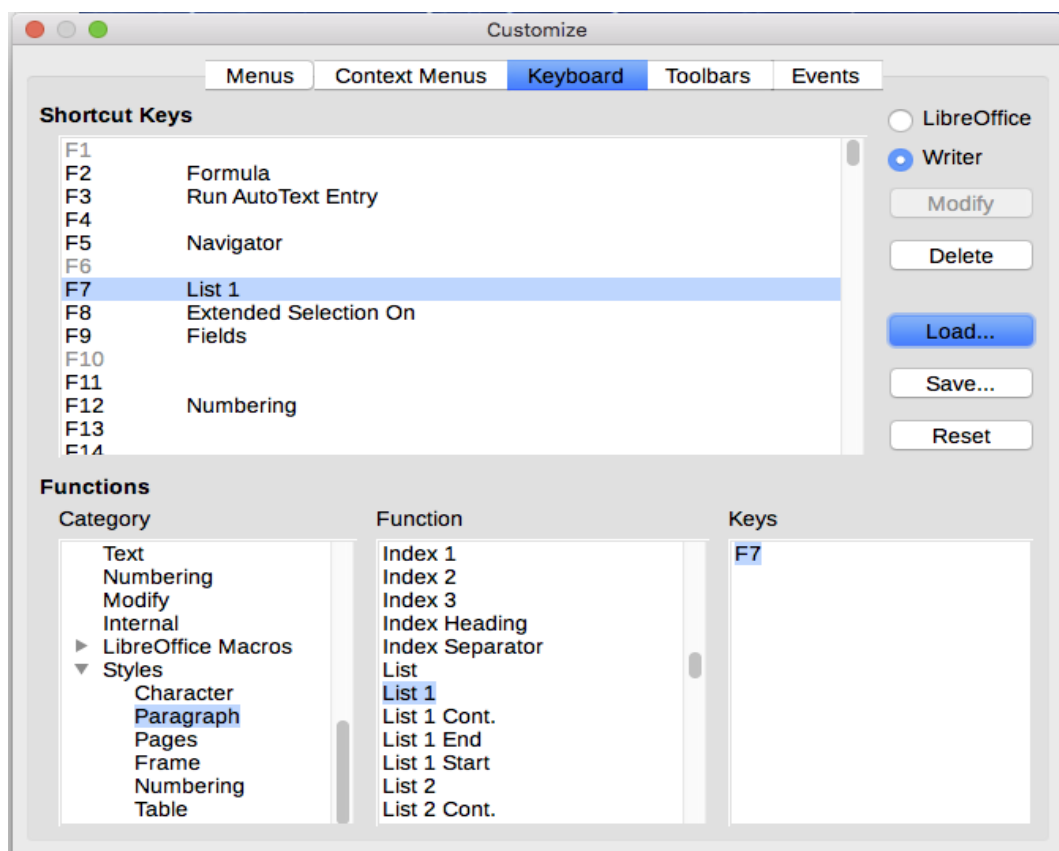
Figure 447: Defining keyboard shortcuts for applying styles
