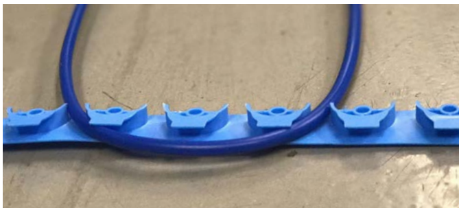
Plastic fixing strips (PLG-DCM-12) holding the DCM-PRO Cable.
