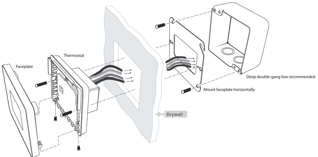
Close-up of the double-gang box with faceplate
