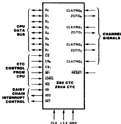
Figure 1. Pin Functions
