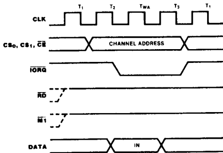
Figure 10. Write Cycle Timing
