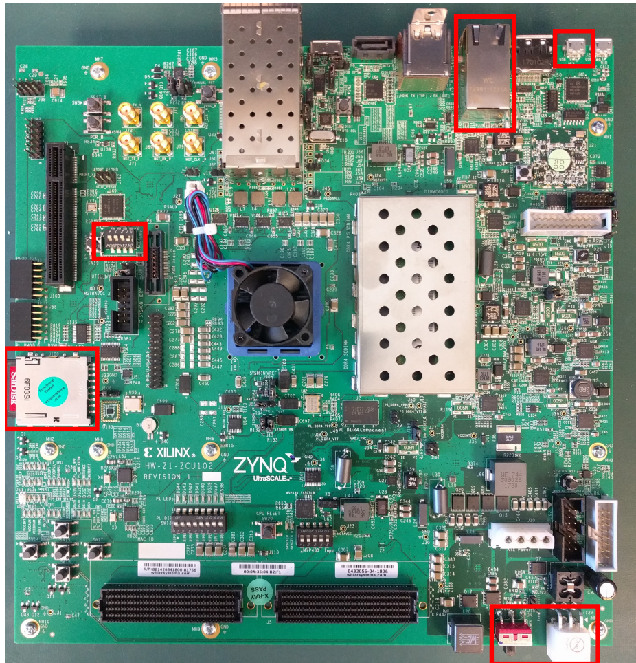
Figure 1: Top View (ZCU102)
