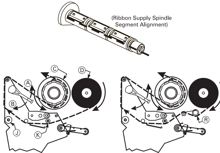
Figure 4 • Ribbon Loading
