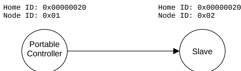
Figure 24. Including a Slave node.
