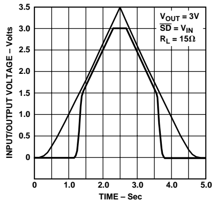
Figure 9. Power-Up/Power-Down
