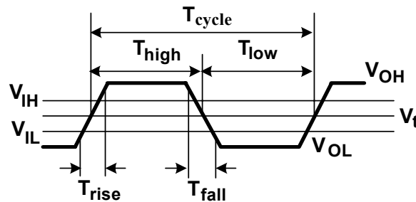
Figure 18. Output Timing
