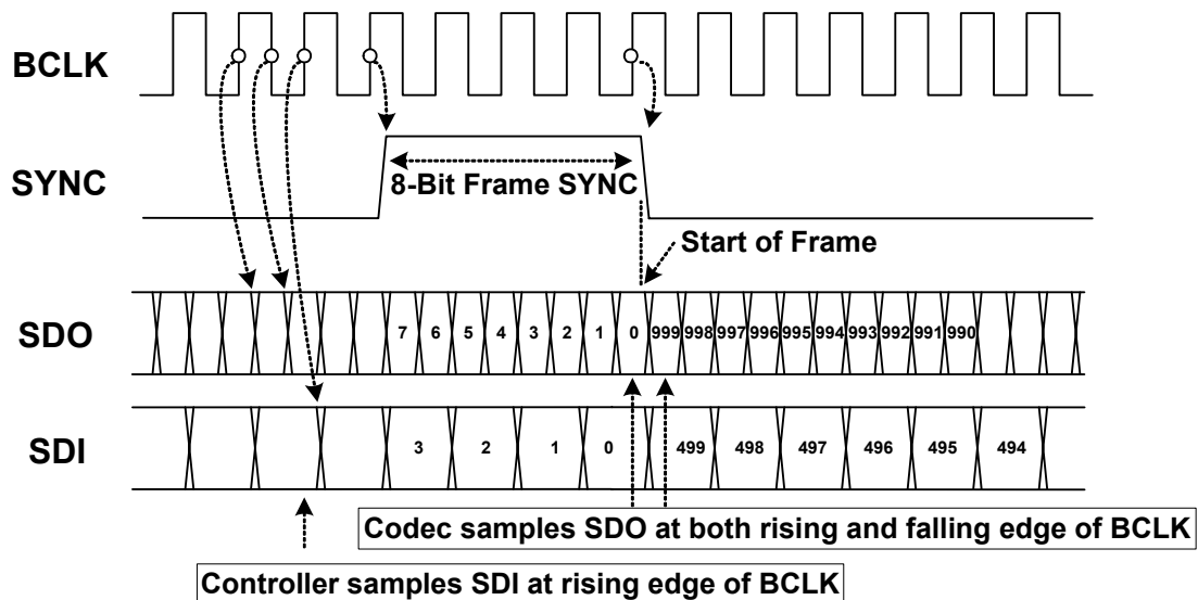
Figure 6. Bit Timing
