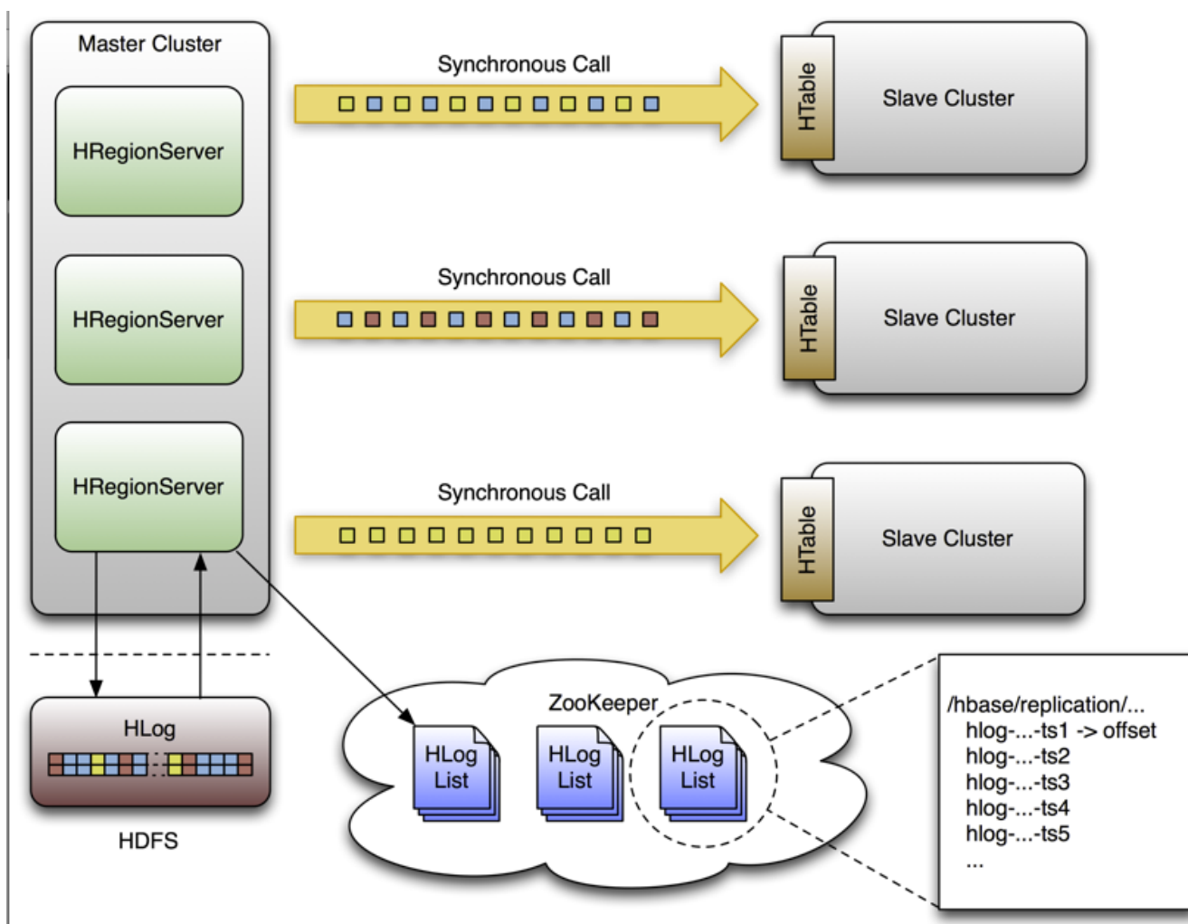
Figure 17. Replication Architecture Overview
