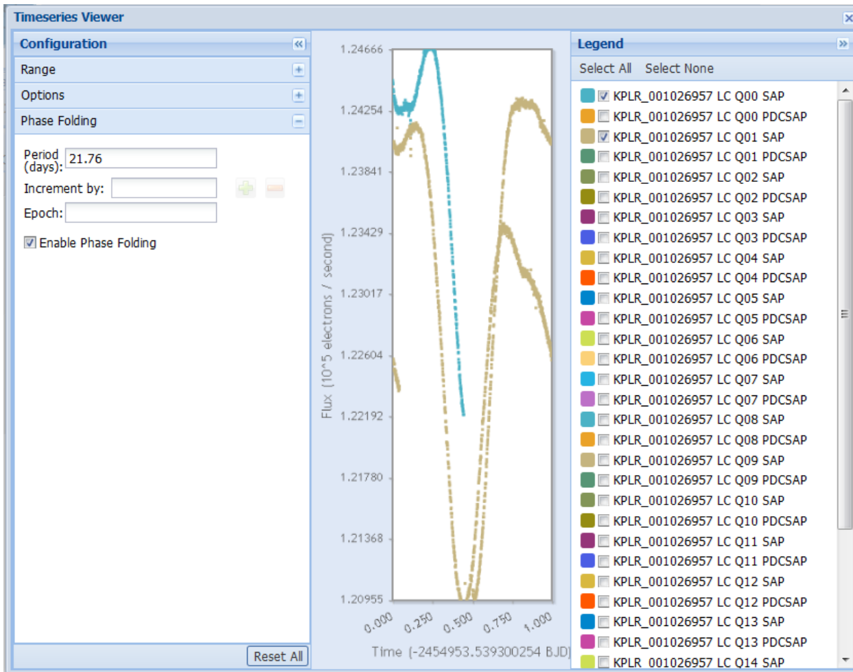
Figure 3-5 Phase folded Q0 and Q1 SAP light curves for KIC1026957. The period used is 21.76 days.
