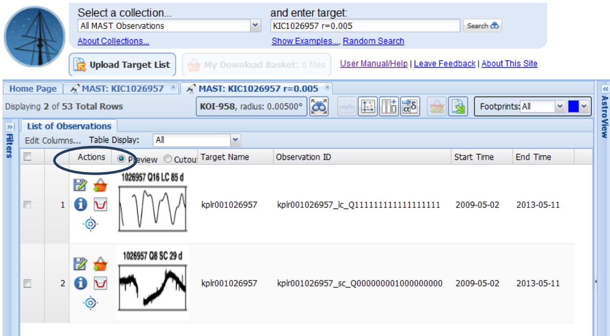
Figure 3-4 Filtered Portal results for KIC1026957.
