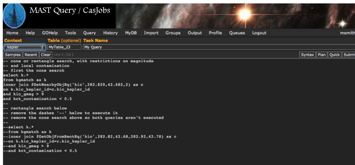
Figure 3-16 The Kepler/GALEX CasJob form. This page can be used to formulate sophisticated queries to constrain a class of objects. This example shows a comment-annotated query for selection of matching objects around a designated area in the sky from the Complete table.
