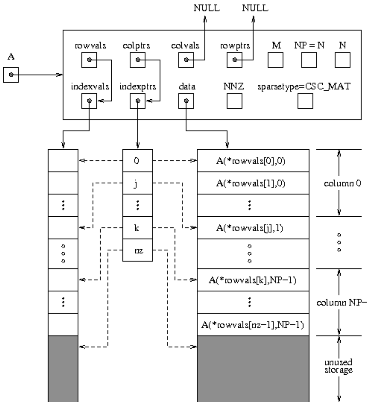
Fig. 10.2: Diagram of the storage for a compressed-sparse-column matrix of type SUNMATRIX_SPARSE: Here A is an M \times N sparse CSC matrix with storage for up to NNZ nonzero entries (the allocated length of both data and indexvals ). The entries in indexvals may assume values from 0 to M-1 , corresponding to the row index (zero-based) of each nonzero value. The entries in data contain the values of the nonzero entries, with the row i , column j entry of A (again, zero-based) denoted as A(i, j) . The indexptrs array contains N+1 entries; the first N denote the starting index of each column within the indexvals and data arrays, while the final entry points one past the final nonzero entry. Here, although NNZ values are allocated, only nz are actually filled in; the greyed-out portions of data and indexvals indicate extra allocated space.
