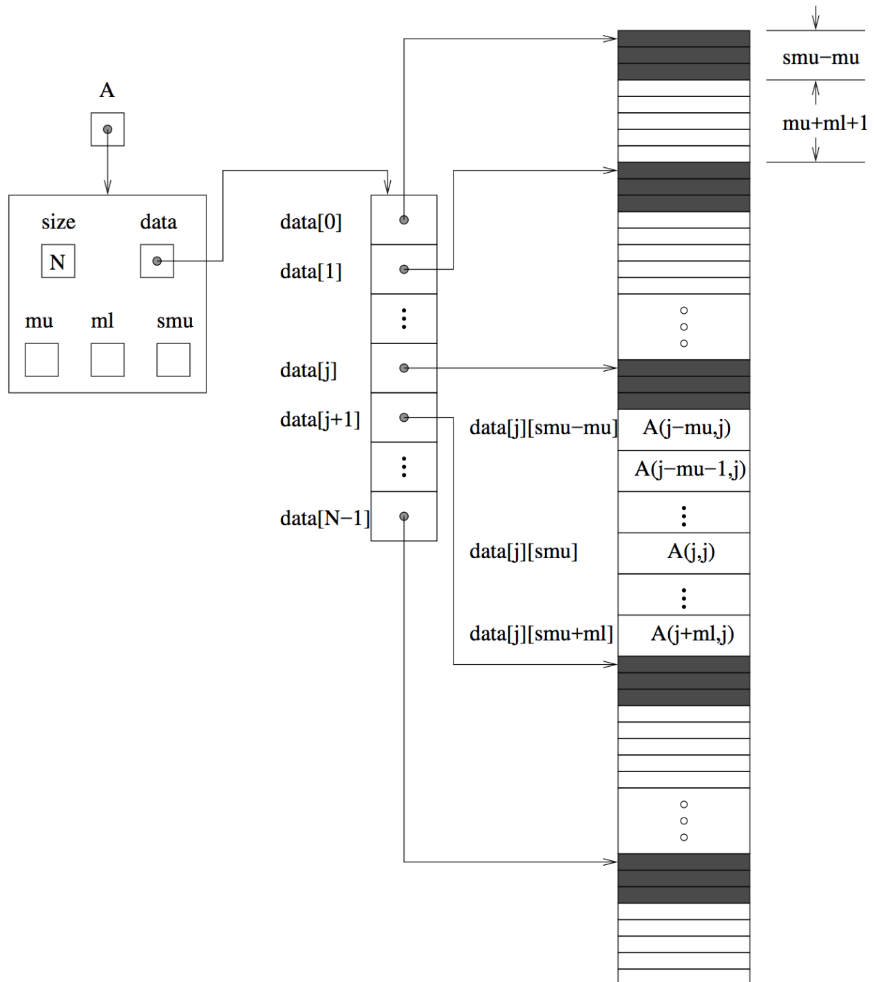
Fig. 10.1: Diagram of the storage for the SUNMATRIX_BAND module. Here A is an N \times N band matrix with upper and lower half-bandwidths mu and ml , respectively. The rows and columns of A are numbered from 0 to N-1 and the (i, j) -th element of A is denoted A(i, j) . The greyed out areas of the underlying component storage are used by the associated SUNLINSOL_BAND or SUNLINSOL_LAPACKBAND linear solver.
