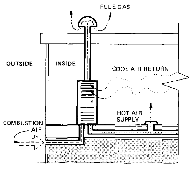
19. Furnace Operation. There are two distinct air flows in the operation of a gas-fired, forced-air furnace: (1) combustion air intake and flue gas exhaust and (2) the heating air supply and return.
