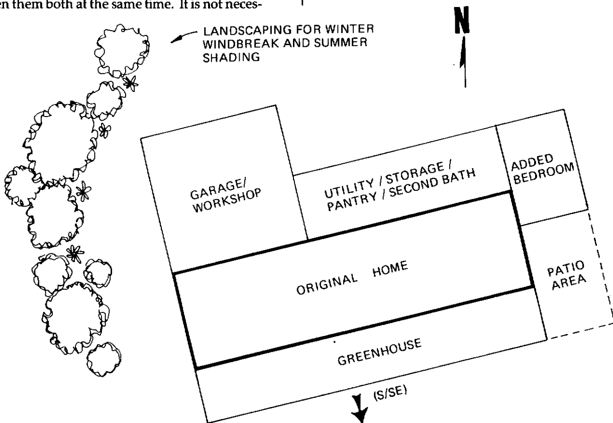
29. Home Additions. Well-designed and well-placed additions can result in an energy-efficient site-built home. The greenhouse and garage can be used as air-lock entryways.
