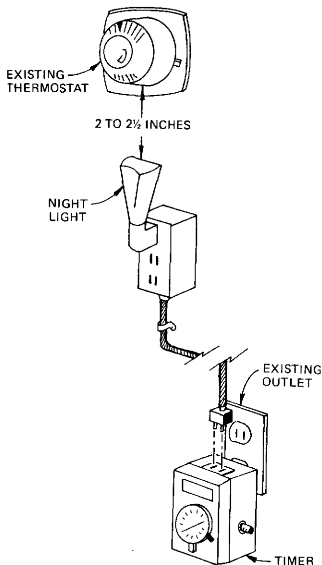
20. Do-it-Yourself Clock Thermostat. This is an inexpensive way to automatically set back your thermostat at night. Adjust the height of the night light until you get the right amount of setback.
