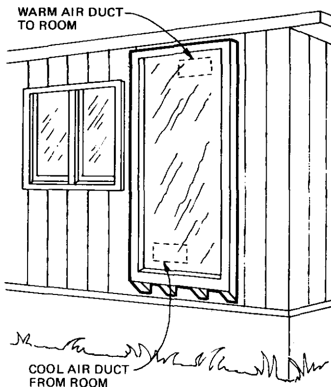
31. Thermosiphon Air Panel. A TAP can be made easily and cheaply and it will automatically supply heated air to the adjacent room during sunny days.
