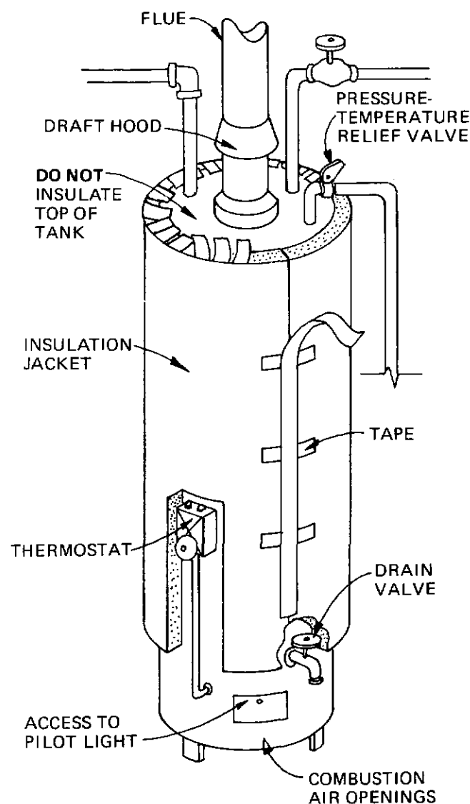
26. Gas Water Heater. Here are the points that should not be covered. Particularly important are the combustion air inlets, the draft hood, and the flue.
