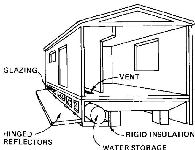
33. Underskirt Solar System. This is cheaper than a greenhouse but does not provide as much heat or additional living space.
