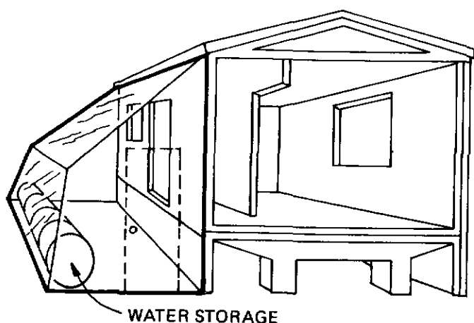
32. Greenhouse / Sunspace. These are relatively easy to build at reasonable cost, provide high solar gain and add living space.
