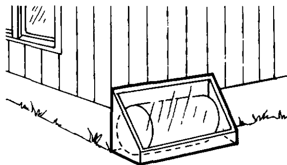
34. Solar Water Pre-Heater. This is an easy, low-cost project which can greatly increase the typical 65°F cold water supply temperature to 120°F plus.
