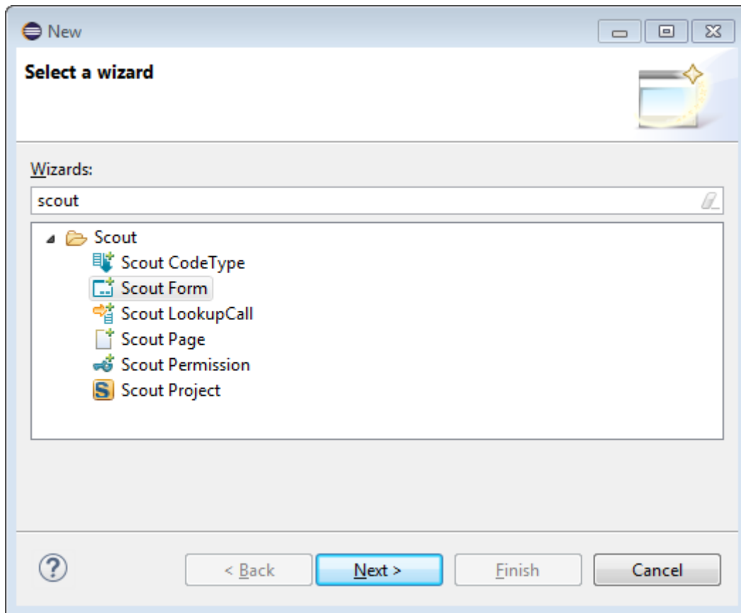
Figure 14. Selecting Scout Wizards in the Eclipse wizard dialog
