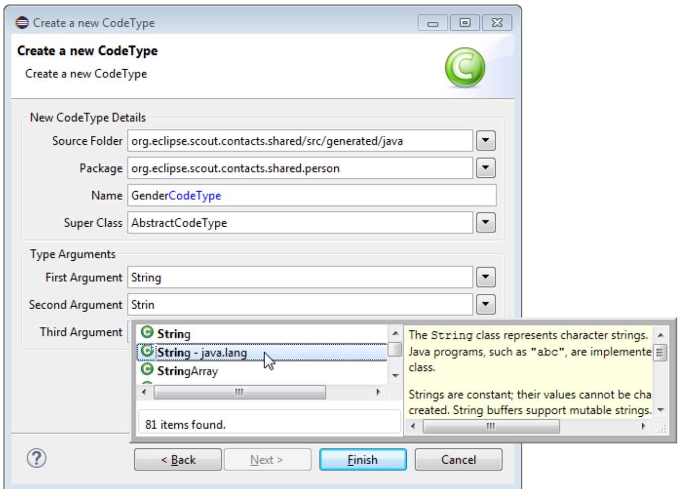
Figure 46. Create the gender code using the Scout new code wizard.
