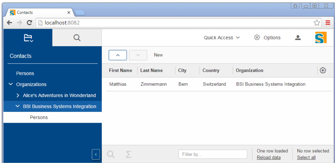
Figure 56. The linked person page only shows person related to the parent organization page.
