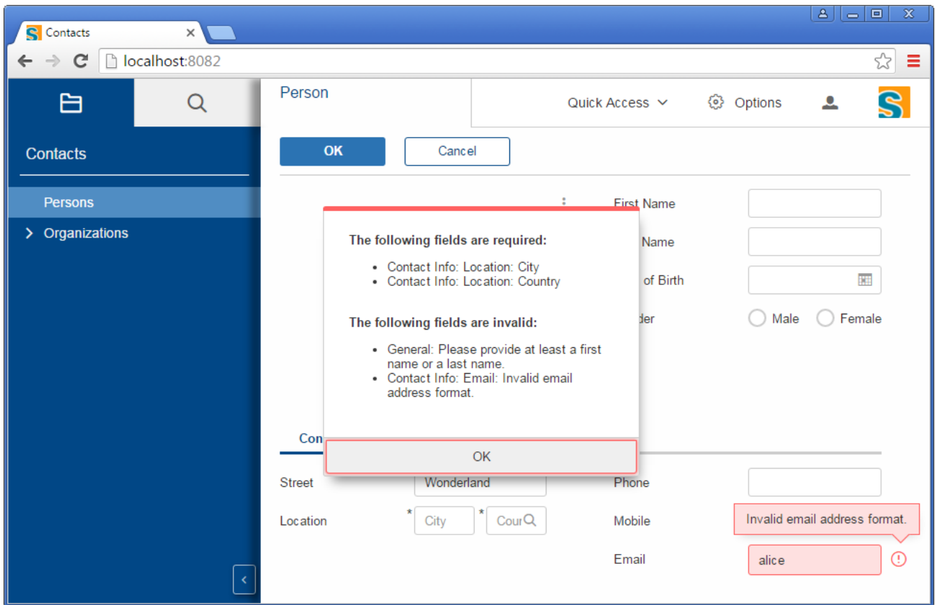
Figure 48. The form field validation implemented for the person form.
