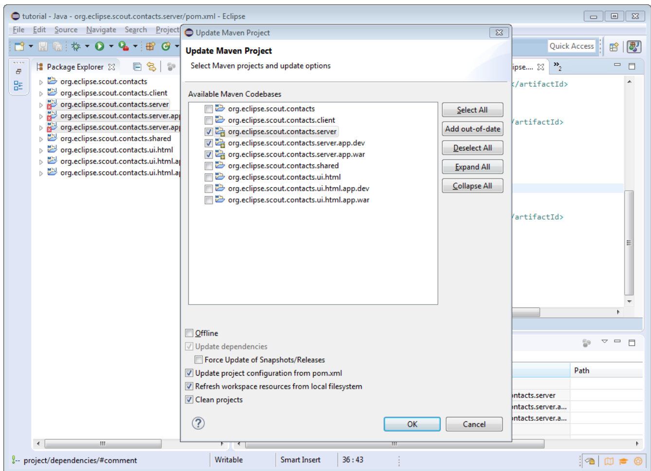
Figure 38. Update the Maven server modules for the "Contacts" application.
