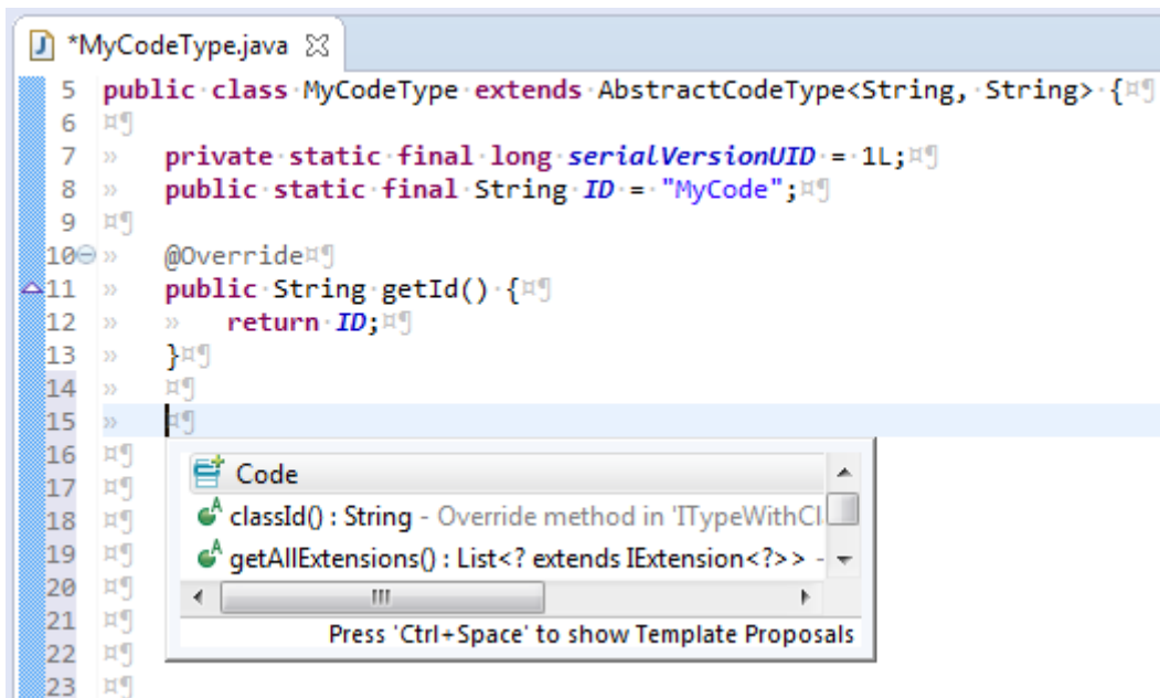
Figure 20. Proposals to create new codes in a CodeType
