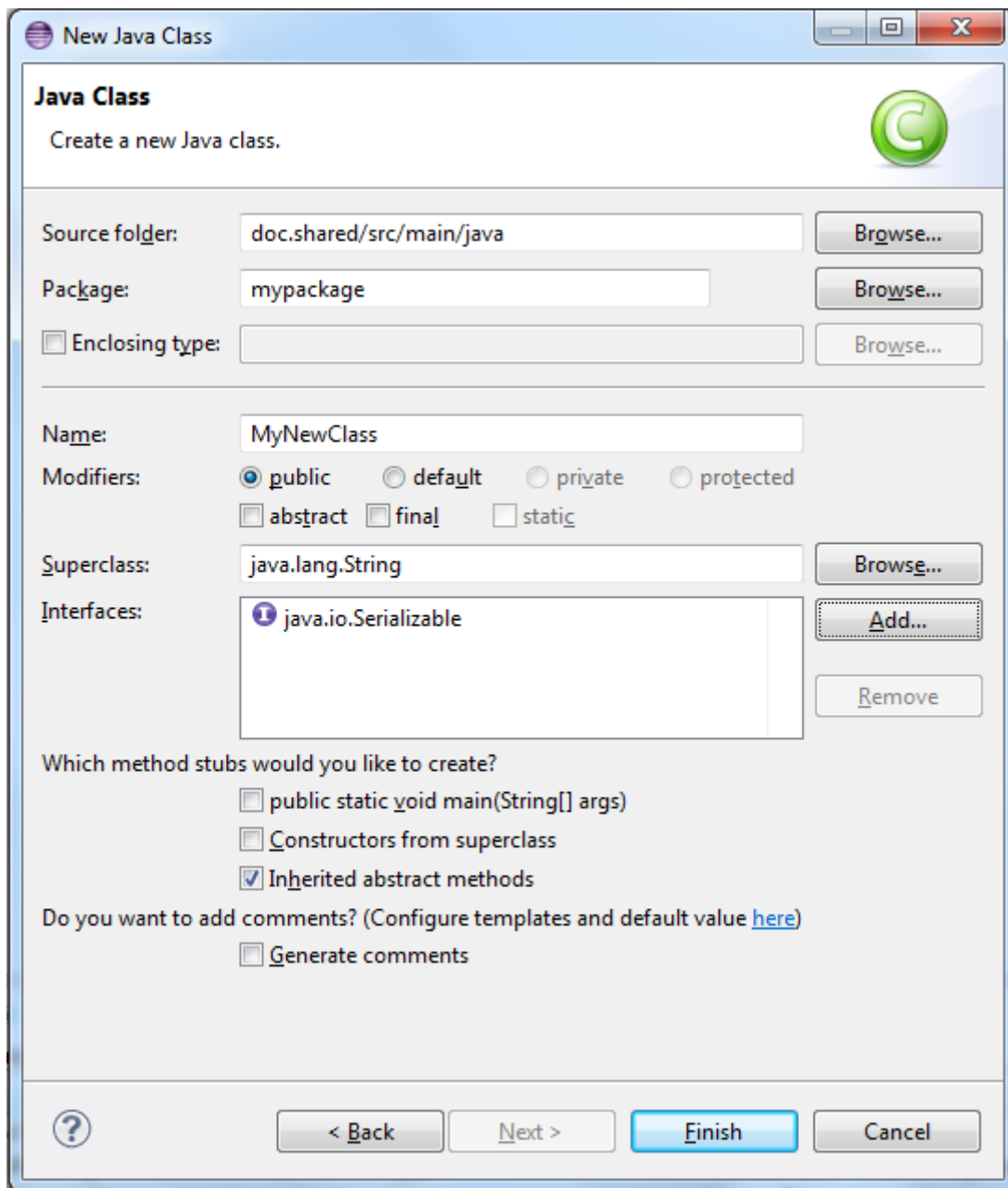
Figure 13. "New Java Class" Wizard
