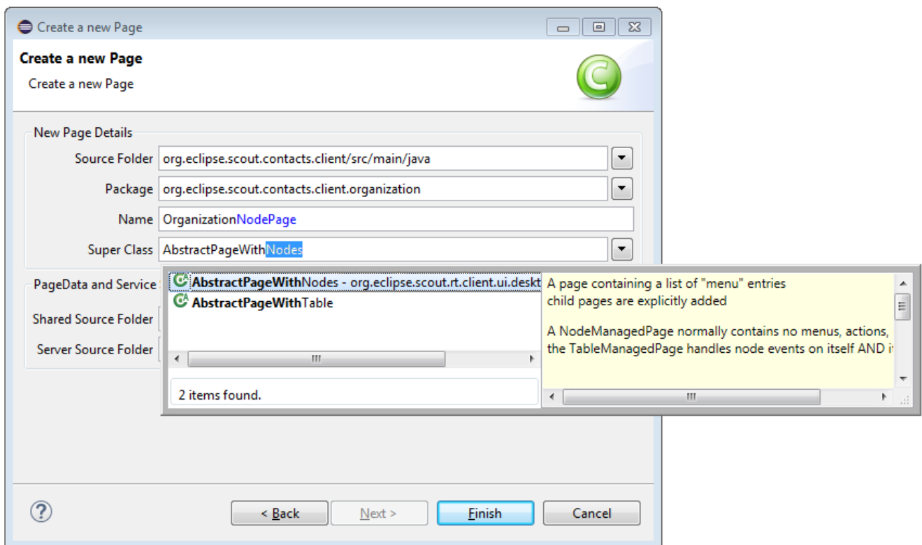
Figure 55. Creating the organization node page.
