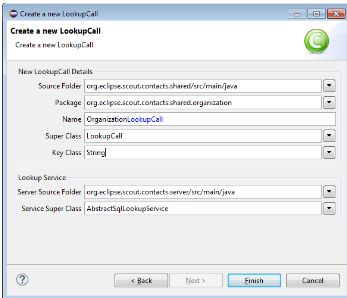
Figure 53. Using the Scout lookup call wizard for creating class OrganizationLookupCall .
