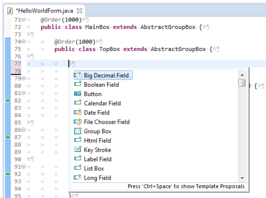
Figure 18. Proposals to create new form fields in a GroupBox
