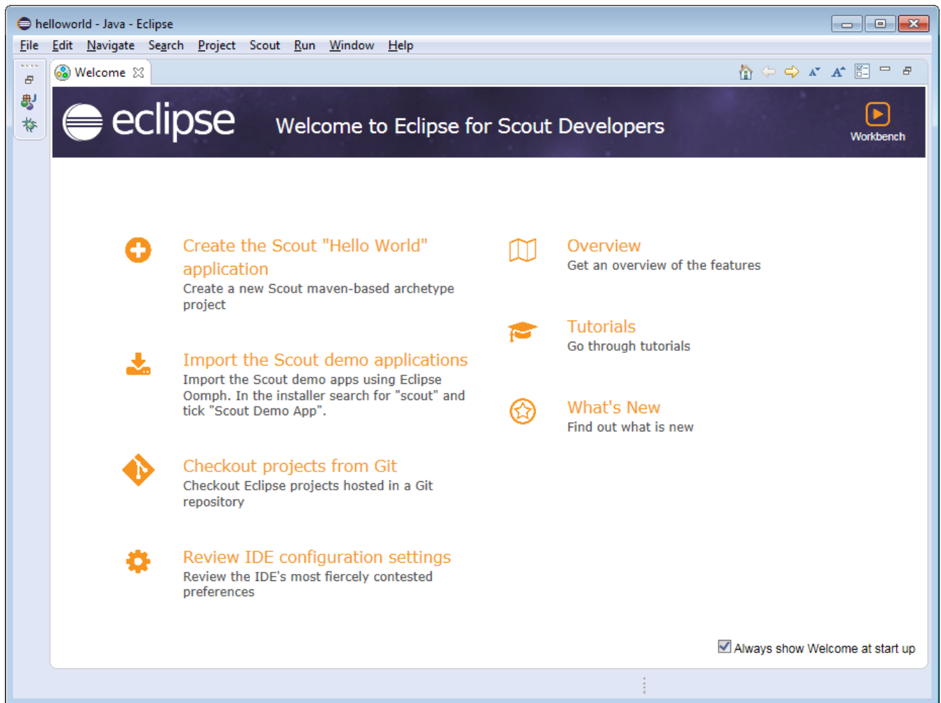
Figure 62. Eclipse Scout welcome screen.
