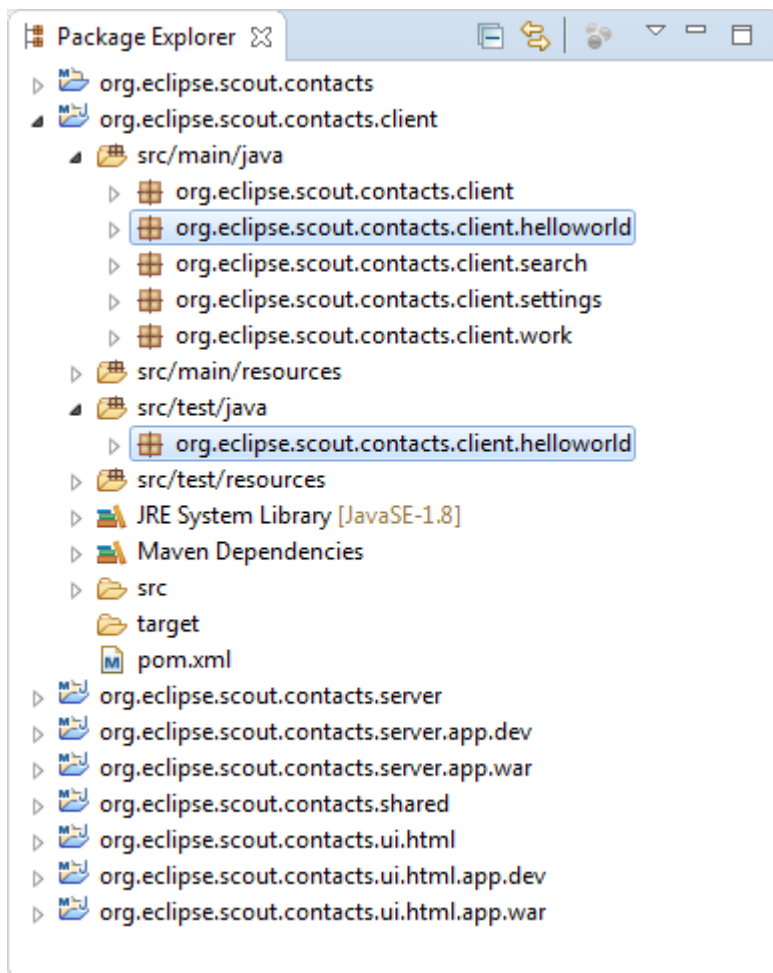
Figure 27. The package explorer with the initial Maven modules created for the "Contacts" application.
