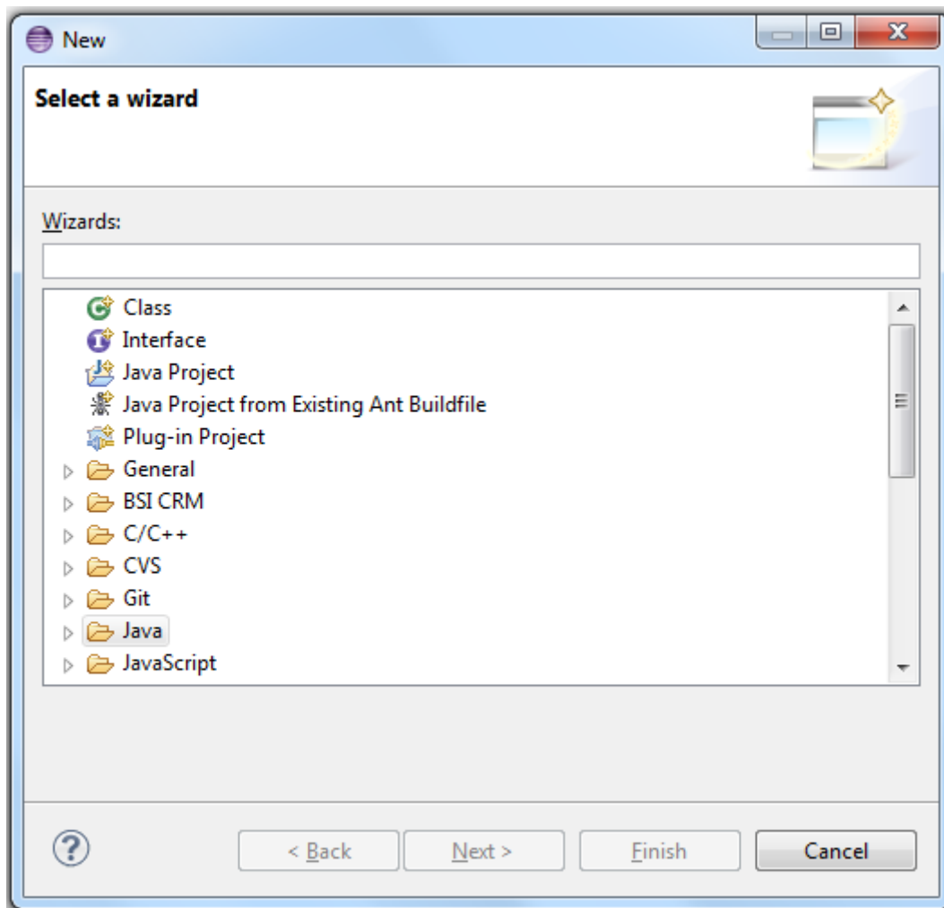
Figure 12. "New" Wizard
