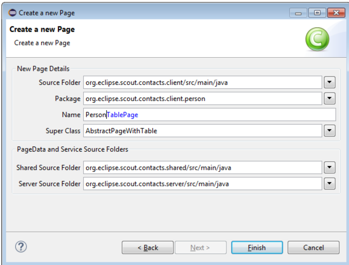
Figure 34. Add the person page to the "Contacts" application.
