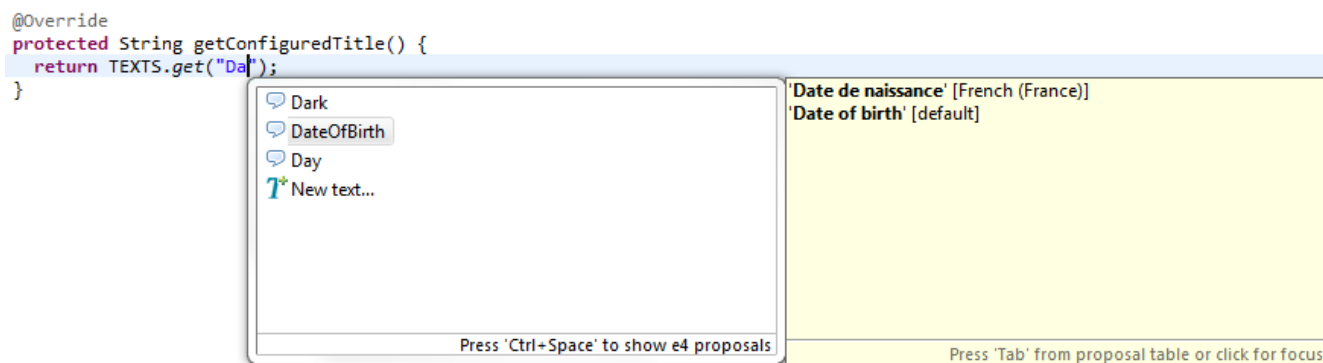
Figure 21. Proposals corresponding to NLS Support.
