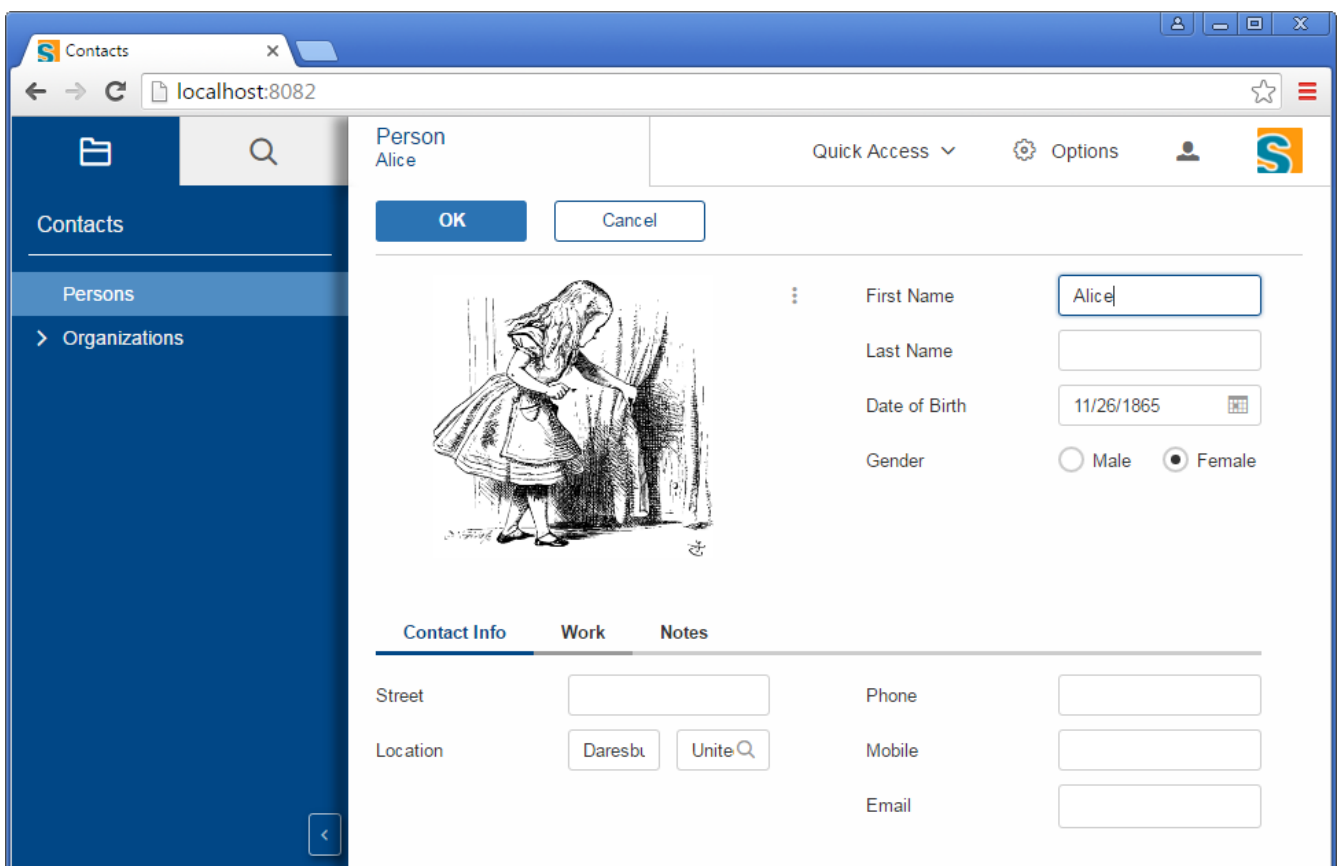
Figure 47. The "Contacts" application with the person form at the end of tutorial step 4.
