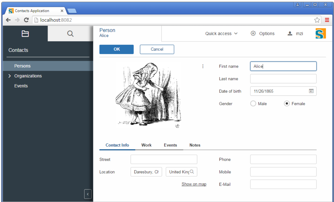
Figure 25. The "Contacts" application with a person opened in a form.
