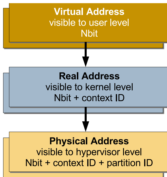
Figure 3. Virtual-to-Physical Memory Mapping
