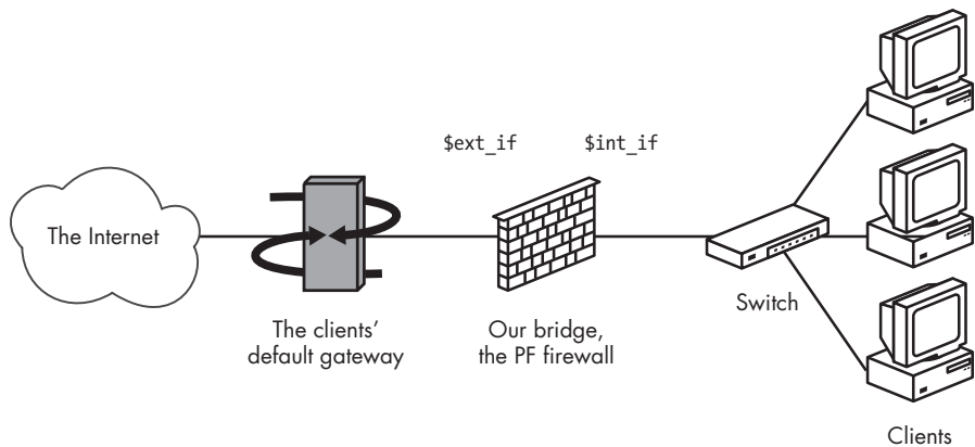
Figure 5-3: A network with a bridge firewall
