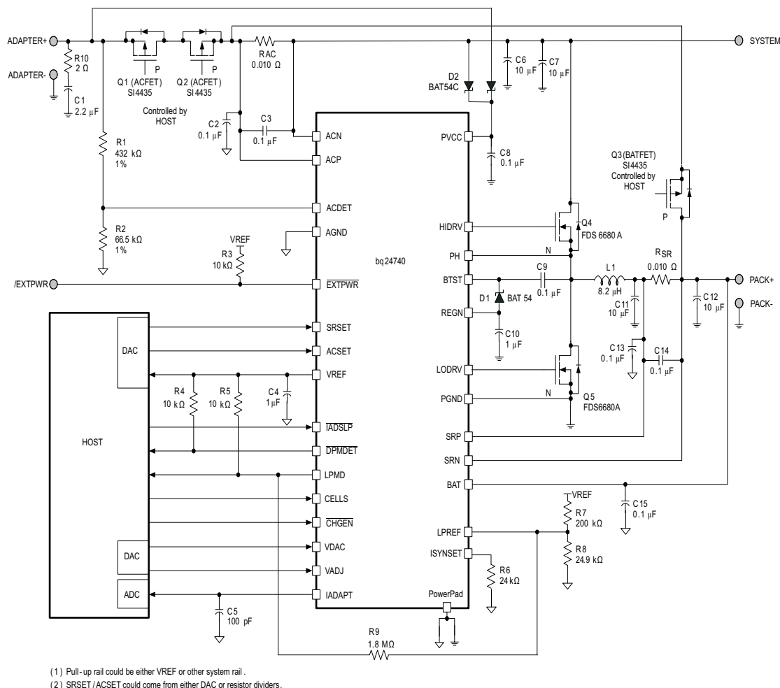
Figure 3. Typical System Schematic: Sensing Battery Discharge Current, When Adapter Removed. (Set IADSLP at logic high)
