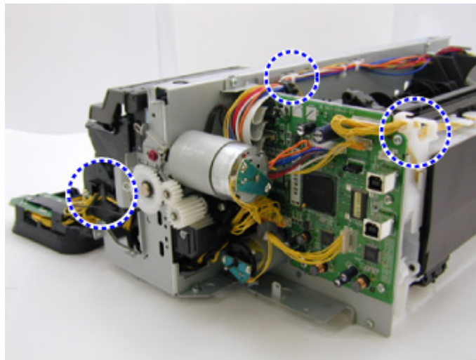
(I) Logic board ass'y and operation panel unit wiring
