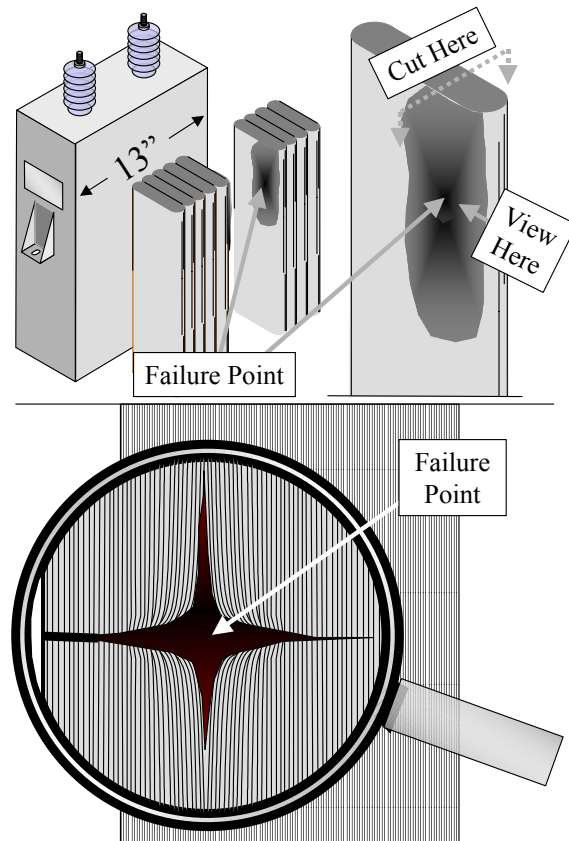
Figure 3. FOIL ELECTRODE CAPACITOR DISSECTION
