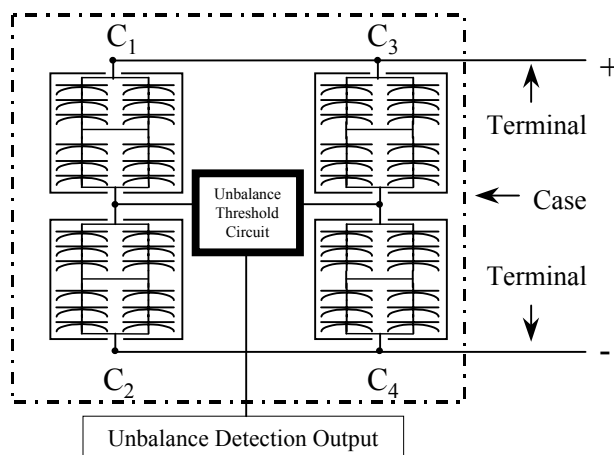
Figure 6. HIGH VOLTAGE CAPACITOR WITH AN INTERNAL UNBALANCE DETECTION CIRCUIT
