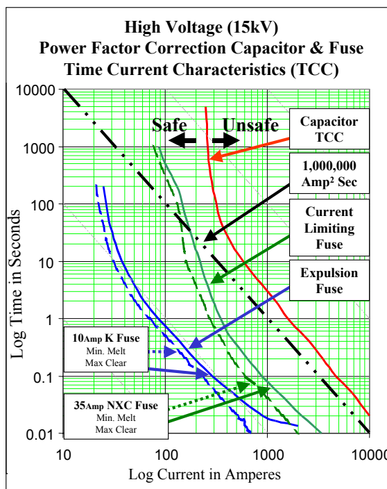
Figure 1. TCC CURVES
