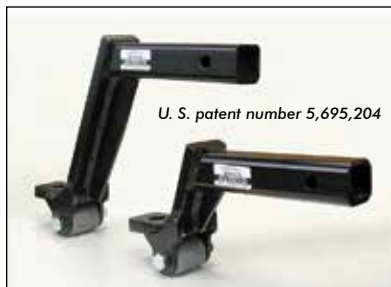
Shown: 10-inch and four-inch Roller Hitches. Also available in six- and eight-inch sizes.
