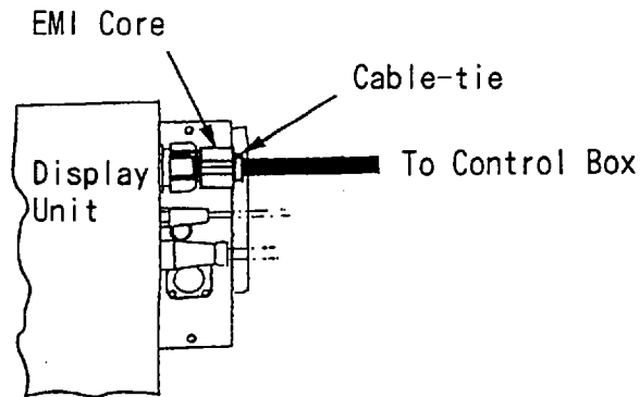
Display unit, right side view
