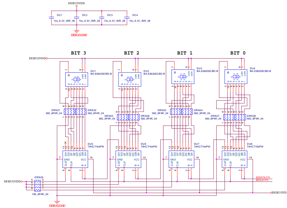
Near 74164 pin-14
