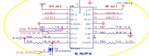
USB Charger components
