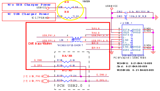
USB 3.0/PCH USB 2.0 Co-layout
