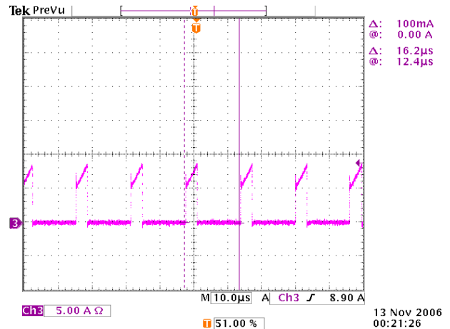
Ch3 is PFC stage Mosfet Drain current (zoom out)
