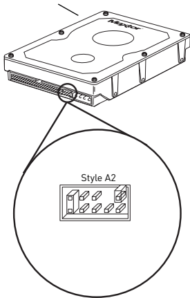
FIGURE 5 COMMON JUMPER BLOCKS
