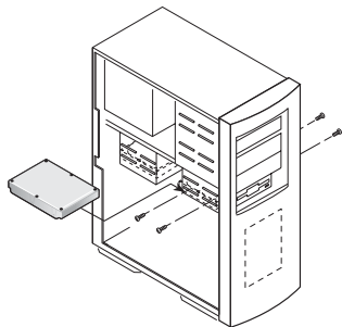
FIGURE 7 TYPICAL 3.5-INCH DEVICE BAY INSTALLATION
