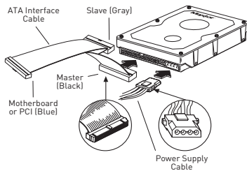
FIGURE 9 CONNECTING THE CABLES
