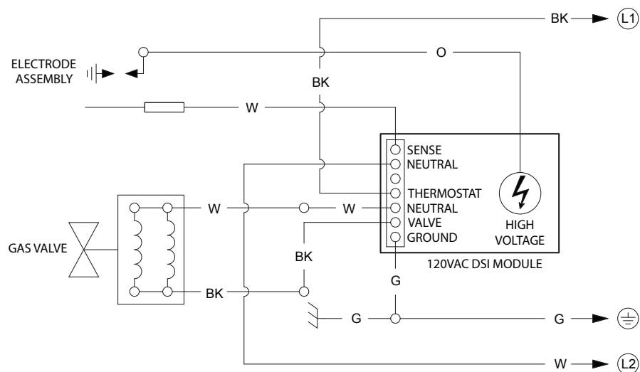
Figure 2.10 • NFS-2/PFS-2 (120V) • 120 V Schematic
