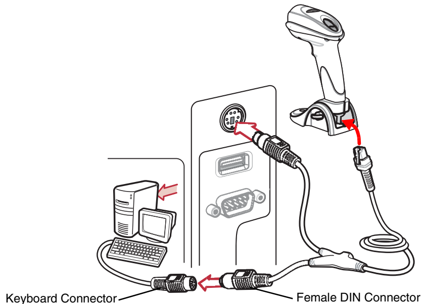
Figure 11-2 Keyboard Wedge Connection with Y-cable for Scanner with Base
