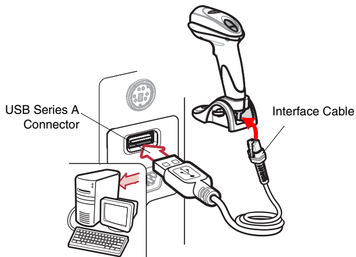
Figure 6-2 USB Connection for Scanner with Base
