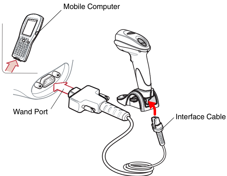
Figure 9-2 Wand Emulation Connection for Scanner with Base
