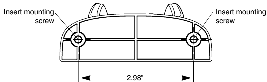
Figure 1-9 Wall Mounting Template
