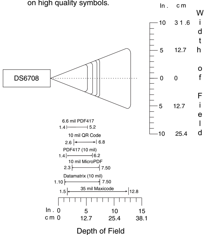
Figure 2-17 DS6708 Digital Scanner Decode Zone for 2D Bar Codes
