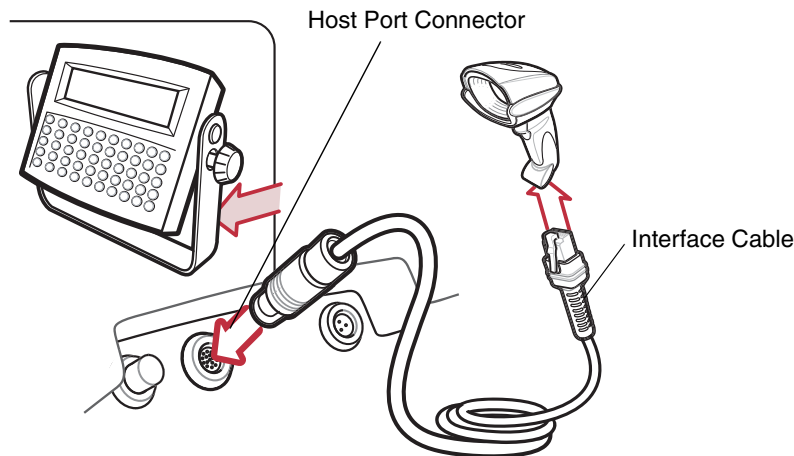
Figure 10-1 Scanner Emulation Connection
