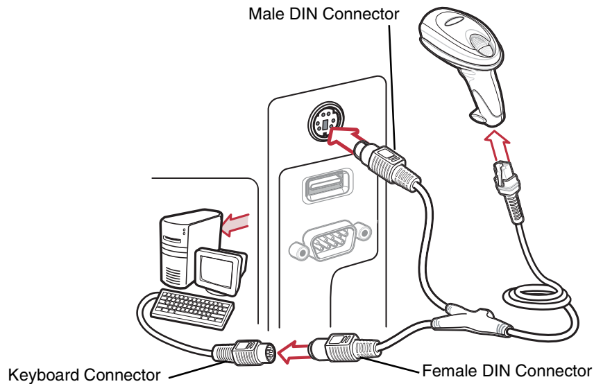
Figure 11-1 Keyboard Wedge Connection with Y-cable
