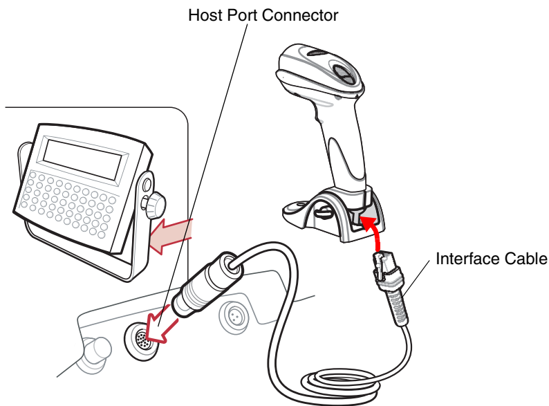
Figure 10-2 Scanner Emulation Connection for Scanner with Base
