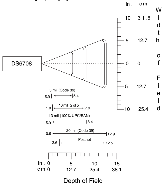
Figure 2-16 DS6708 Digital Scanner Decode Zone for 1D Bar Codes
