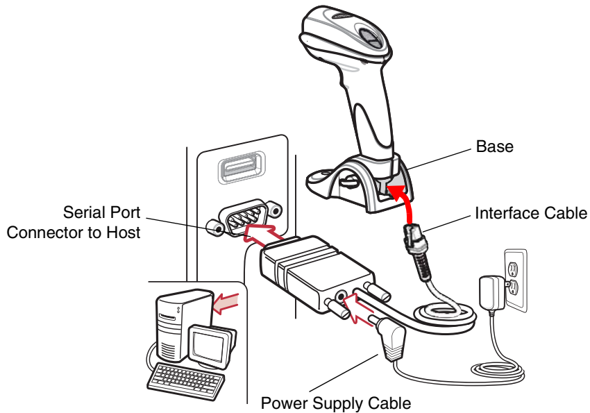
Figure 7-1 RS-232 Direct Connection
