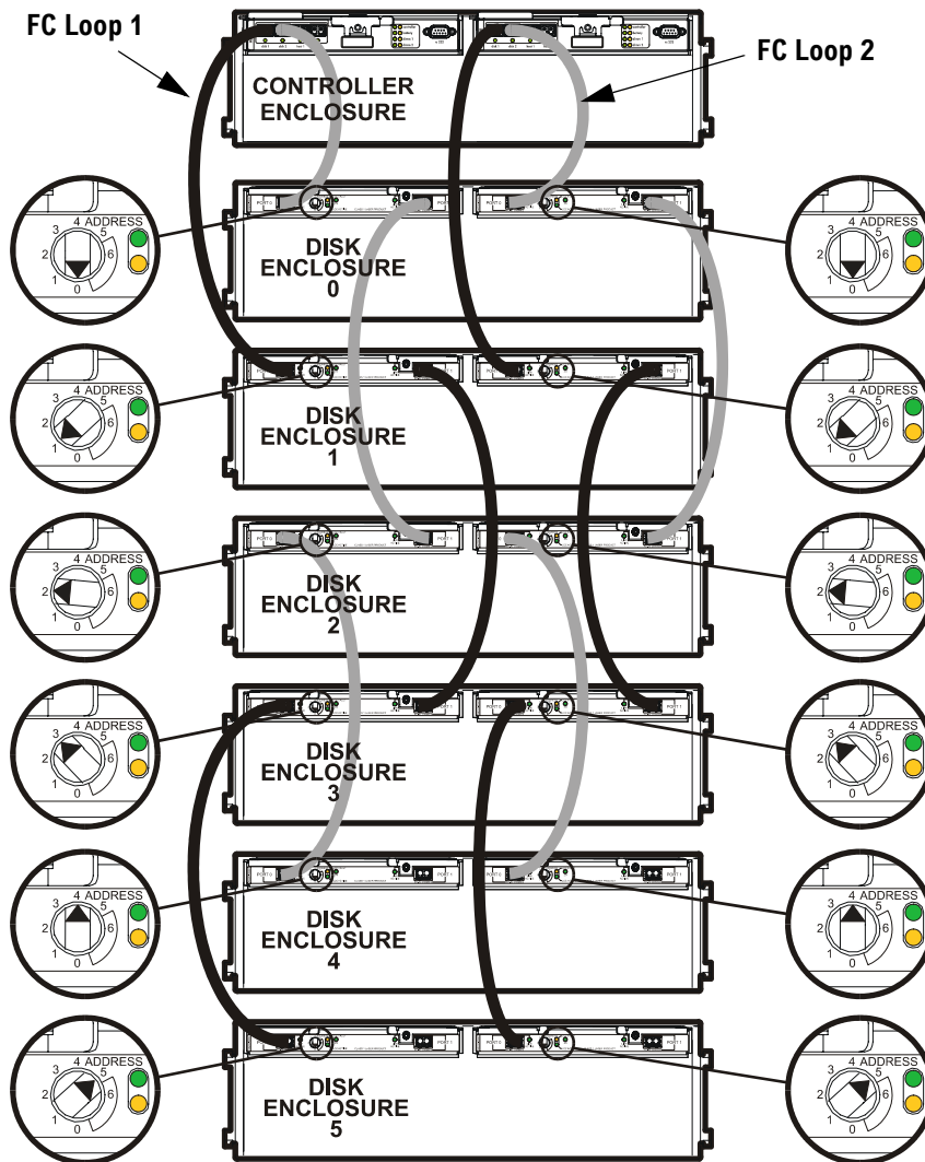
Figure 10 VA 7410 Back-End Fiber Optic Cabling & Addressing (6 Disk Enclosures)
