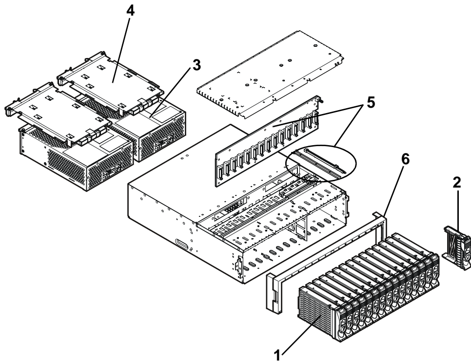
Figure 33 Disk Enclosure FRUs
