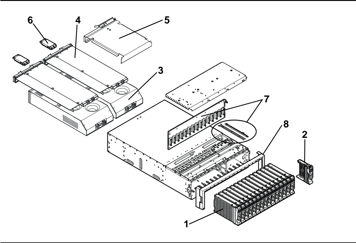
Figure 32 Controller Enclosure FRUs
