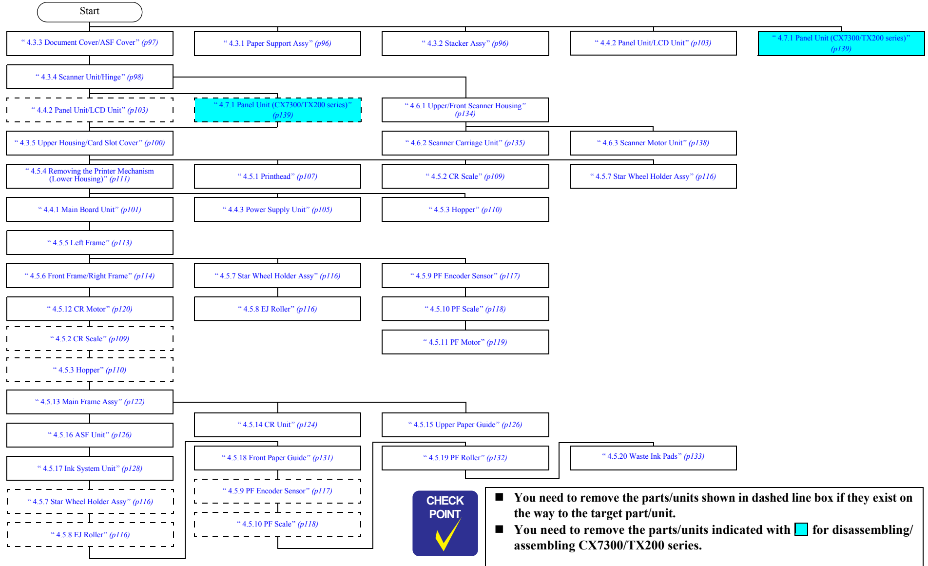
Figure 4-1. Disassembling Flowchart
