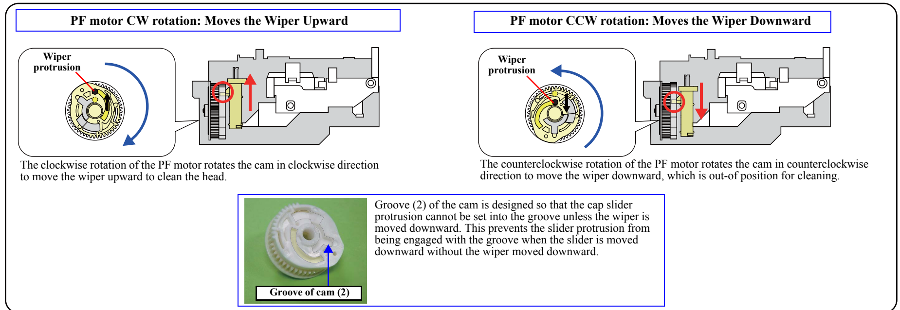
Figure 2-17. Wiping Mechanism
