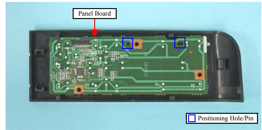
Figure 4-23. Removing the Panel Board
