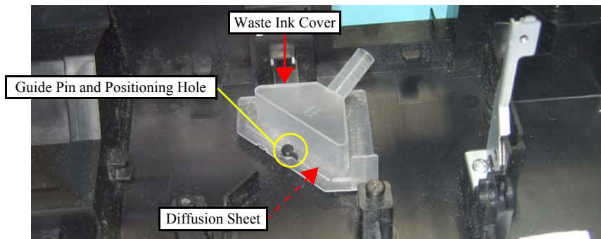
Figure 4-102. Removing the Waste Ink Cover and Diffusion Sheet
