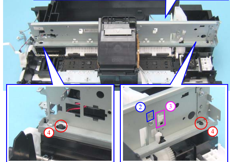
Figure 4-74. Main Frame Assy
