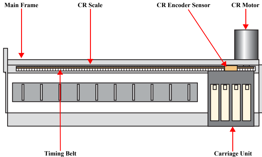
Figure 2-7. Carriage Mechanism
