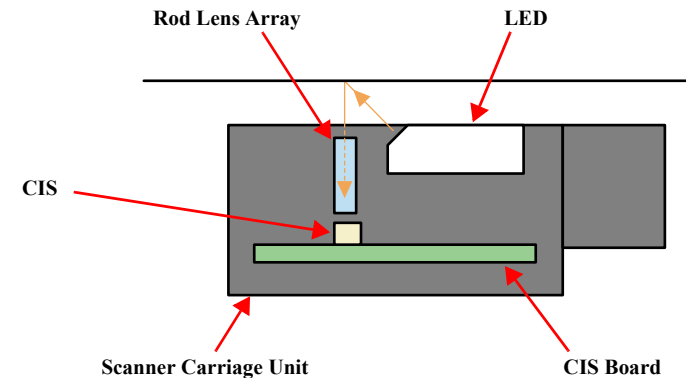
Figure 2-21. Scanning image
