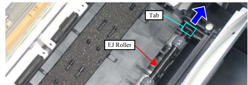
Figure 4-61. Removing the EJ Roller (2)
