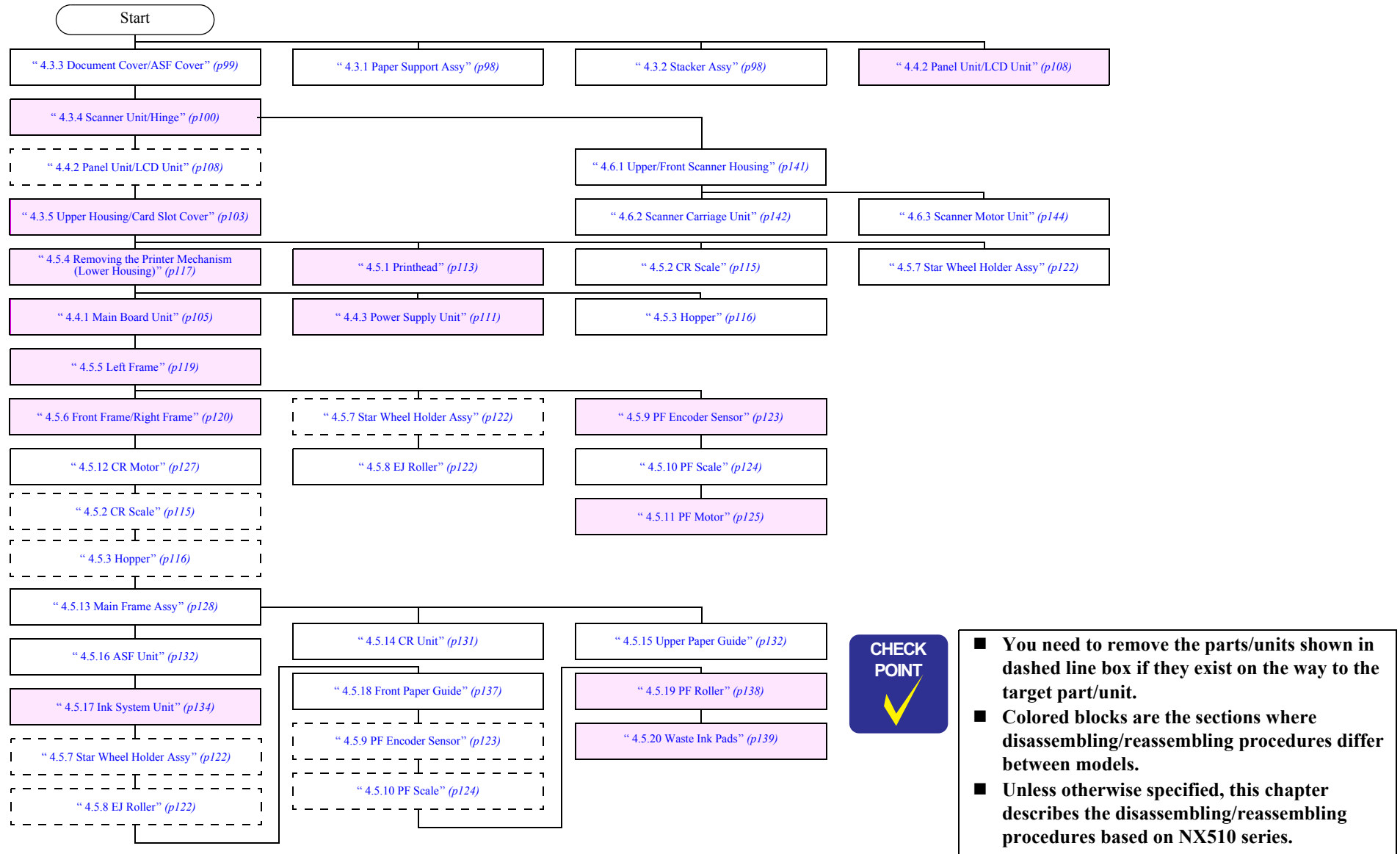
Figure 4-1. Disassembling Flowchart
