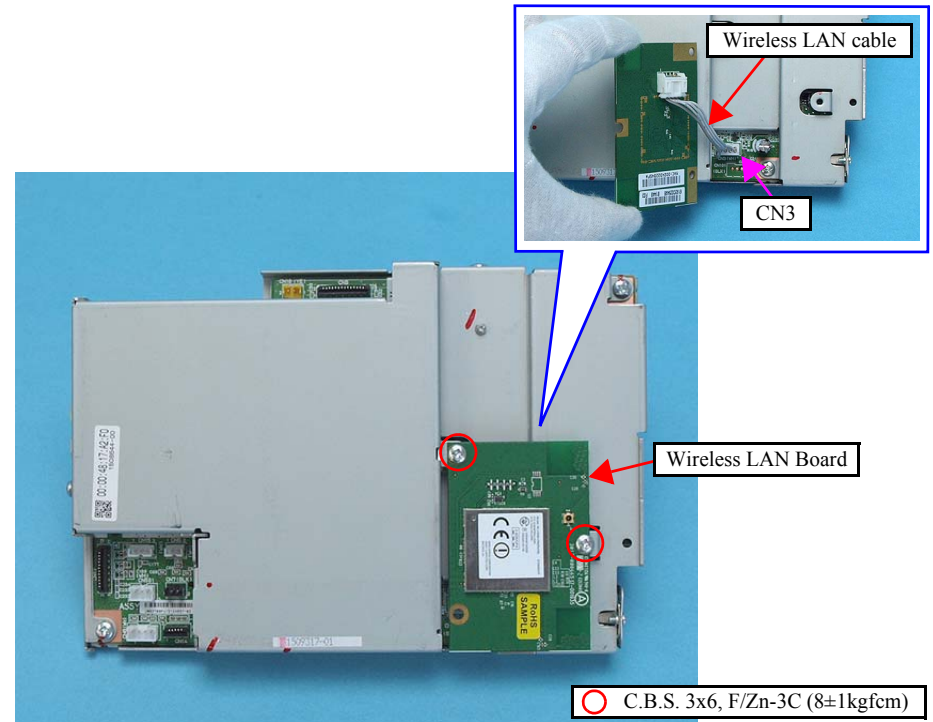
Figure 4-21. Removing the Wireless LAN Board
