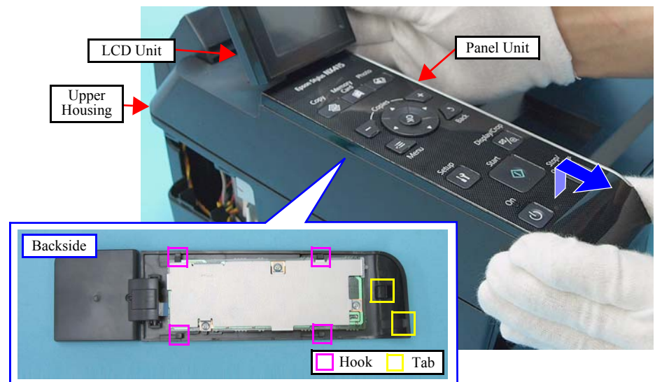
Figure 4-132. Removing the Panel Unit and LCD Unit (1)
