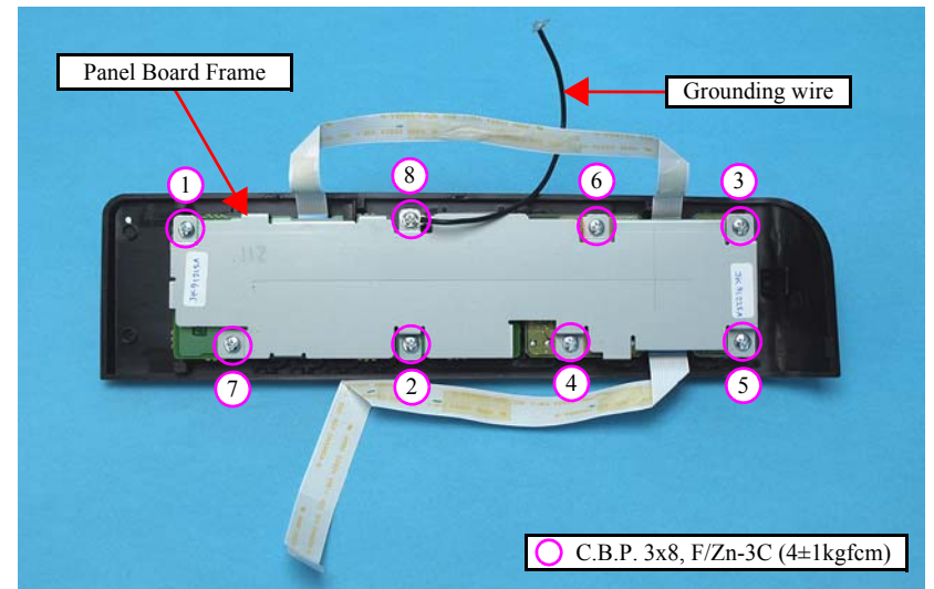
Figure 4-149. Removing the Panel Board Frame
