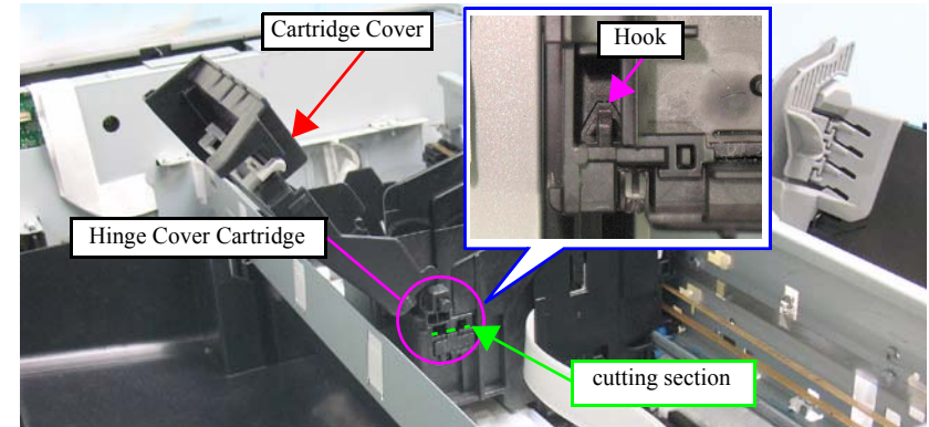
Figure 4-37. Removing the Cartridge Cover
