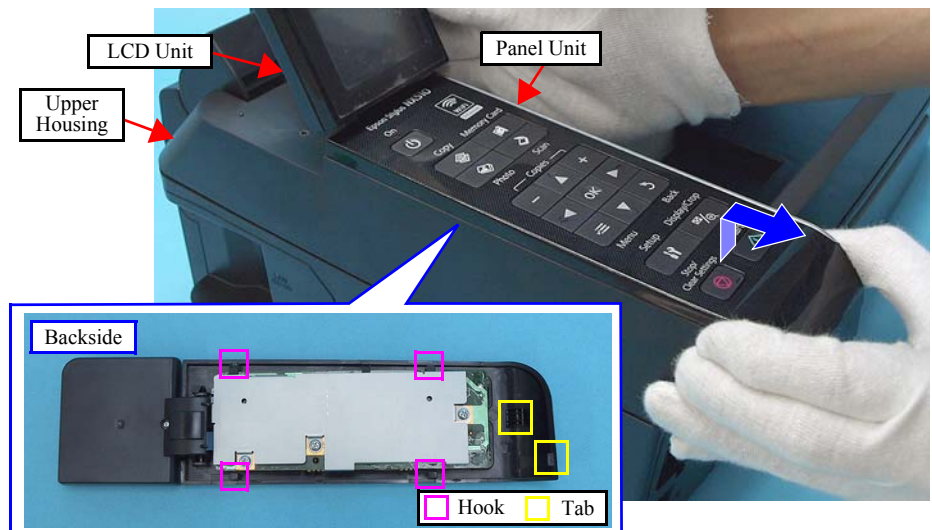
Figure 4-25. Removing the Panel Unit and LCD Unit (1)
