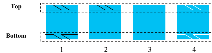
Figure 5-8. PF (standard print area) Adjustment Printout Pattern
