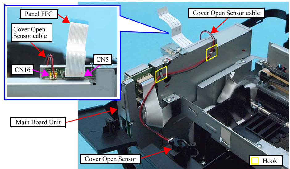
Figure 4-47. Removing the Printer Mechanism (1)
