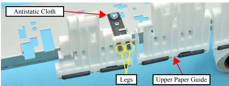
Figure 4-86. Installing the Upper Paper Guide
