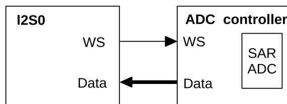
Figure 66: ADC Interface of I2S0
