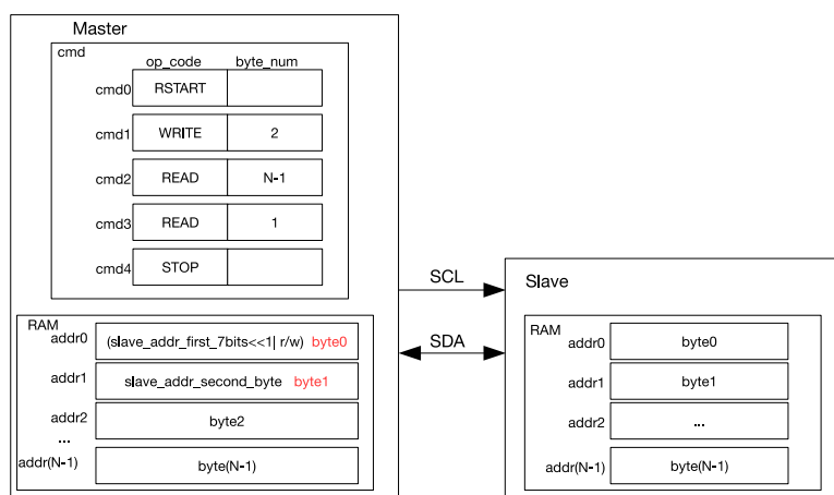
Figure 47: I2C Master Reads from Slave with 10-bit Address
