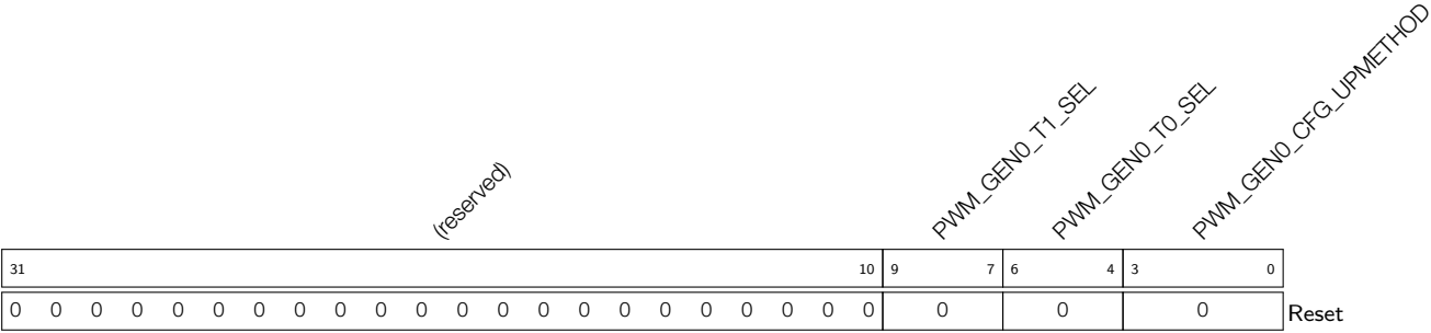
Register 15.19: PWM_GEN0_CFG0_REG (0x0048)
