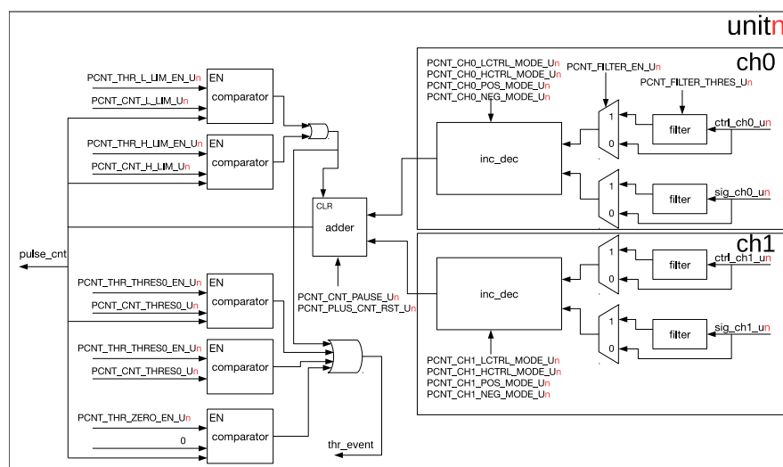
Figure 109: PULSE_CNT Architecture
