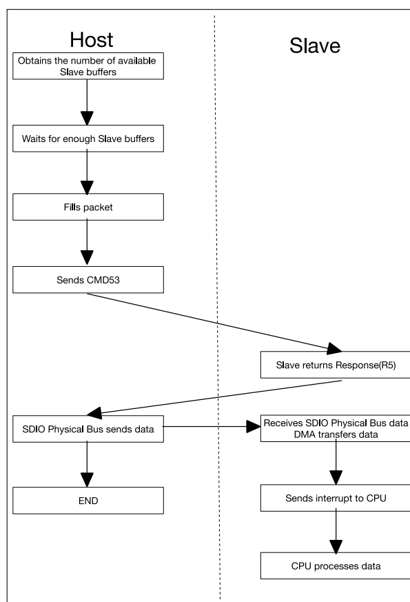
Figure 25: Packet Receiving Procedure (Initiated by Host)
