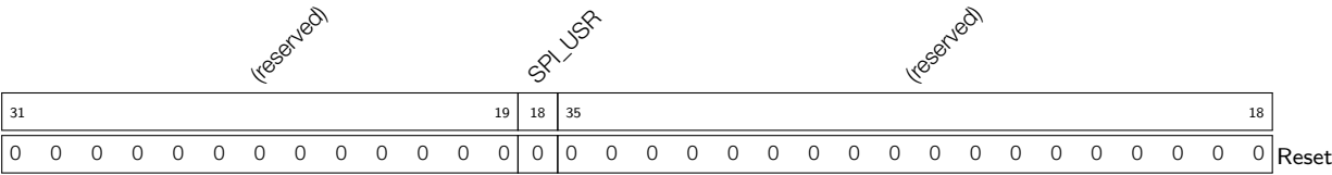
Register 7.1: SPI_CMD_REG (0x0)
