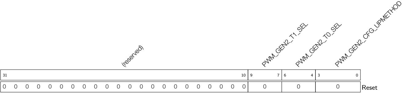
Register 15.47: PWM_GEN2_CFG0_REG (0x00b8)
