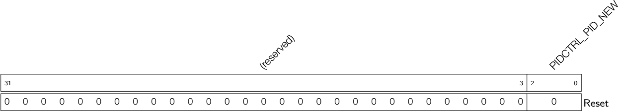
Register 26.13: PIDCTRL_PID_NEW_REG (0x048)
