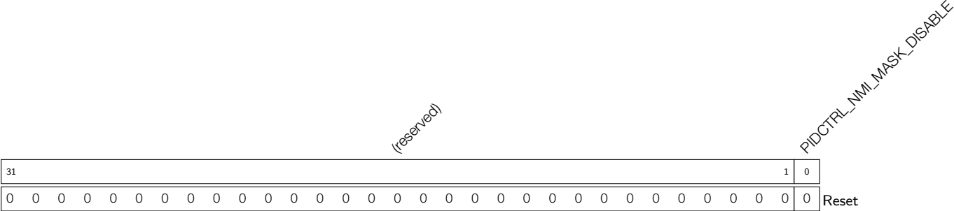
Register 26.16: PIDCTRL_NMI_MASK_DISABLE_REG (0x058)
