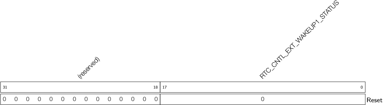
Register 29.36: RTC_CNTL_EXT_WAKEUP1_STATUS_REG (0x0034)
