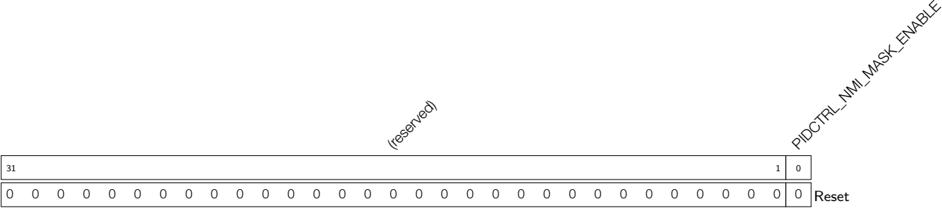
Register 26.15: PIDCTRL_NMI_MASK_ENABLE_REG (0x054)
