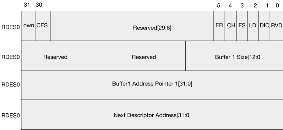
Figure 36: The Structure of a Linked List
