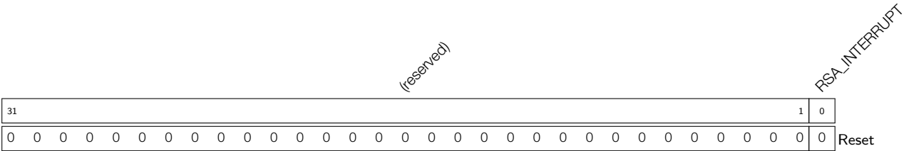
Register 22.6: RSA_INTERRUPT_REG (0x814)
