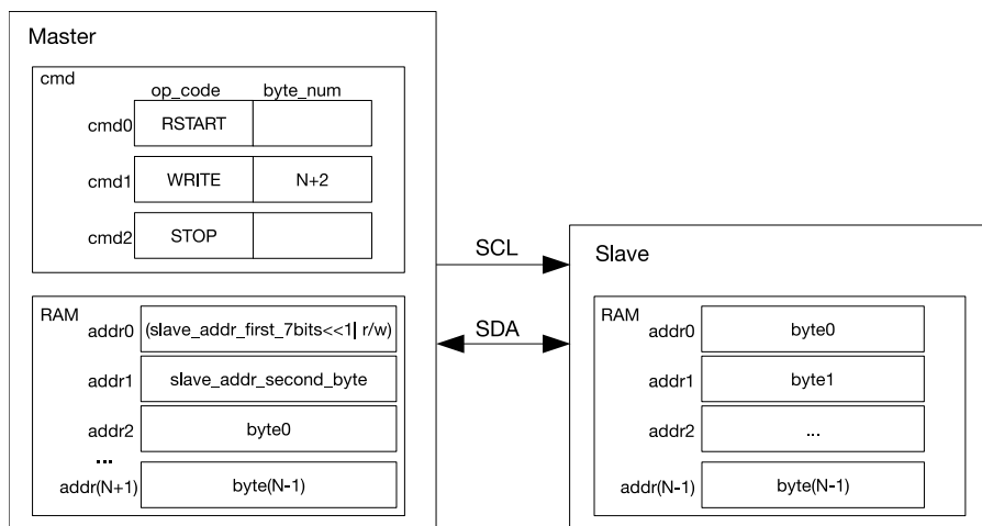
Figure 43: I2C Master Writes to Slave with 10-bit Address
