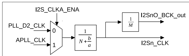
Figure 51: I2S Clock
