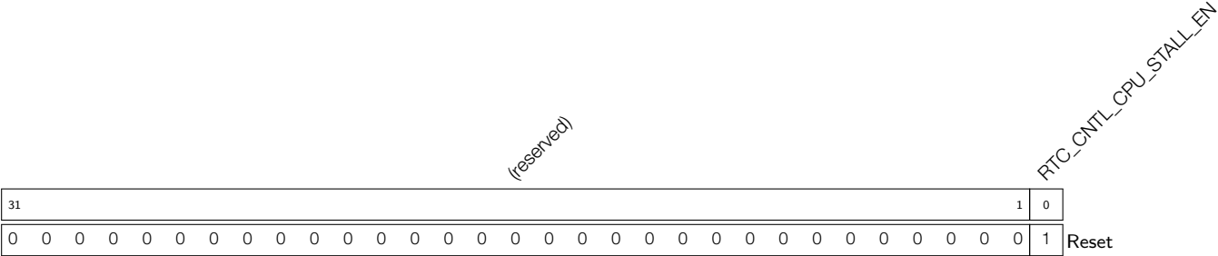
Register 29.8: RTC_CNTL_TIMER1_REG (0x0007)
