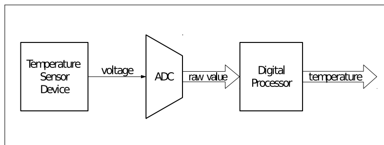
Figure 126: Temperature Sensor
