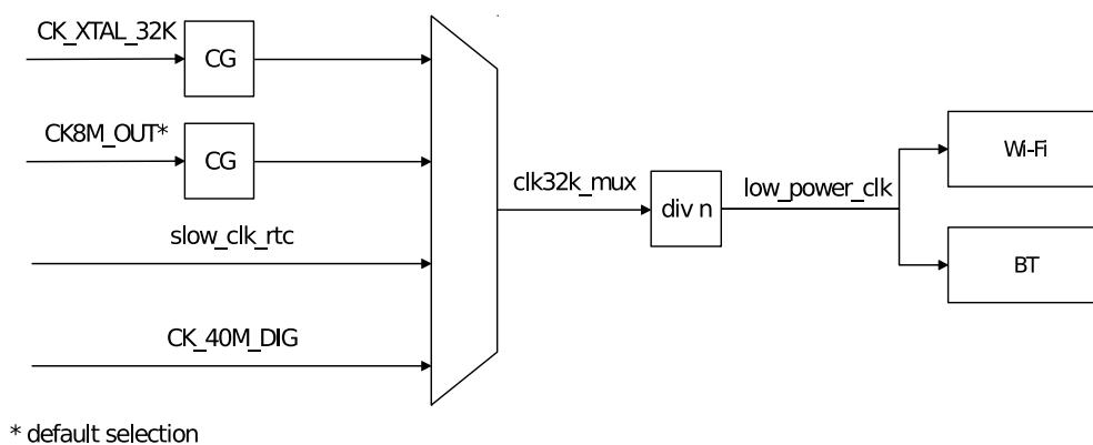
Figure 159: Digital Low-Power Clocks
