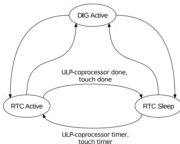
Figure 160: RTC States
