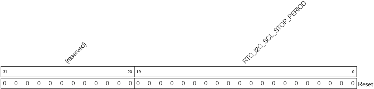
Register 28.19: RTC_I2C_SCL_STOP_PERIOD_REG (0x044)
