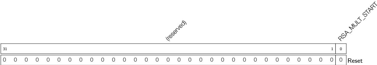
Register 22.5: RSA_MULT_START_REG (0x810)
