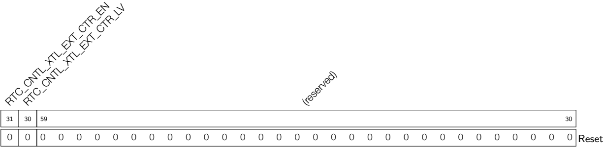
Register 29.19: RTC_CNTL_EXT_XTL_CONF_REG (0x0017)
