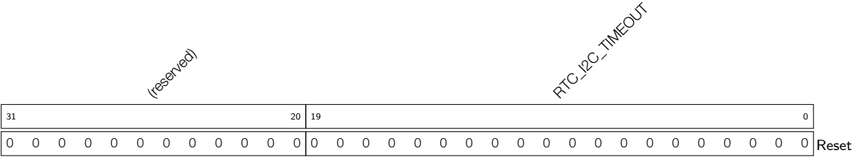
Register 28.11: RTC_I2C_TIMEOUT_REG (0x00c)
