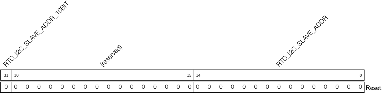
Register 28.12: RTC_I2C_SLAVE_ADDR_REG (0x010)
