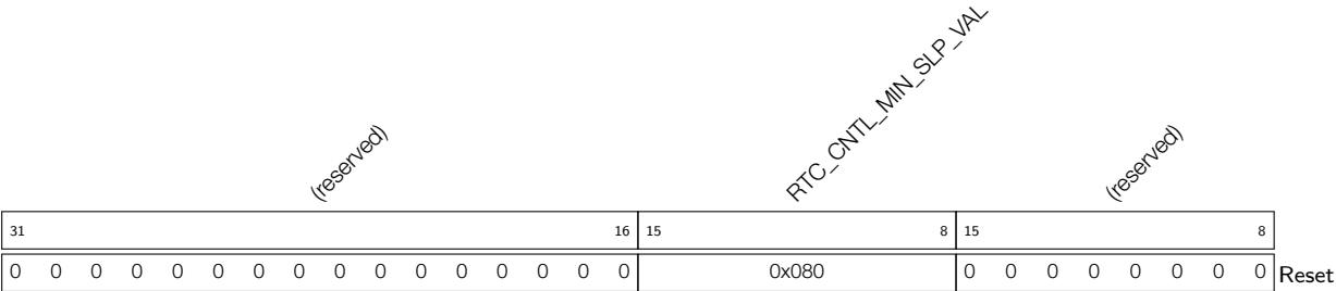
Register 29.10: RTC_CNTL_TIMER5_REG (0x000b)
