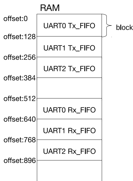
Figure 70: UART shared RAM
