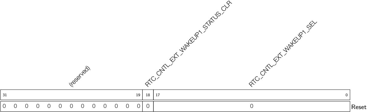
Register 29.35: RTC_CNTL_EXT_WAKEUP1_REG (0x0033)
