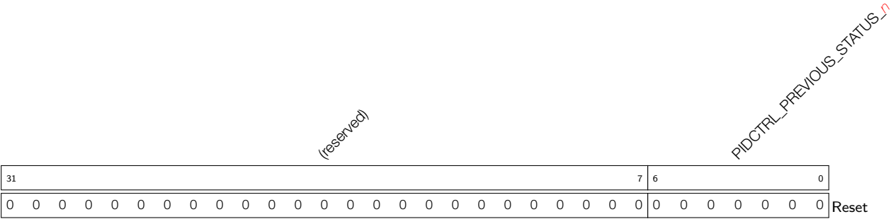
Register 26.12: PIDCTRL_FROM_n_REG (n: 1-7) (0x28+0x4*n)
