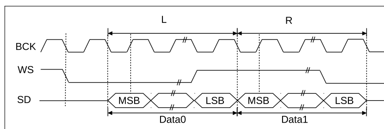
Figure 52: Philips Standard
