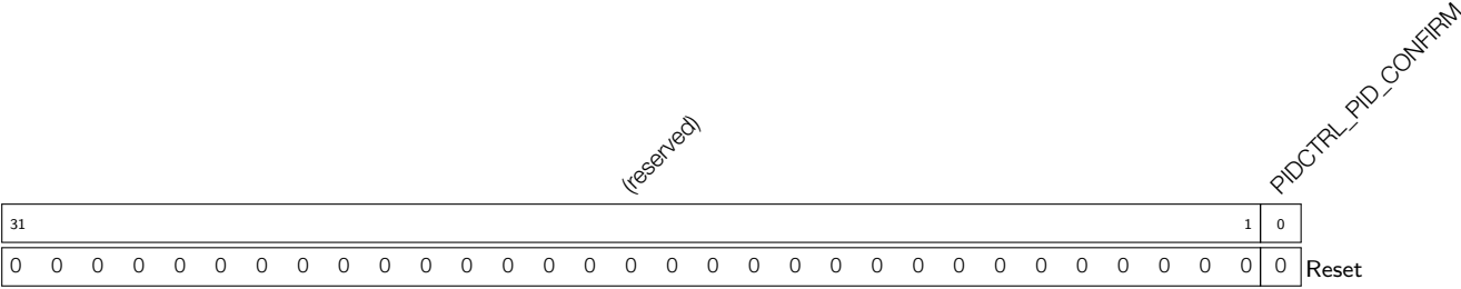
Register 26.14: PIDCTRL_PID_CONFIRM_REG (0x04C)
