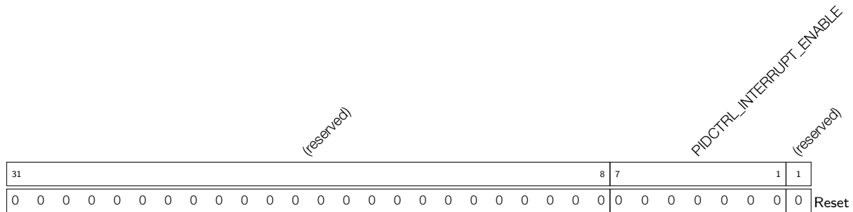
Register 26.1: PIDCTRL_INTERRUPT_ENABLE_REG (0x000)
