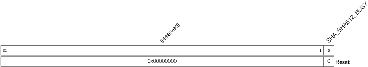
Register 21.17: SHA_SHA512_BUSY_REG (0x0BC)
