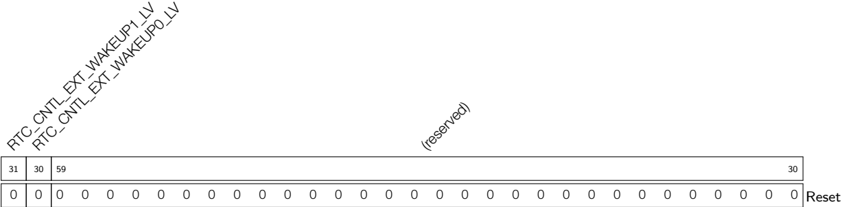
Register 29.20: RTC_CNTL_EXT_WAKEUP_CONF_REG (0x0018)
