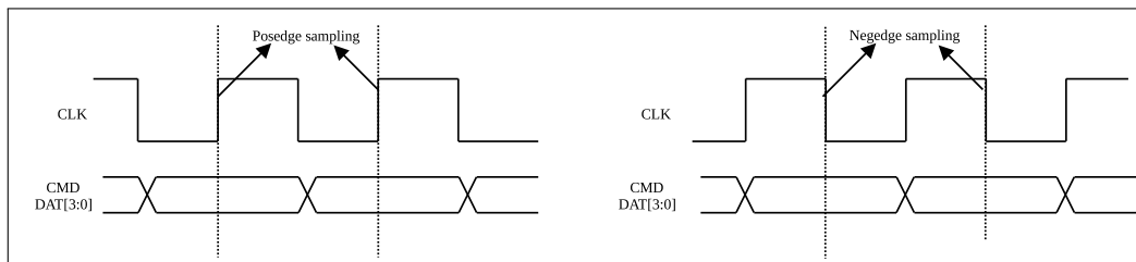
Figure 27: Sampling Timing Diagram
