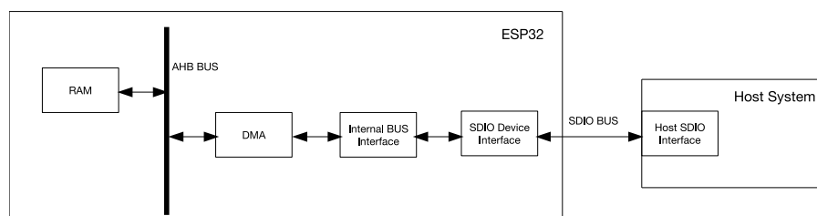
Figure 19: SDIO Slave Block Diagram
