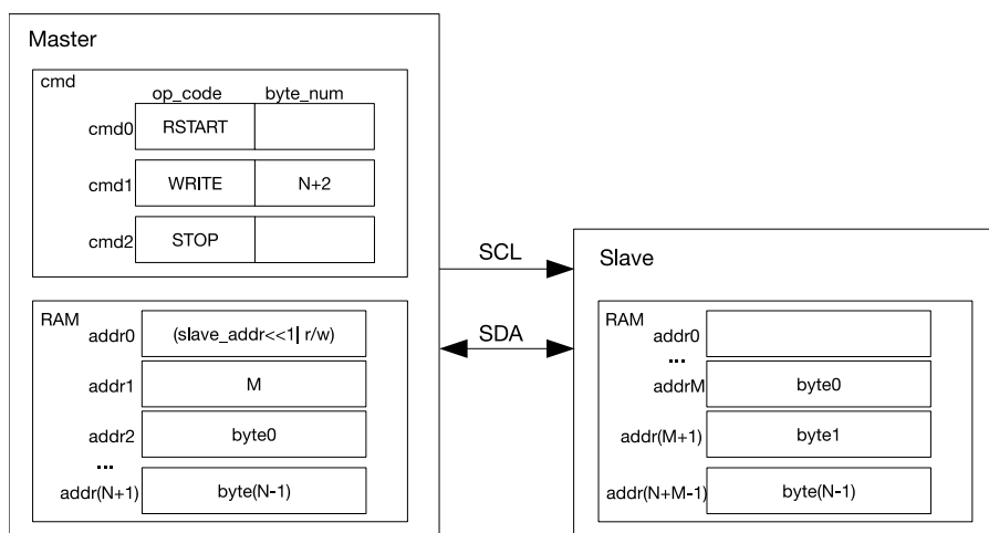
Figure 44: I2C Master Writes to addrM in RAM of Slave with 7-bit Address
