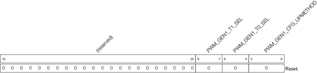
Register 15.33: PWM_GEN1_CFG0_REG (0x0080)
