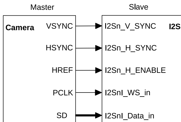
Figure 65: Camera Slave Receiving Mode
