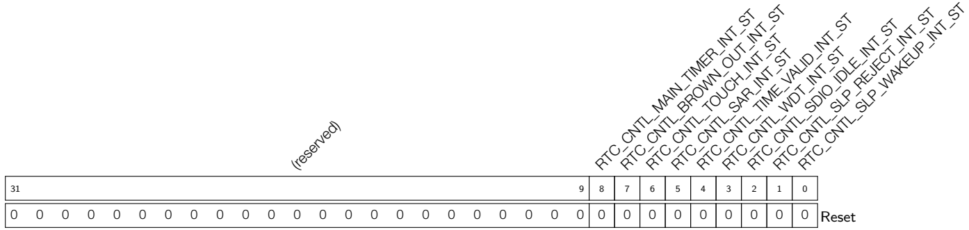
Register 29.16: RTC_CNTL_INT_ST_REG (0x0011)
