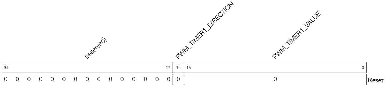
Register 15.9: PWM_TIMER1_STATUS_REG (0x0020)
