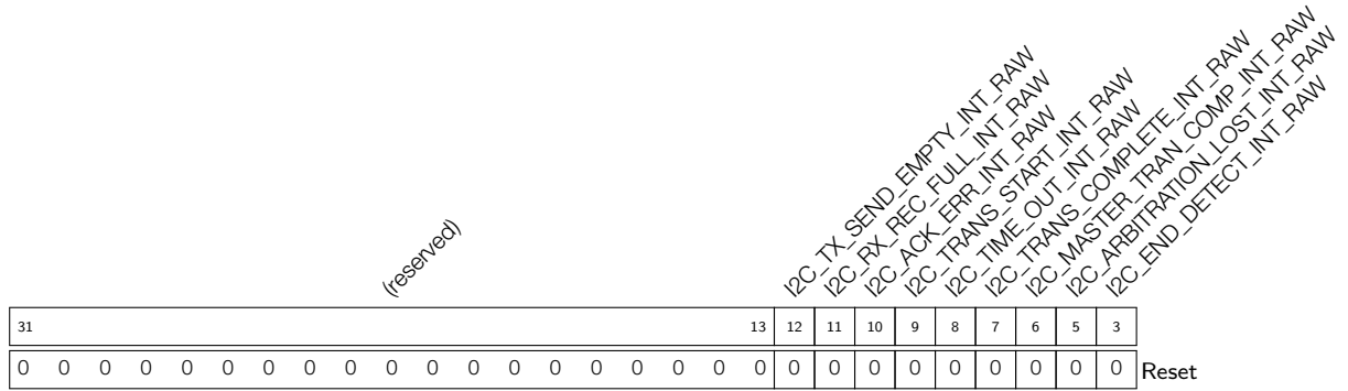
Register 10.8: I2C_INT_RAW_REG (0x0020)
