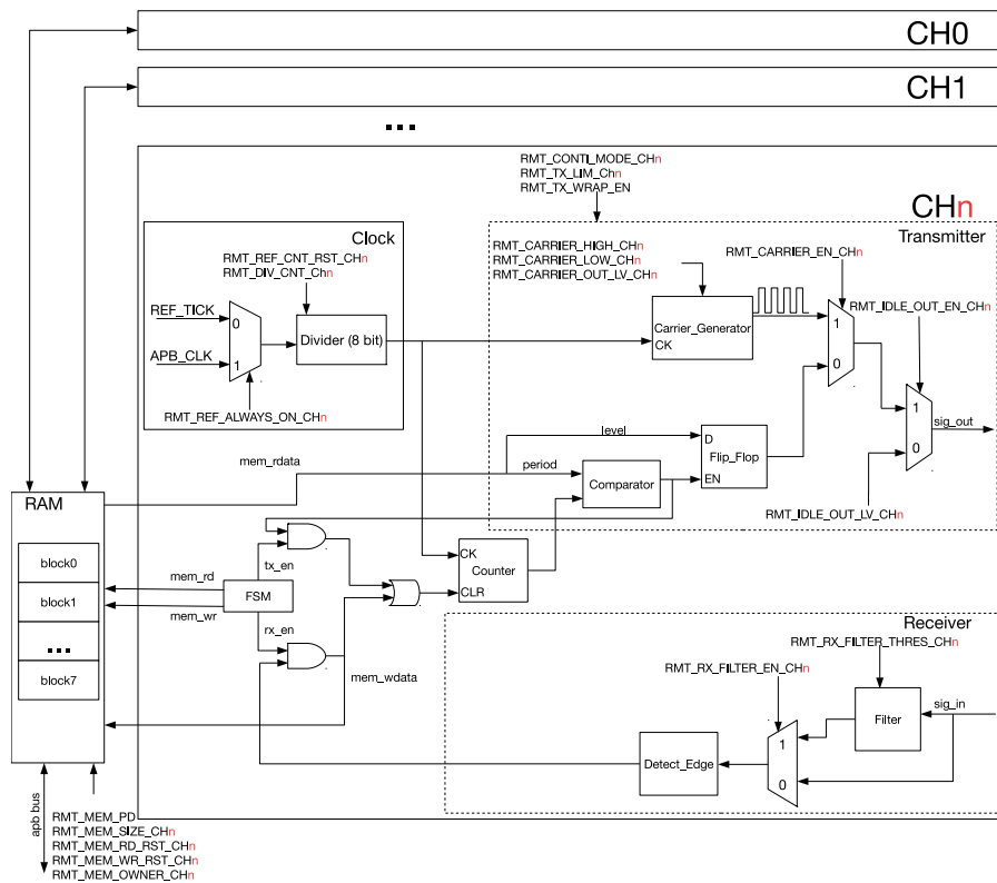
Figure 78: RMT Architecture
