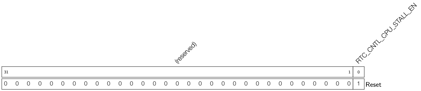
Register 29.8: RTC_CNTL_TIMER1_REG (0x0007)
