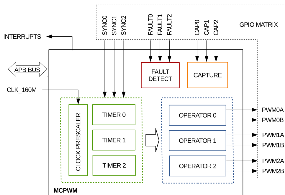
Figure 80: MCPWM Module Overview
