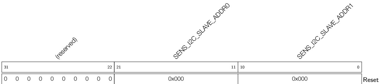
Register 28.3: SENS_SAR_SLAVE_ADDR1_REG (0x003c)
