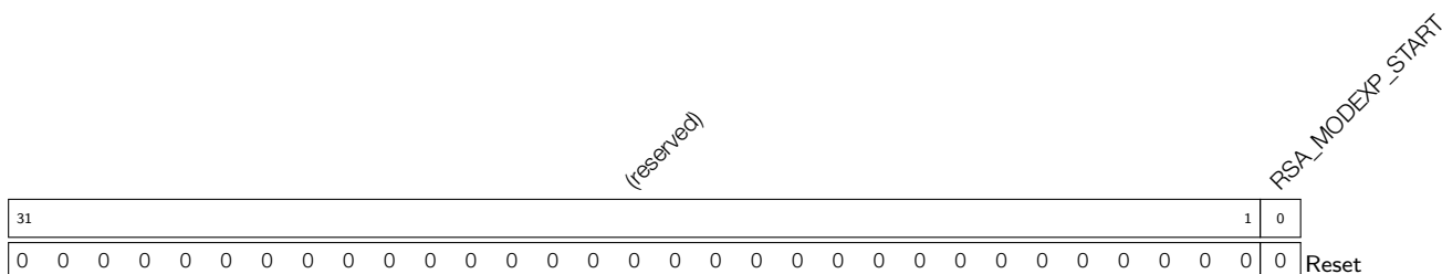
Register 22.3: RSA_MODEXP_START_REG (0x808)
