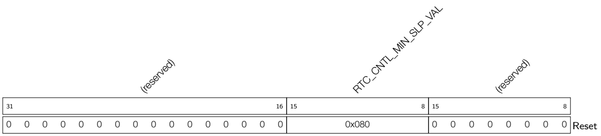
Register 29.10: RTC_CNTL_TIMER5_REG (0x000b)
