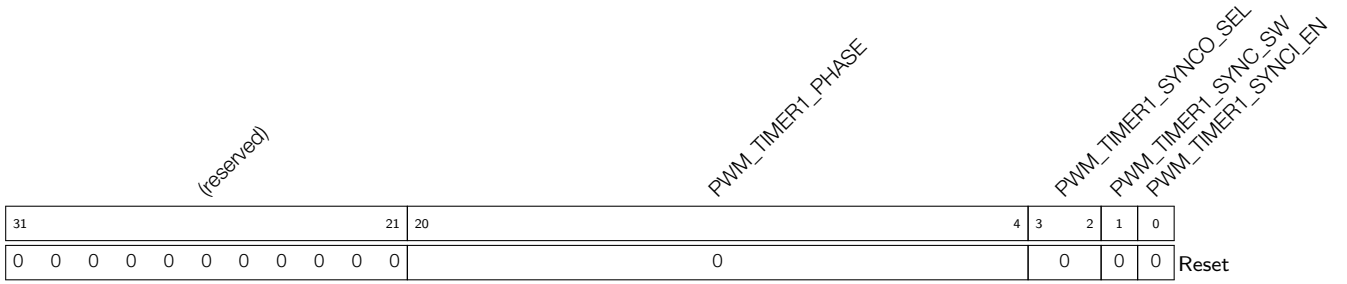
Register 15.8: PWM_TIMER1_SYNC_REG (0x001c)
