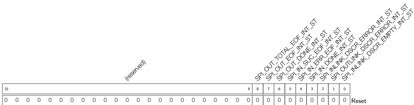
Register 7.31: SPI_DMA_INT_ST_REG (0x118)
