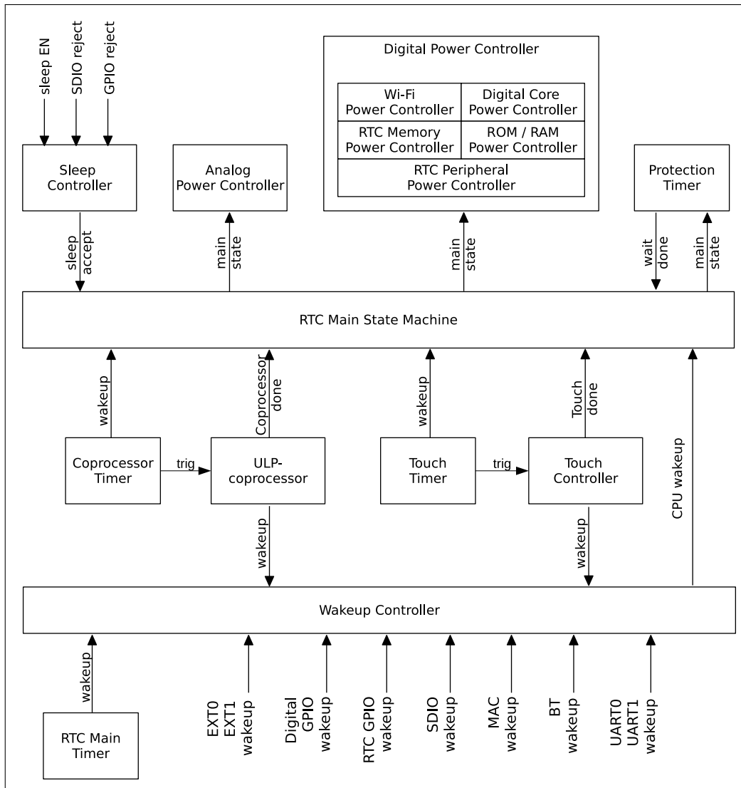
Figure 157: RTC Structure
