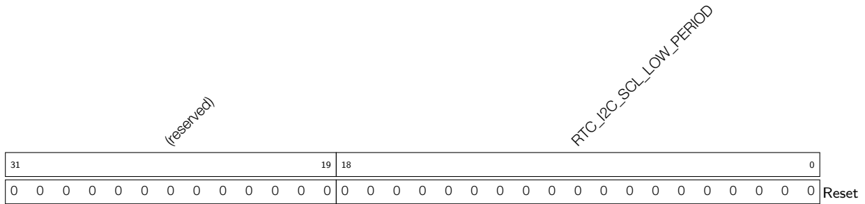
Register 28.8: RTC_I2C_SCL_LOW_PERIOD_REG (0x000)
