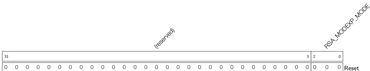
Register 22.2: RSA_MODEXP_MODE_REG (0x804)
