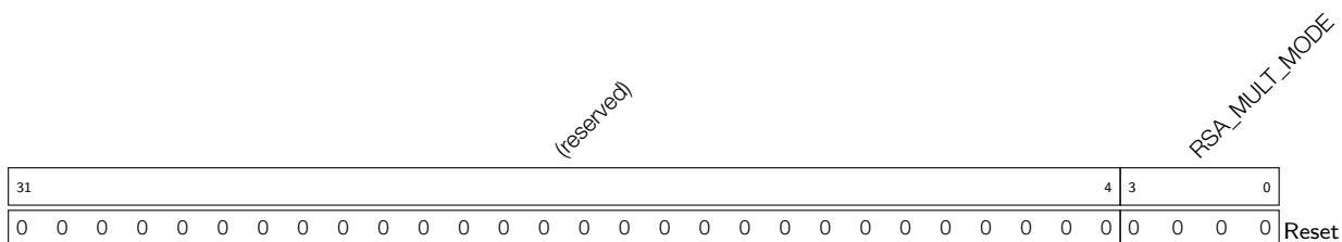
Register 22.4: RSA_MULT_MODE_REG (0x80C)
