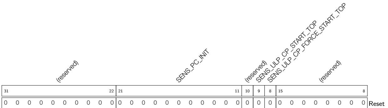
Register 28.2: SENS_SAR_START_FORCE_REG (0x002c)
