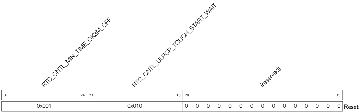
Register 29.9: RTC_CNTL_TIMER2_REG (0x0008)
