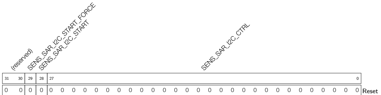
Register 28.7: SENS_SAR_I2C_CTRL_REG (0x0050)
