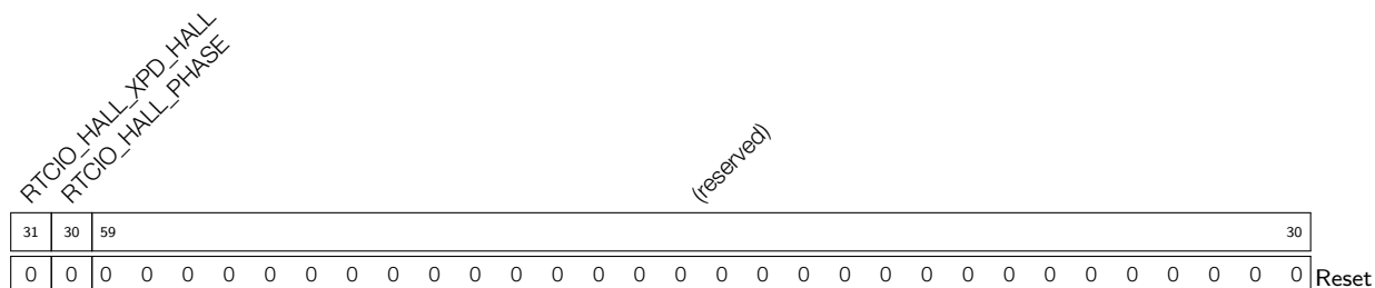
Register 4.47: RTCIO_HALL_SENS_REG (0x0078)
