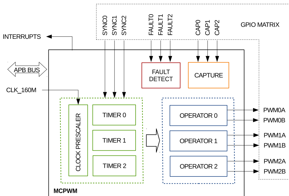
Figure 90: MCPWM Module Overview
