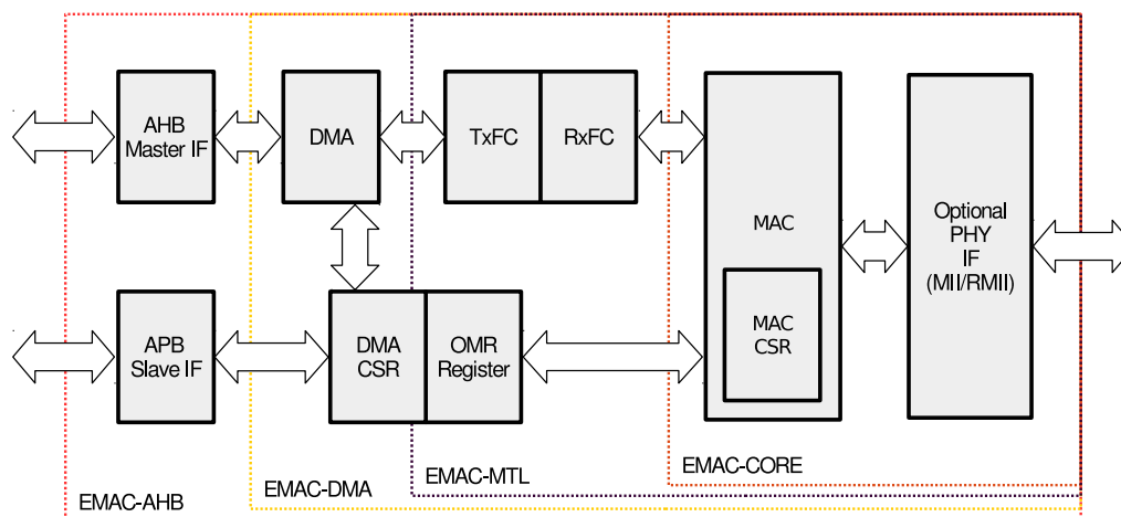
Figure 40: Ethernet Block Diagram
