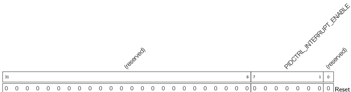
Register 27.1: PIDCTRL_INTERRUPT_ENABLE_REG (0x000)
