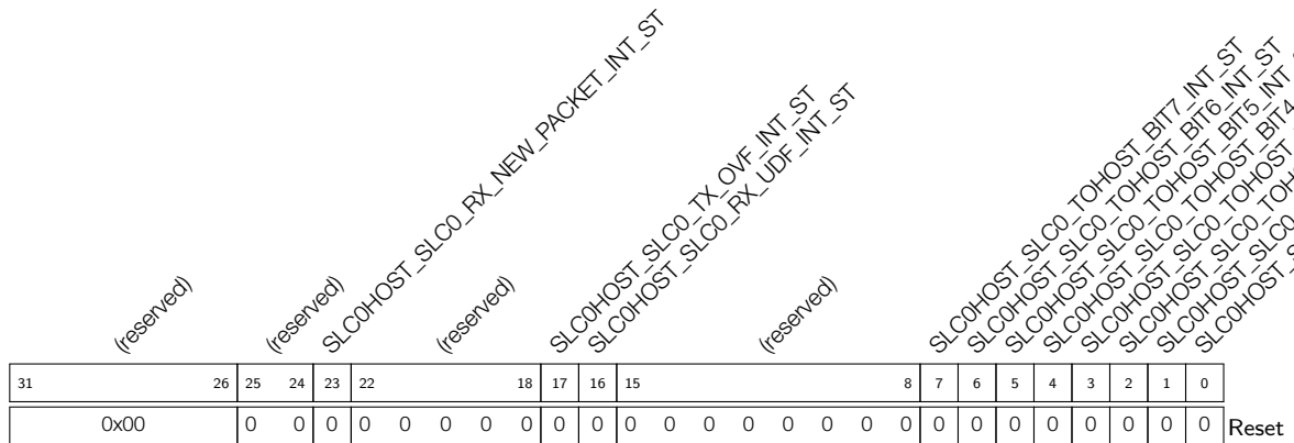
Register 8.16: SLC0HOST_INT_ST_REG (0x58)
