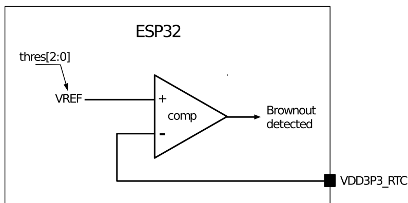
Figure 163: Brownout Detector
