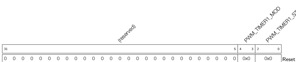
Register 16.7: PWM_TIMER1_CFG1_REG (0x0018)
