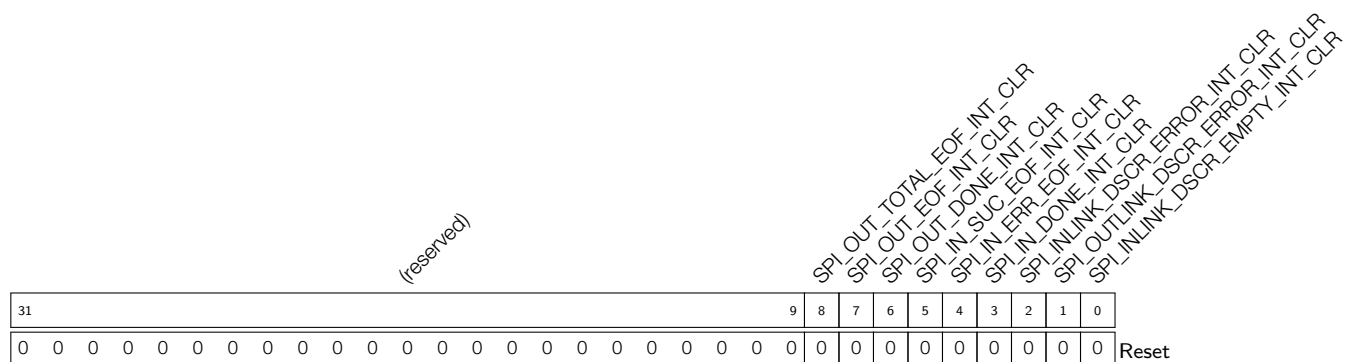
Register 7.32: SPI_DMA_INT_CLR_REG (0x11C)
