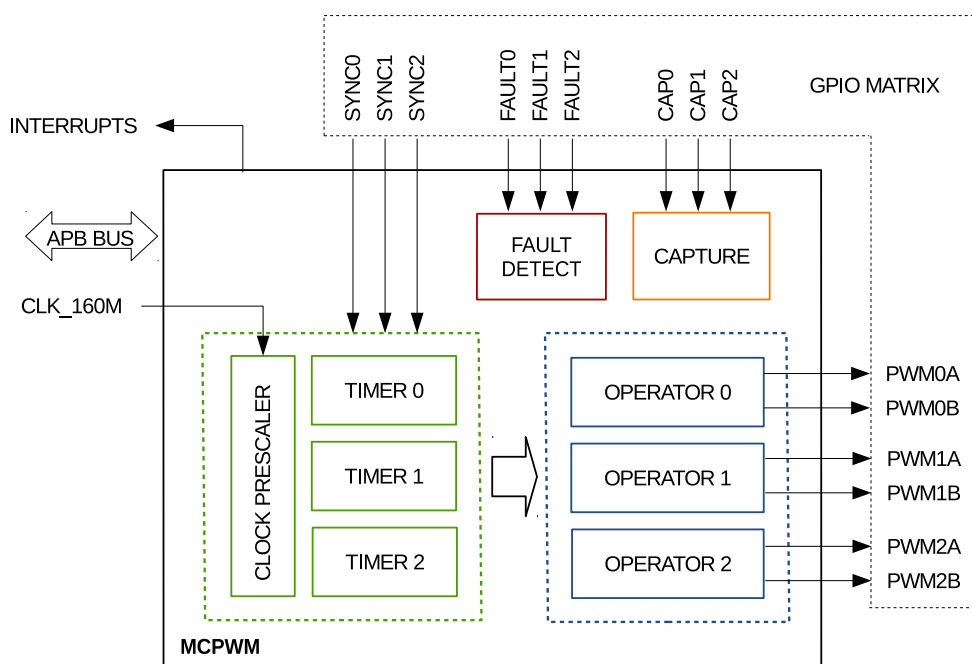
Figure 91: MCPWM Module Overview
