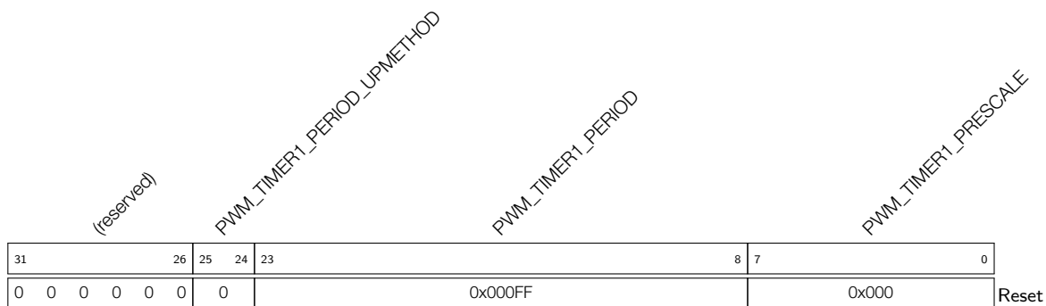
Register 16.6: PWM_TIMER1_CFG0_REG (0x0014)
