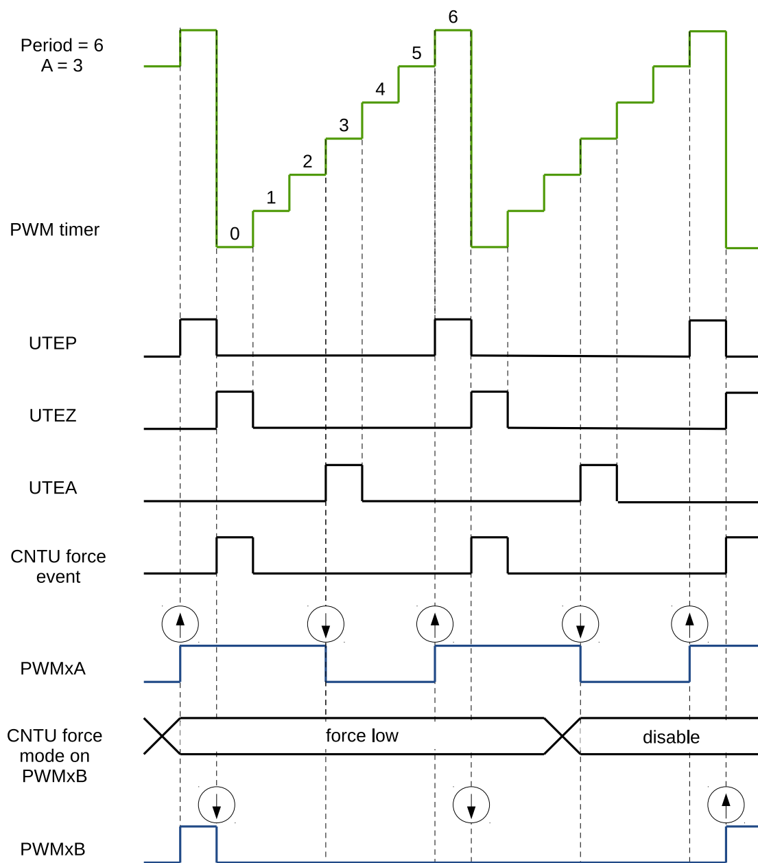
Figure 111: Example of a CNTU Software-Force Event on PWMxB
