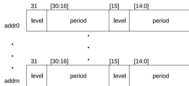
Figure 89: Data Structure
