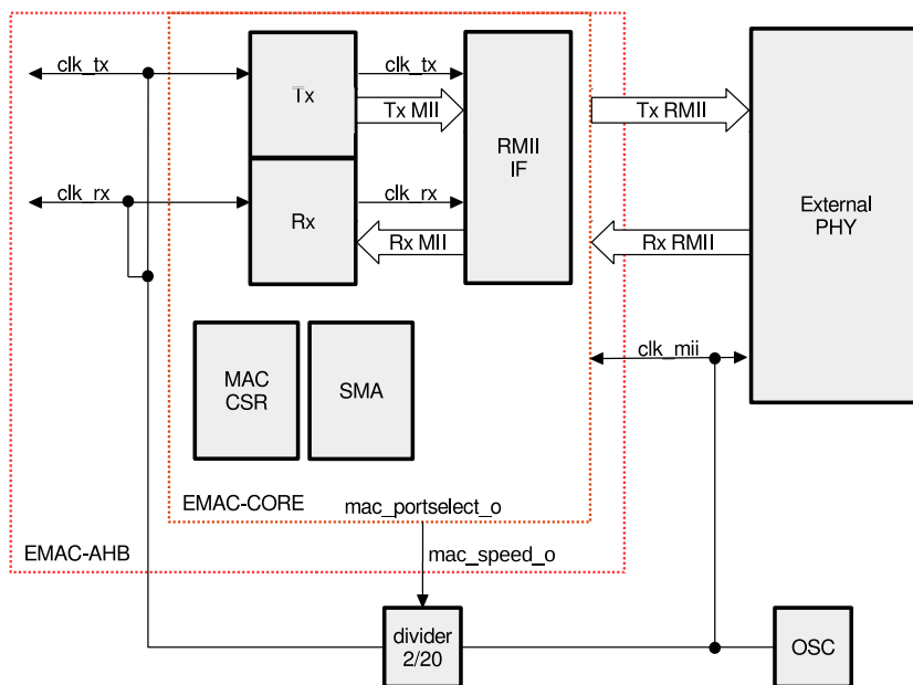
Figure 44: RMII Clock
