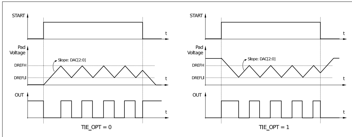
Figure 127: Touch Sensor Operating Flow
