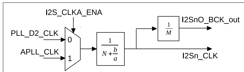
Figure 60: I2S Clock
