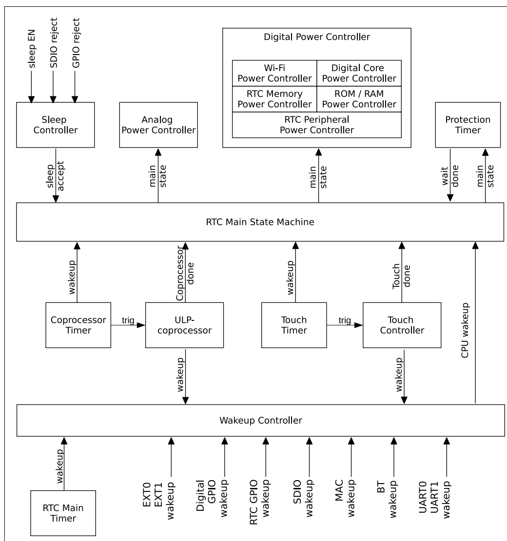
Figure 167: RTC Structure
