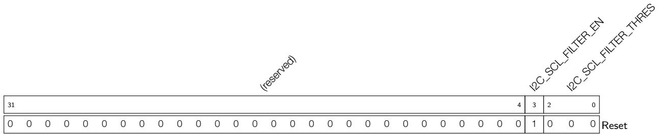
Register 11.19: I2C_SCL_FILTER_CFG_REG (0x0050)
