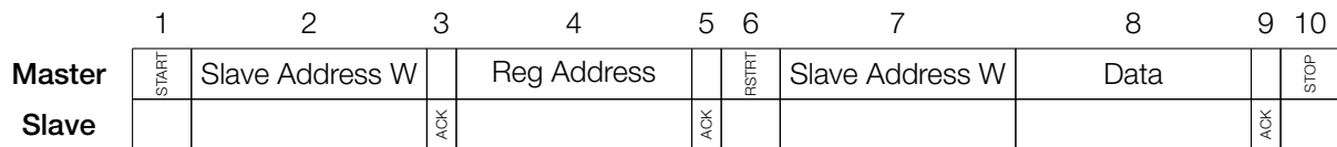
Figure 161: I2C Write Operation
