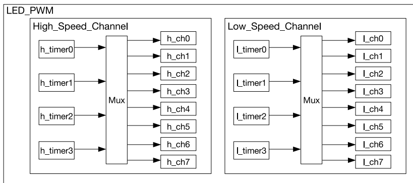
Figure 83: LED_PWM Architecture
