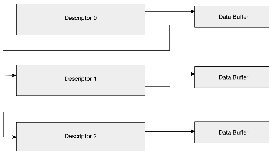
Figure 36: Descriptor Chain
