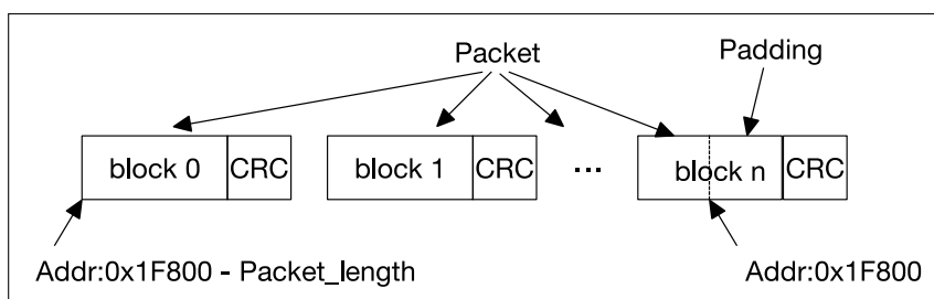
Figure 21: SDIO Bus Packet Transmission
