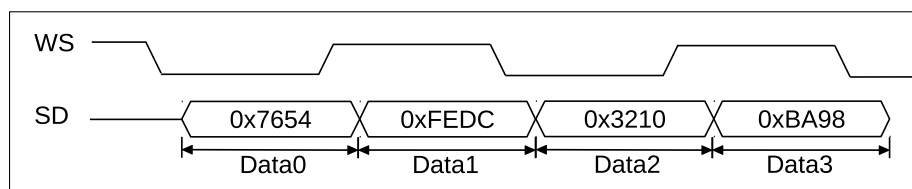
Figure 65: The First Stage of Receiving Data
