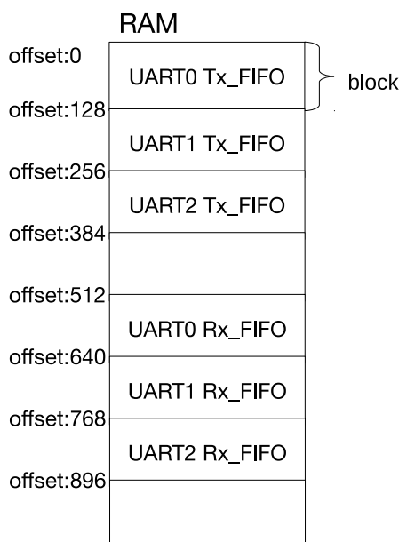
Figure 79: UART shared RAM
