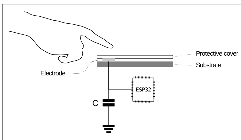
Figure 125: Touch Sensor
