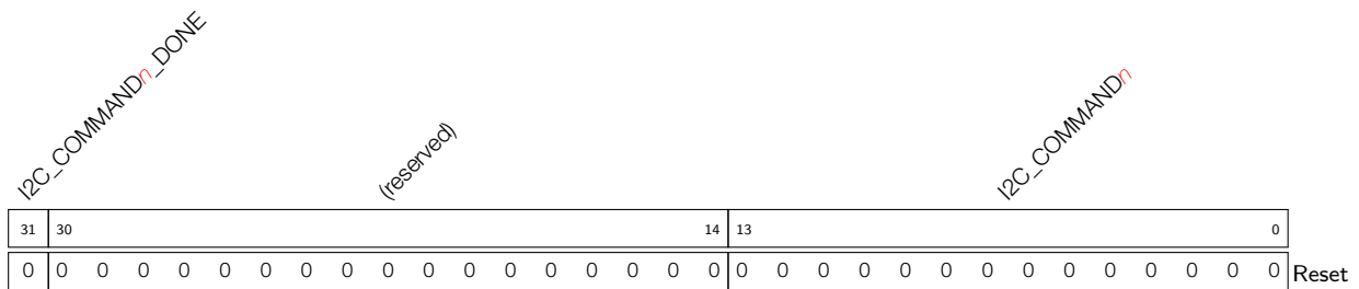
Register 11.21: I2C_CMD n _REG ( n : 0-15) (0x58+4* n )
