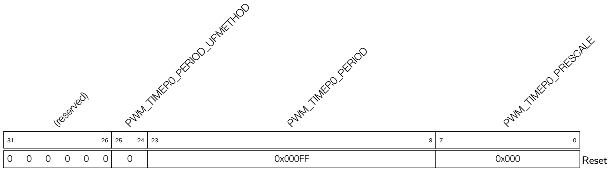
Register 16.2: PWM_TIMER0_CFG0_REG (0x0004)
