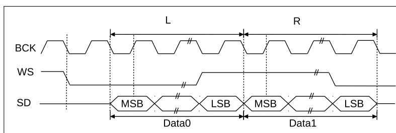
Figure 61: Philips Standard
