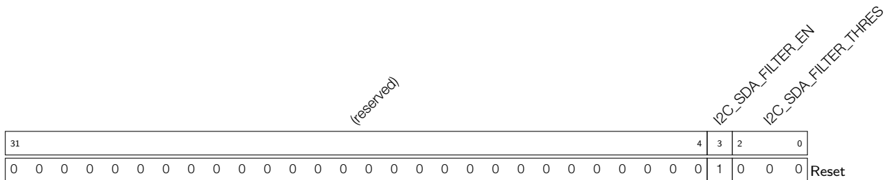
Register 11.20: I2C_SDA_FILTER_CFG_REG (0x0054)
