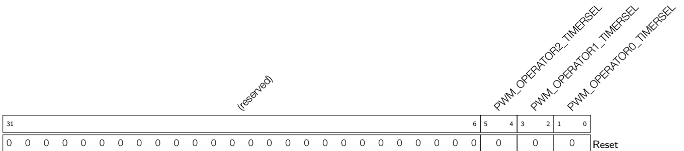
Register 16.15: PWM_OPERATOR_TIMERSEL_REG (0x0038)
