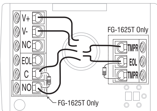
Normally Open Loop/With EOL Resistor
