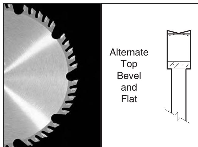
Figure 41. Combination blade.
