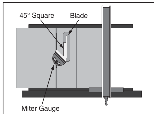
Figure 126. Example of checking 45° stop on miter gauge.
