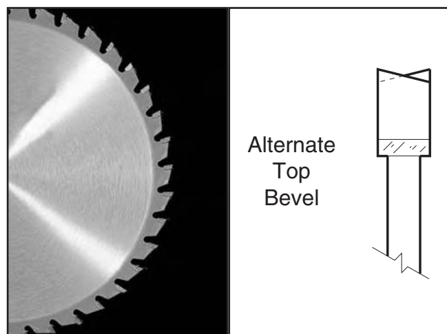
Figure 40. Crosscutting blade.
