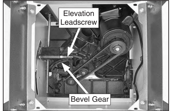
Figure 108. Bevel gear and elevation leadscrew.
