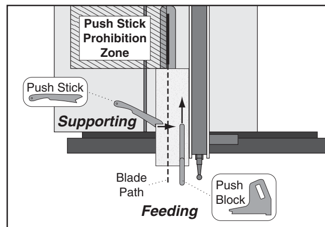
Figure 89. Using a push block and push stick to make a rip cut.
