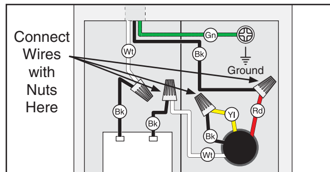
Figure 4. Saw rewired to 220V.
