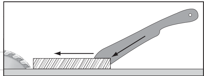
Figure 86. Side view of a push stick in-use.
