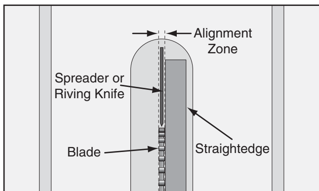
Figure 49. Spreader/ripping knife alignment zone.
