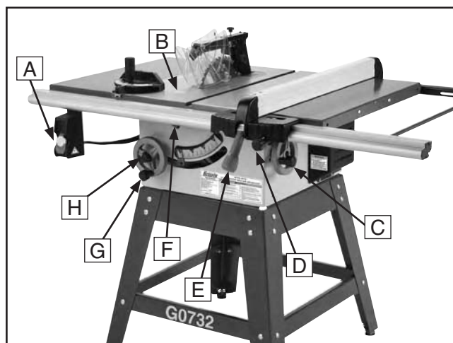
Figure 36. Basic table saw controls G0732.
