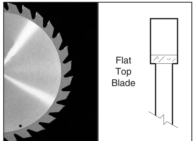
Figure 39. Ripping blade.
