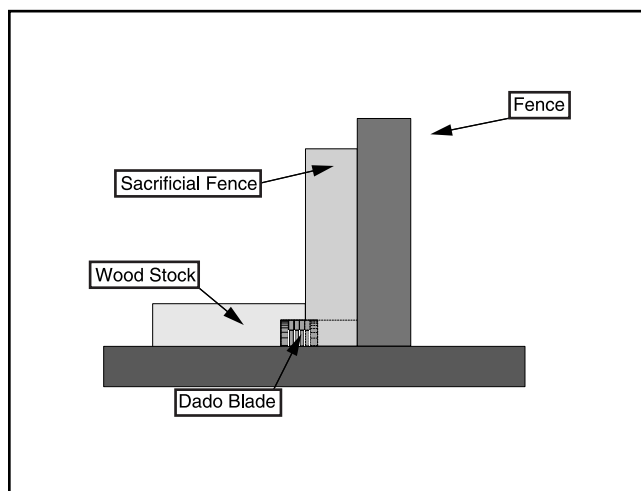
Figure 36. Rabbet cutting.
