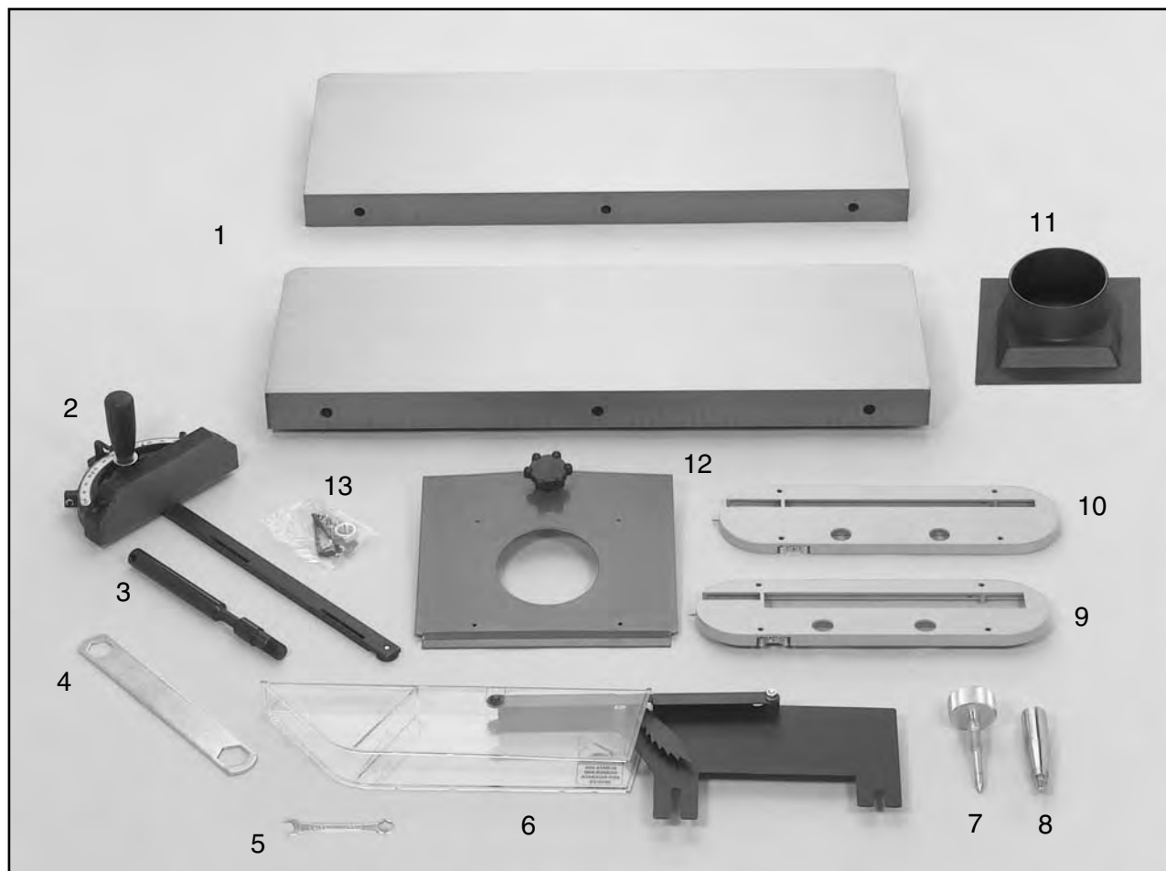
Figure 9C. G1023Z Series component layout.
