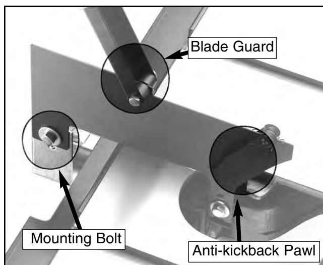
Figure 18. Blade guard and splitter in place.
