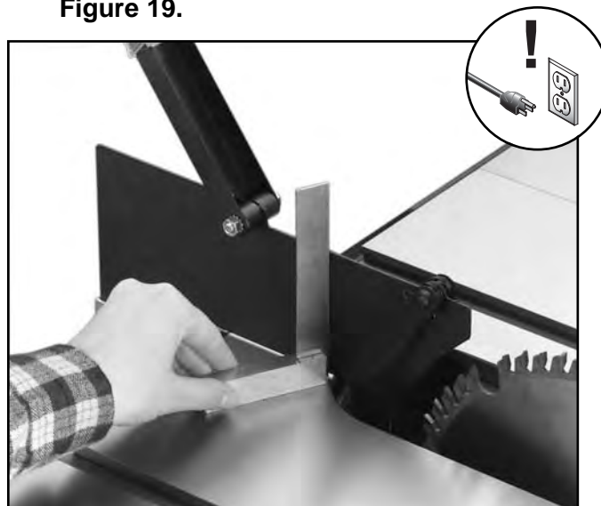
Figure 19. Blade splitter square to table.
