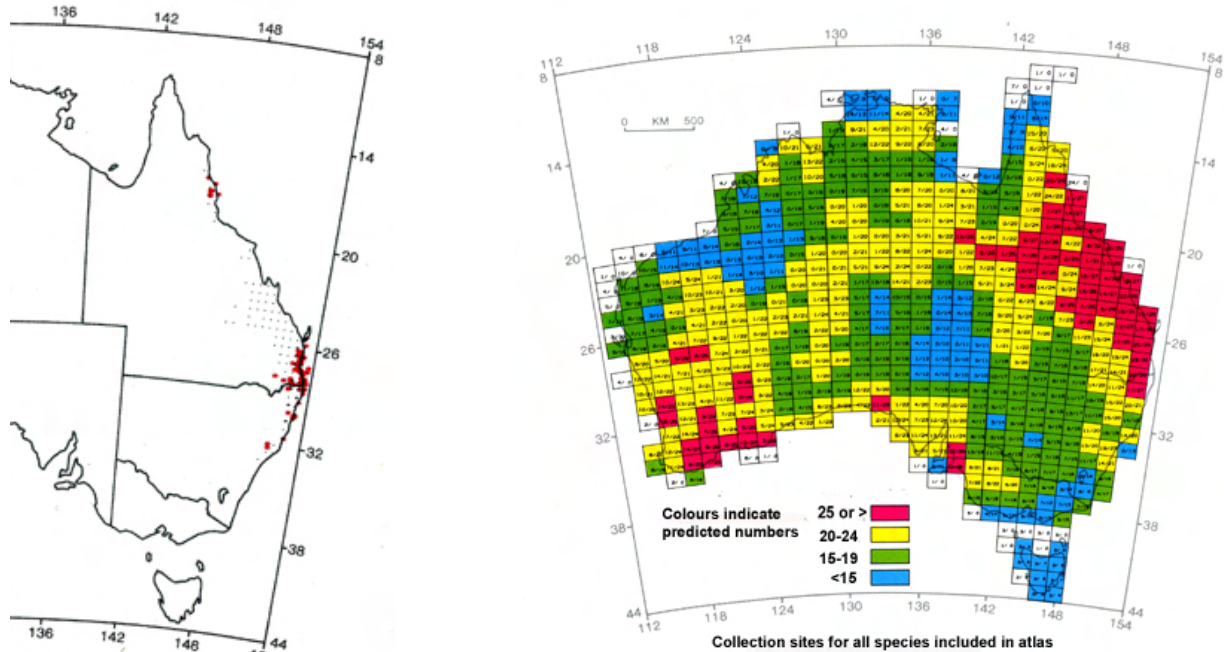
Fig. 5. Left-hand image - Potential distribution for Tropidechis carinatis in Australia. Red stars indicate known collections, dots show modelled distribution. Right-hand image shows predicted numbers of species in each 1^{\circ} \times 1.5^{\circ} cell. From Longmore (1986) with permission of Australian Biological Resources Study.
