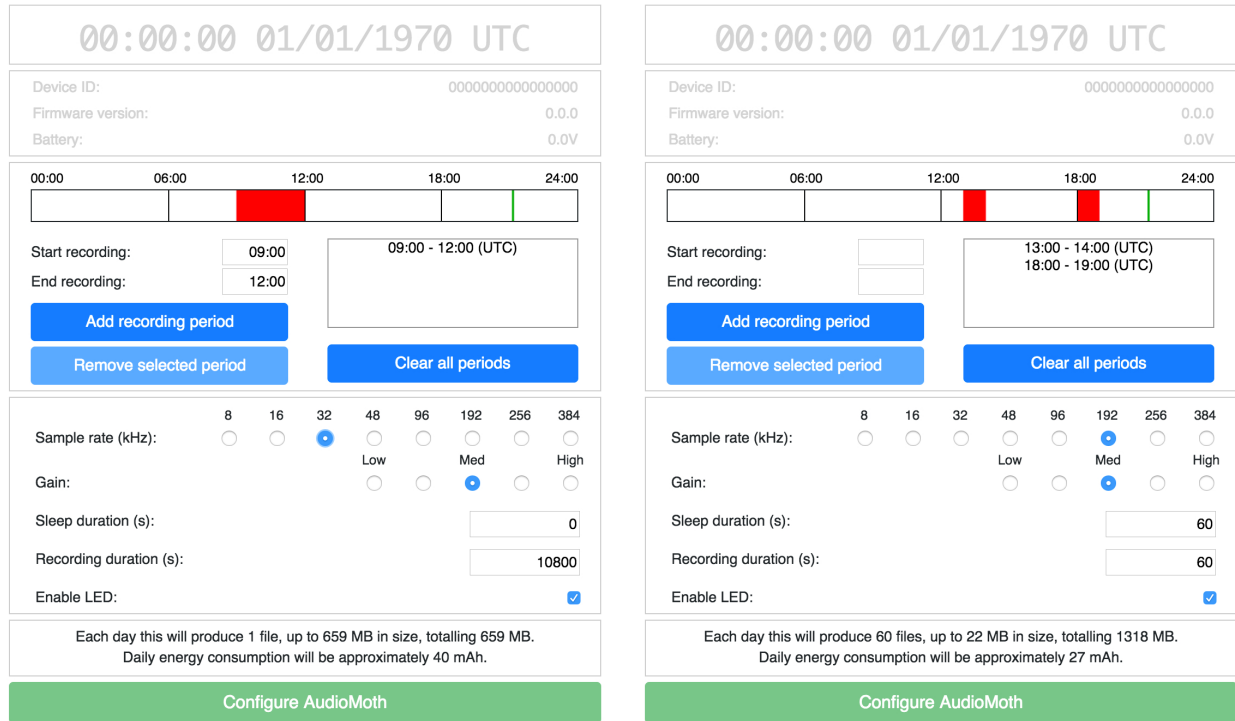
Figure 3: Two example programs
