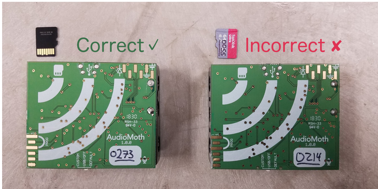
Figure 4: Correct way to insert SD card
