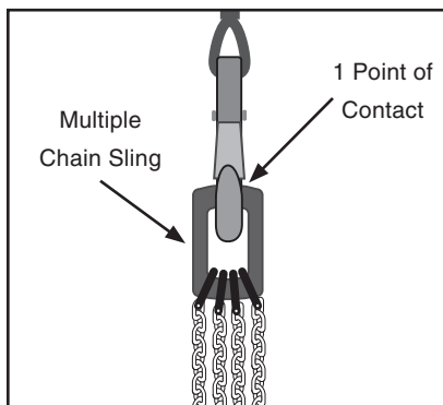
Figure 5. Example of proper hardware.
