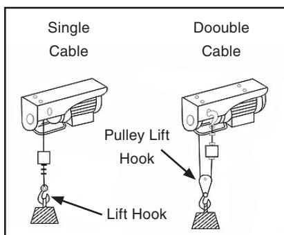
Figure 8. Cable options.
