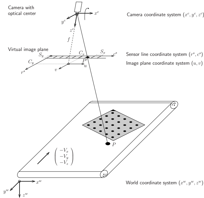
Figure 3.5: Line scan camera rotated around the x-axis.
