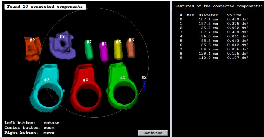
Figure 2.29: Features calculated for the connected components of a 3D object model.
