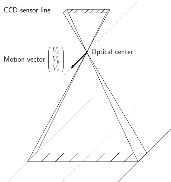
Figure 2.17: Principle of line scan image acquisition.
