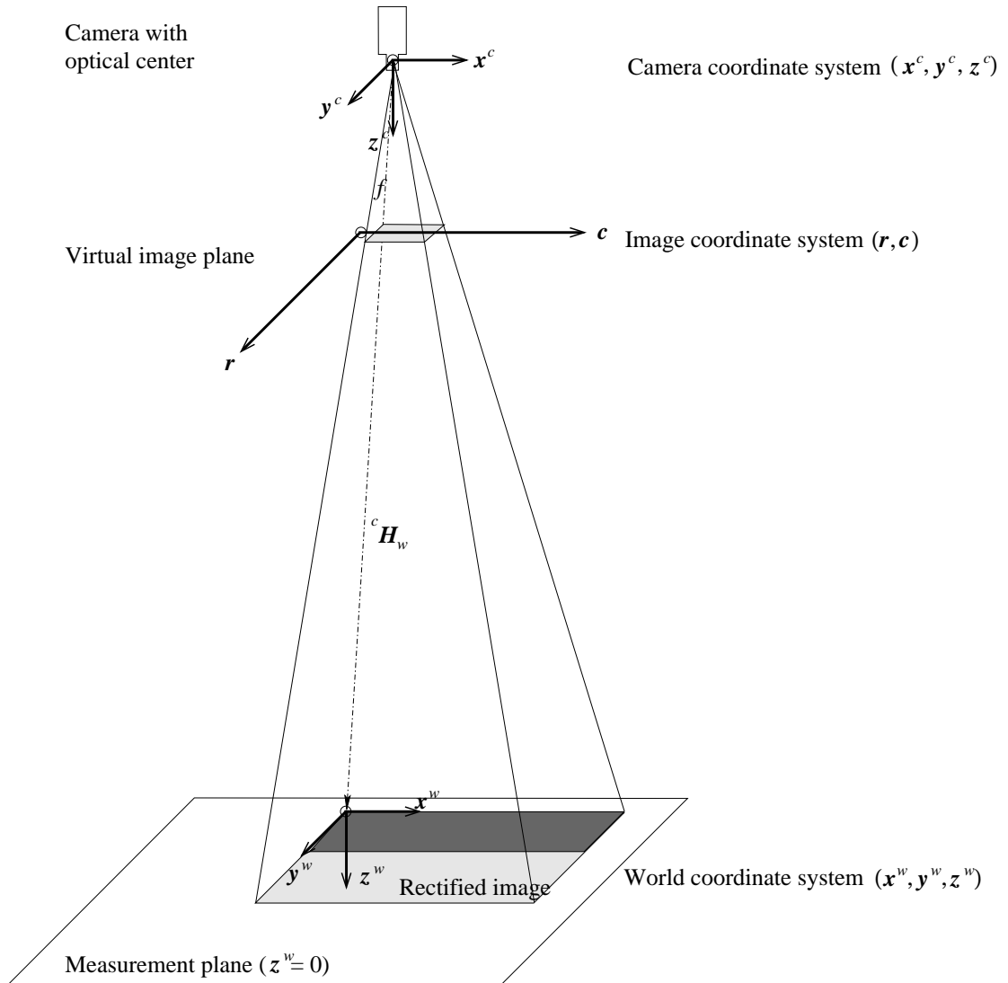
Figure 3.12: Projection of the image into the measurement plane with part of the rectified image lying outside the image area.
