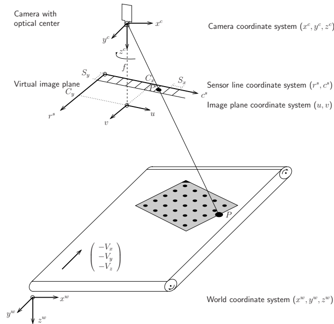
Figure 3.4: Line scan camera rotated around the optical axis.
