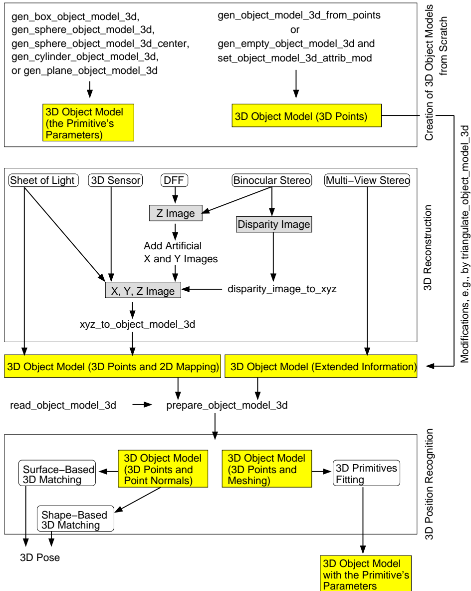
Figure 2.23: Overview on the 3D object model.
