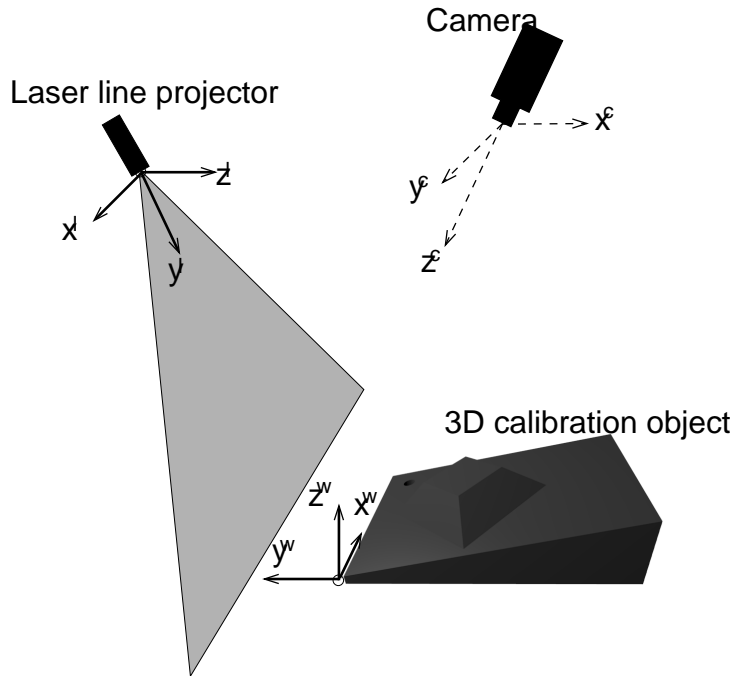
Figure 6.9: Sheet-of-light setup with 3D calibration object.
