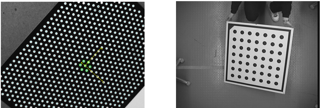
Figure 3.6: HALCON calibration plates of different materials and sizes: (a) with hexagonally arranged marks and (b) with rectangularly arranged marks.
