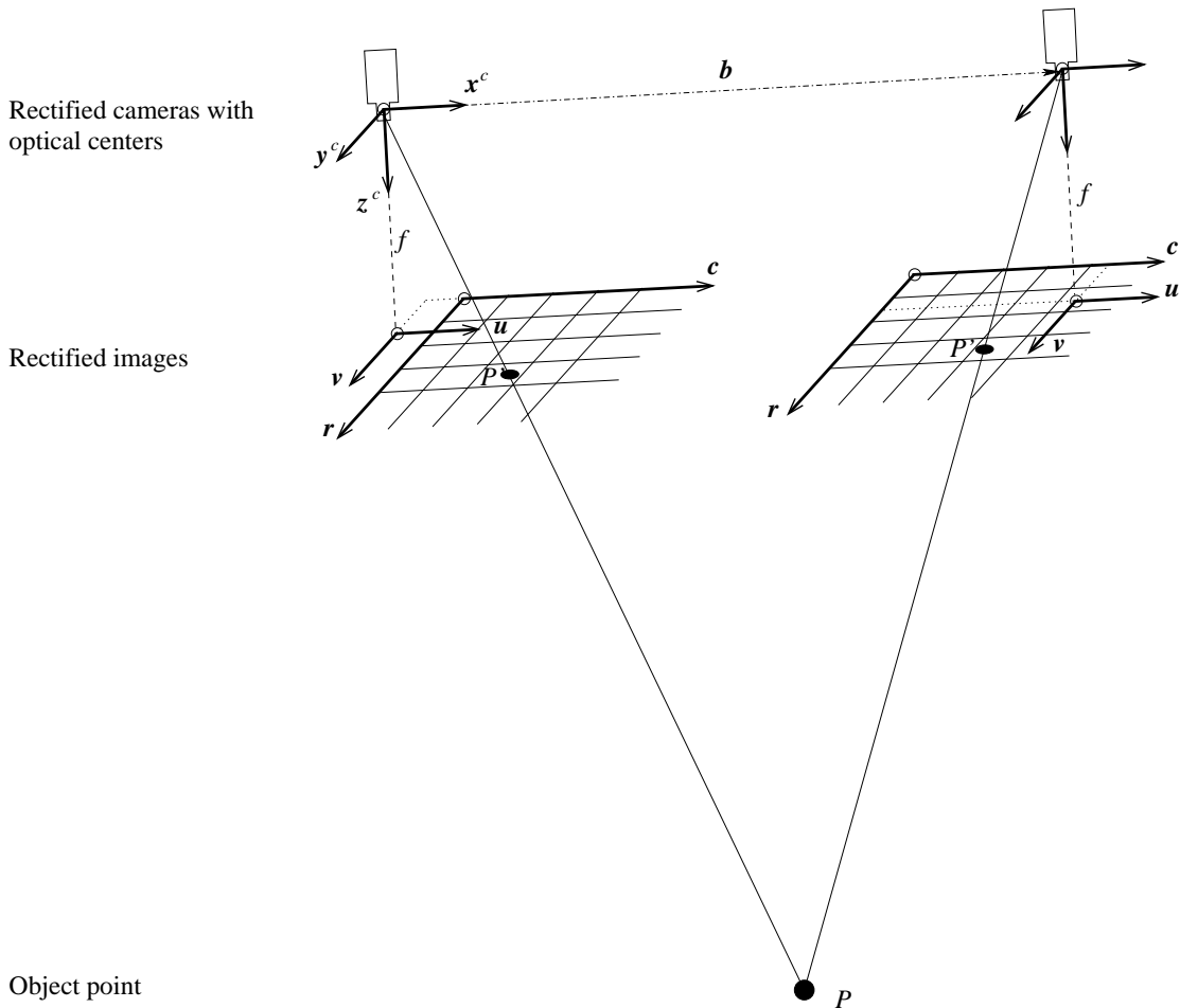
Figure 5.12: Rectified stereo camera system.
