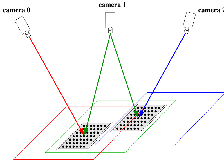
Figure 5.7: Cameras are connected in a chain.
