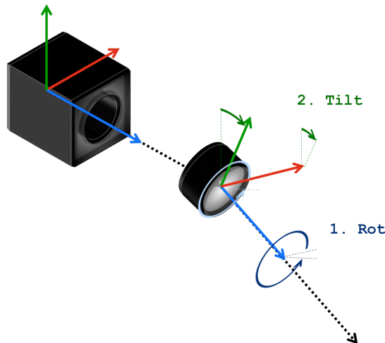
Figure 2.14: The tilt of the lens is described by the two parameters Tilt and Rot . Rot describes the orientation of the tilt axis. Tilt describes the actual tilt of the lens.
