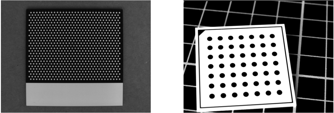
Figure 3.1: The HALCON calibration plates.
