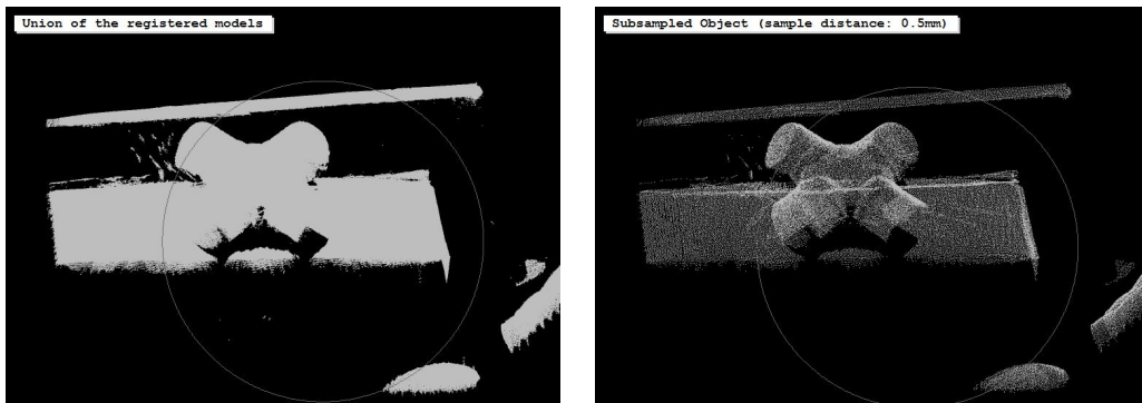
Figure 2.34: The 3D object models (left) united into a single 3D object model and (right) subsampled and smoothed.
