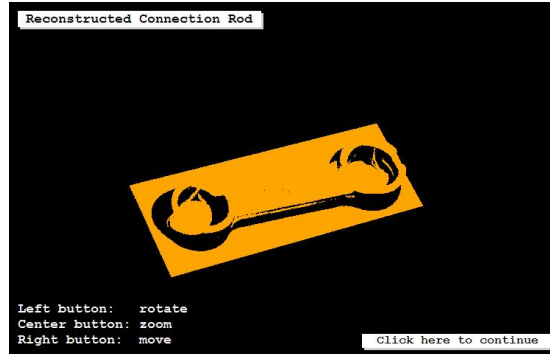
Figure 6.15: Result of calibrated sheet-of-light measurement: 3D object model.
