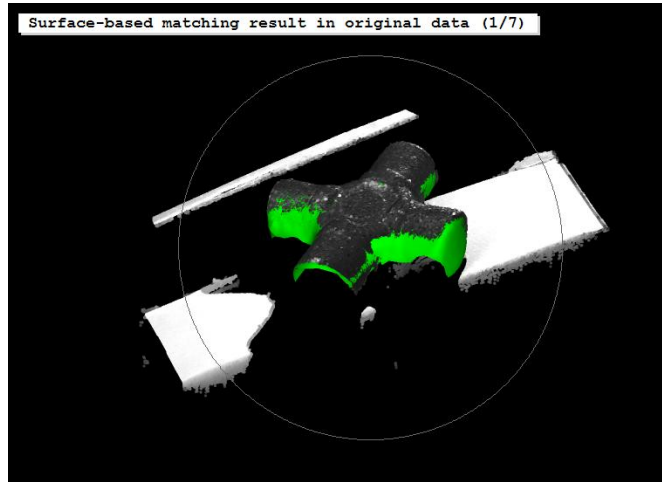
Figure 2.37: Result of surface-based 3D matching in one of the views of the training data.
