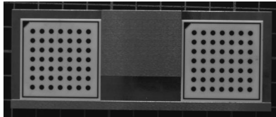
Figure 9.3: Calibration object for two-camera setup.
