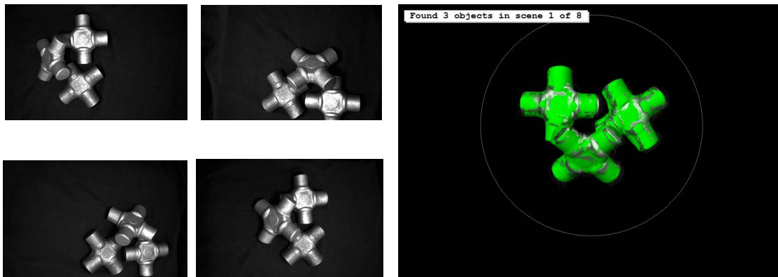
Figure 2.38: Result of surface-based 3D matching in a scene obtained from multi-view stereo images.
