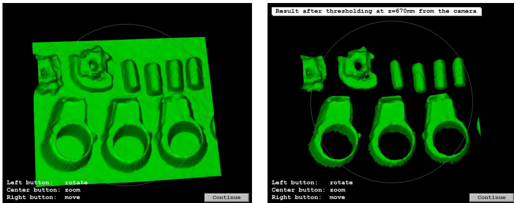
Figure 2.26: 3D object model (left) in its initial state and (right) after removing points of the background using a threshold.
