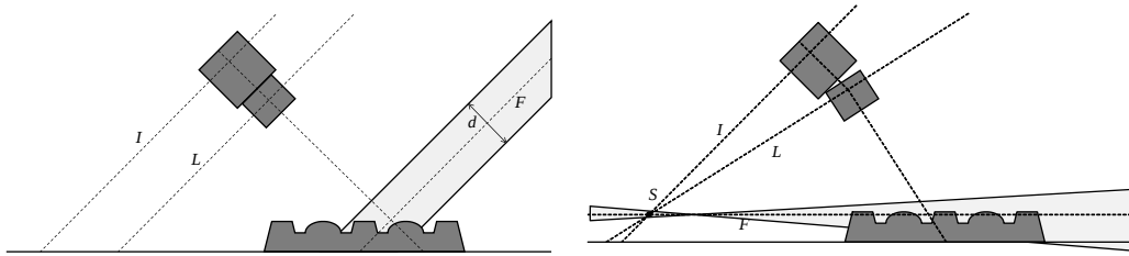
Figure 2.15: The Scheimpflug principle: Left: Without tilt lens the focus plane F is parallel to the image plane I . Therefore, the object is only partly in focus if it exceeds the depth of field d . Right: When using a tilt lens, the focus plane, the image plane, and the lens plane L are intersecting in the Scheimpflug line S . Using this principle, a planar object can be completely in focus even if it is viewed from an angle.
