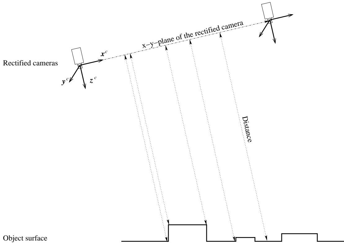
Figure 5.17: Distances of the object surface from the x - y -plane of the coordinate system of the first rectified camera.
