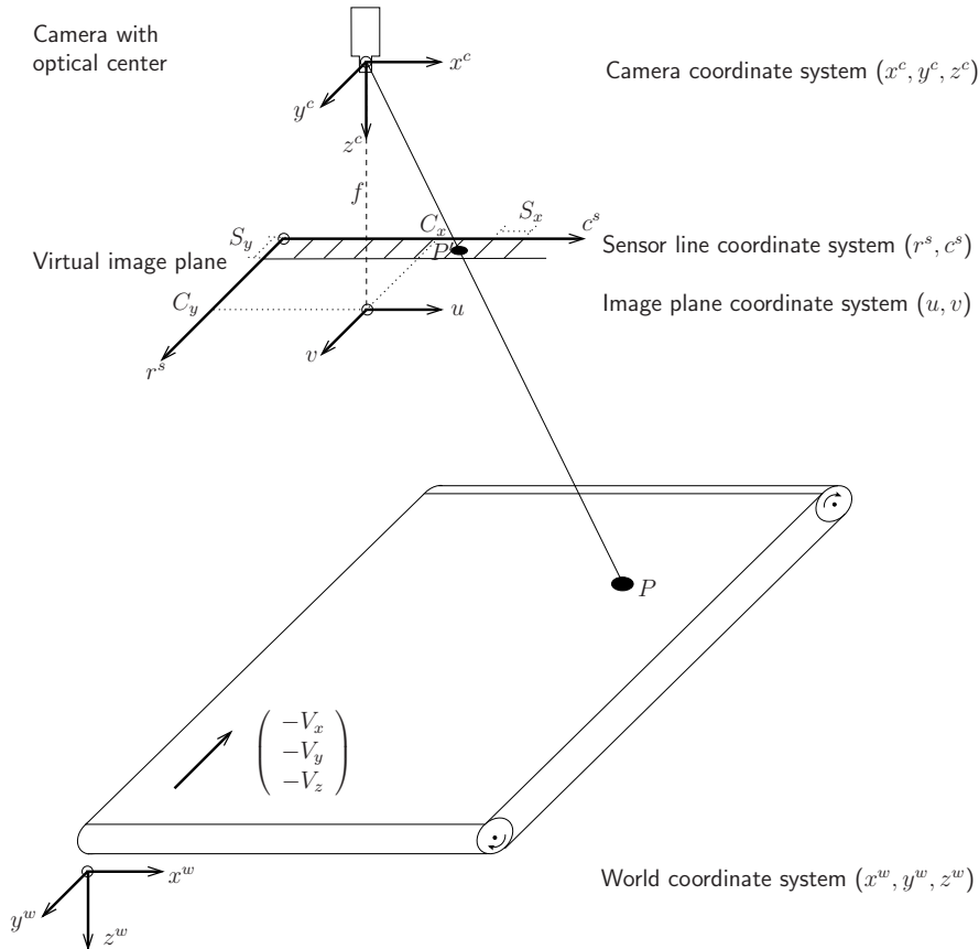
Figure 2.18: Coordinate systems in regard to a line scan camera.
