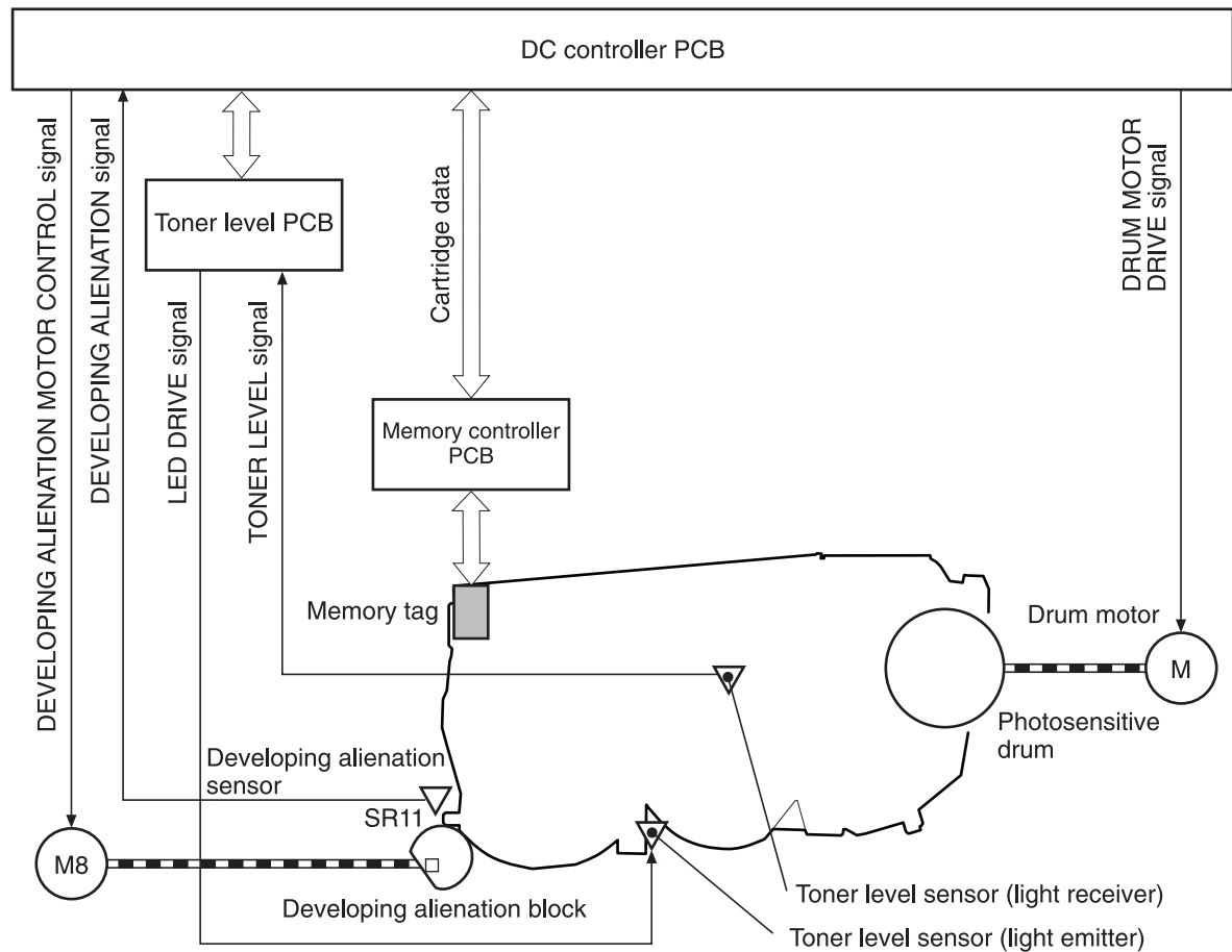
Figure 5-26 Print cartridge
