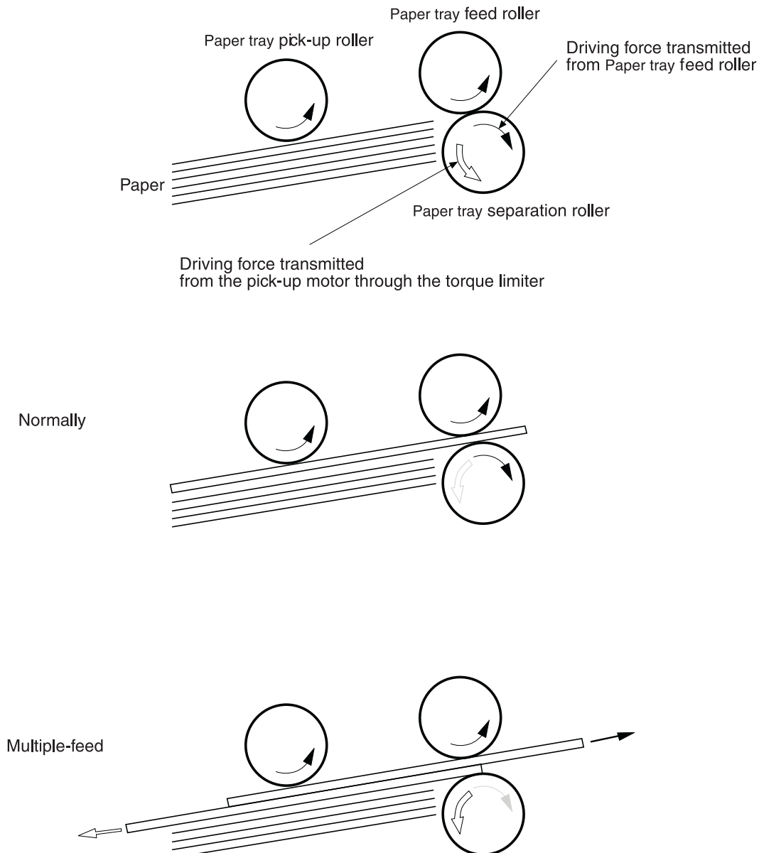
Figure 5-40 Media lift-up
