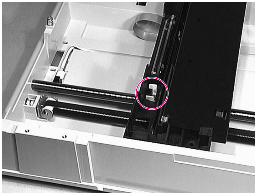
Figure 6-254 Felt Pad
