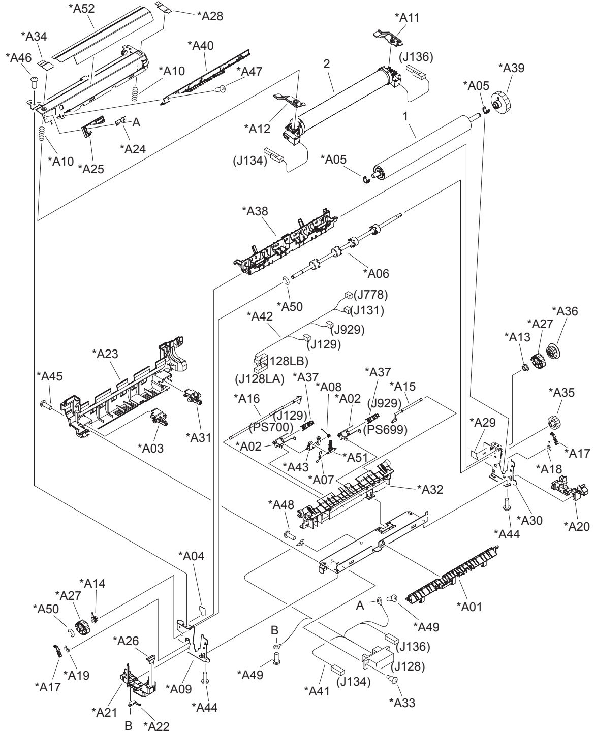
Figure 8-13 Fusing assembly
