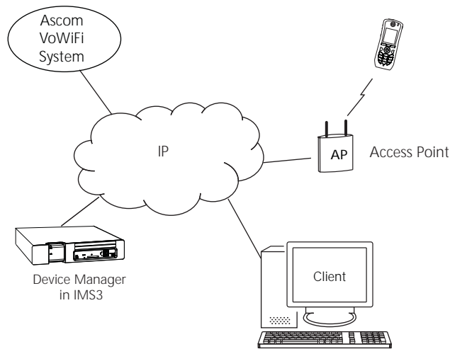
Figure 3. Configuration of VoWiFi Handsets via Over-the-Air (OTA)
