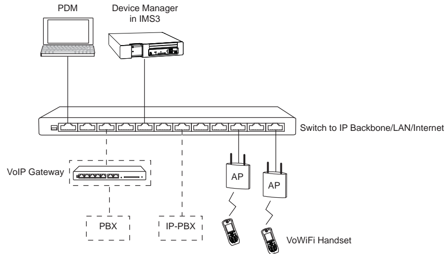
Figure 1. Ascom VoWiFi System
