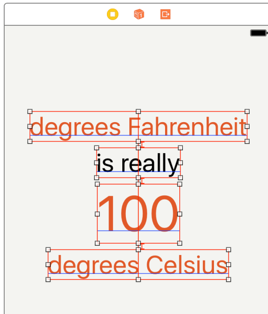
Figure 4.2 Ambiguous frames for the labels
