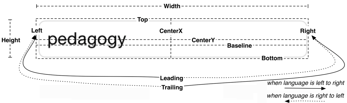
Figure 3.16 Layout attributes defining an alignment rectangle of a view
