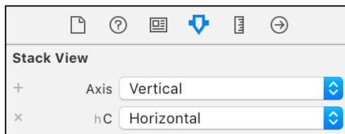
Figure 17.8 Customizing the axis
