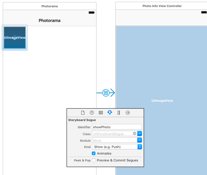
Figure 21.14 Navigation to a photo
