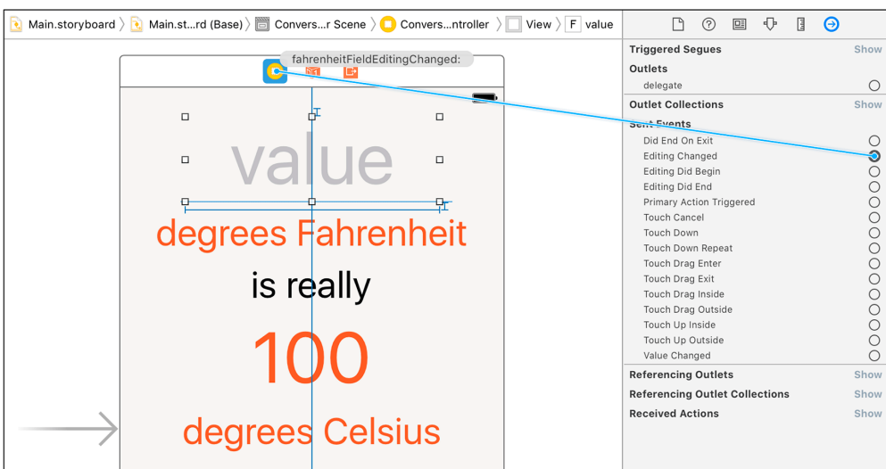
Figure 4.10 Connecting the editing changed event
