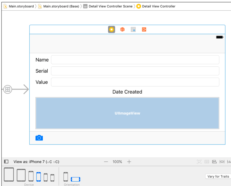
Figure 17.6 DetailViewController viewed as iPhone 7 landscape
