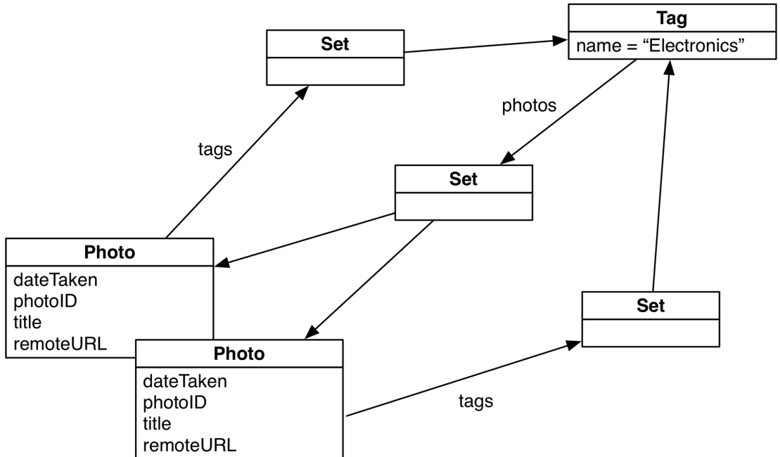
Figure 23.2 Entities in Photorama
