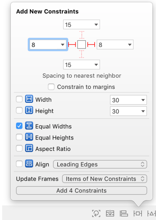
Figure 11.5 Adding new constraints
