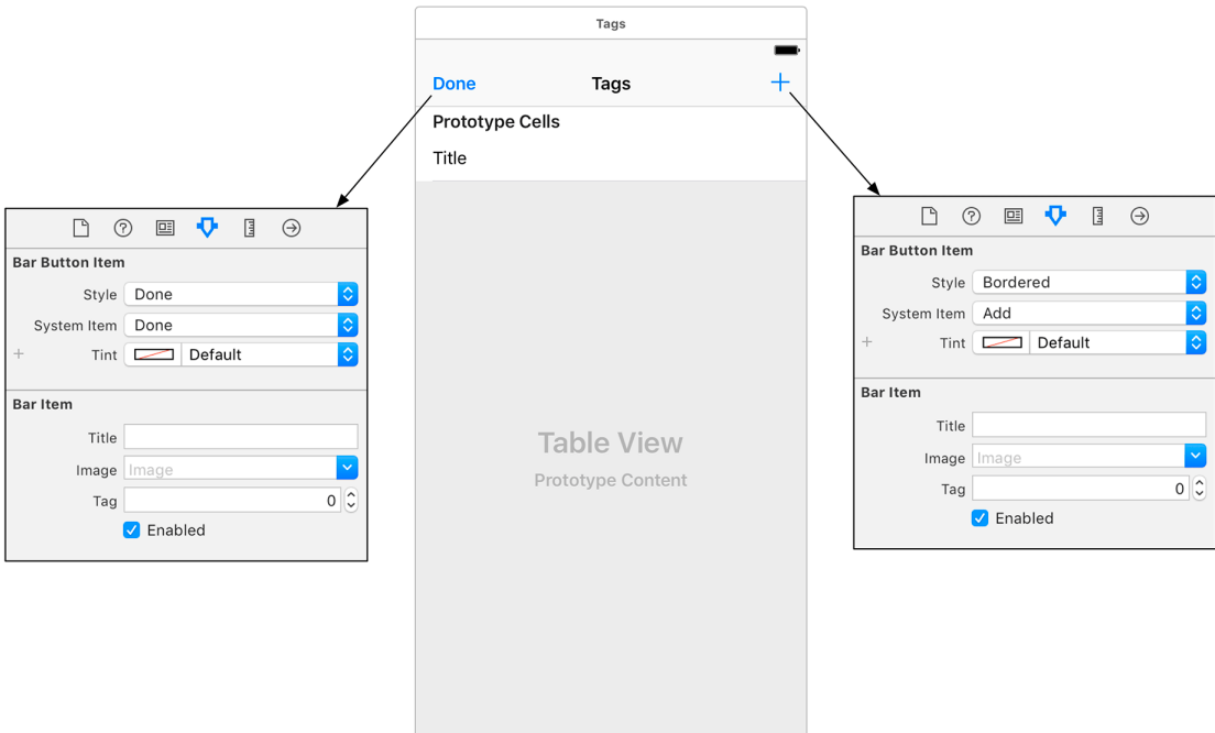
Figure 23.9 Bar button item attributes
