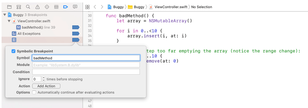
Figure 9.16 Adding a symbolic breakpoint
