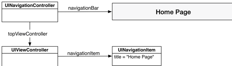
Figure 14.11 UINavigationItem with title
