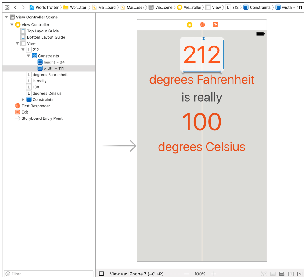
Figure 3.21 Selecting the width constraint
