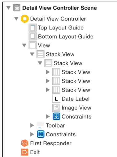
Figure 17.3 Expanding the document outline
