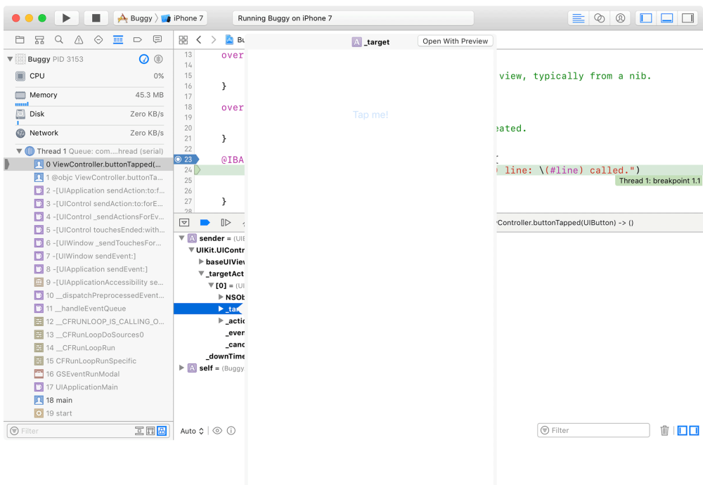
Figure 9.8 Inspecting variables in the variables view
