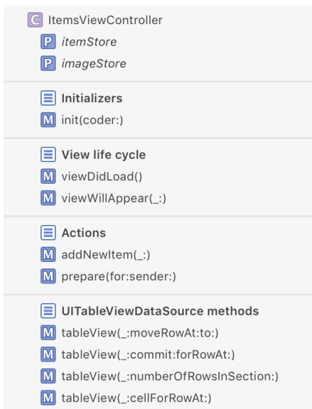
Figure 15.19 File popover with // MARK:s
