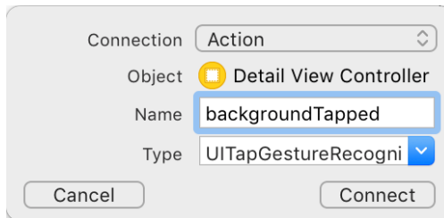
Figure 14.9 Configuring a UITapGestureRecognizer action
