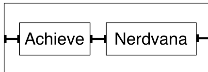
Figure 13.4 Two labels side by side
