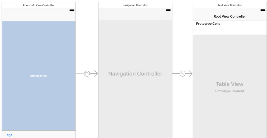
Figure 23.7 Adding the tags view controller
