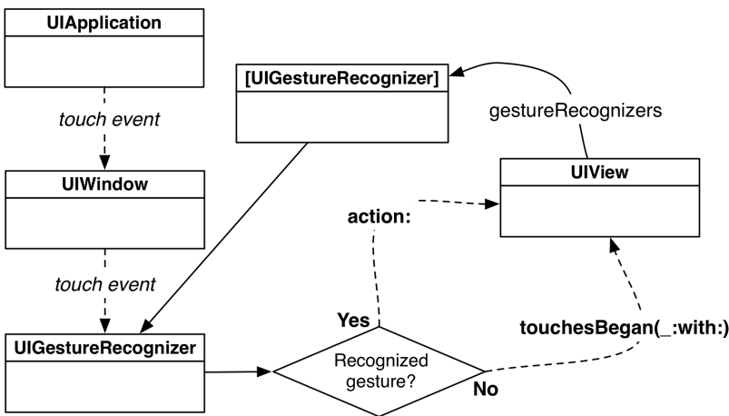
Figure 19.2 Gesture recognizers intercept touches
