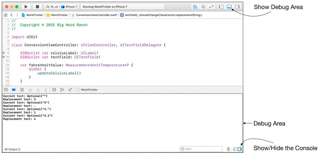
Figure 4.12 Printing to the console
