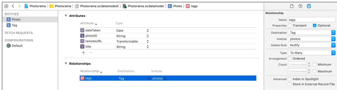
Figure 23.4 Creating the tags relationship
