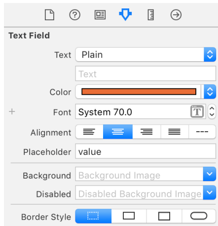
Figure 4.5 Text field attributes inspector
