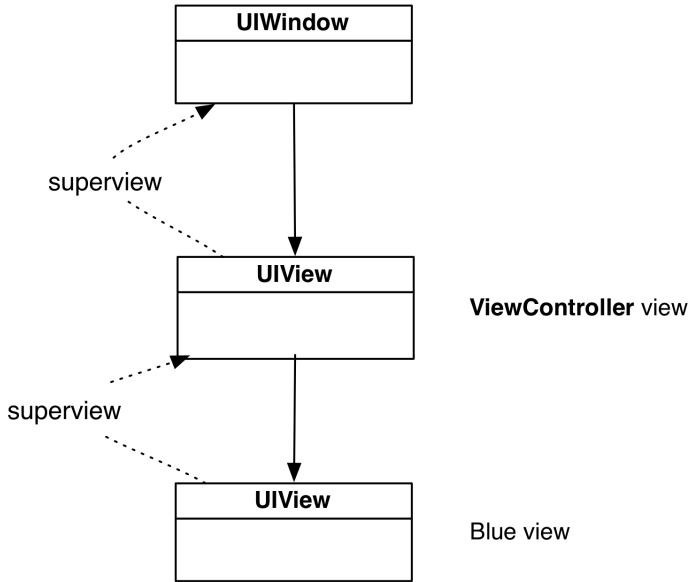
Figure 3.7 Current view hierarchy
