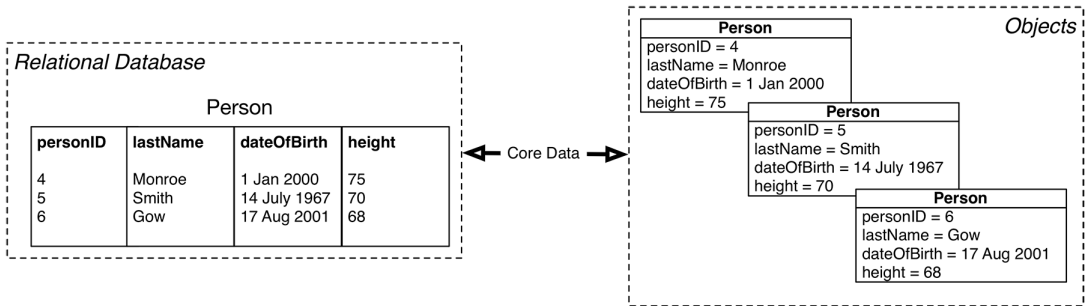
Figure 22.1 Role of Core Data
