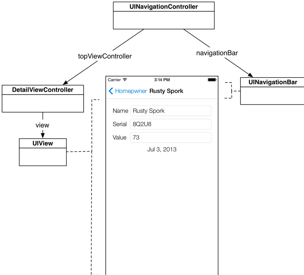
Figure 14.4 A UINavigationController 's view
