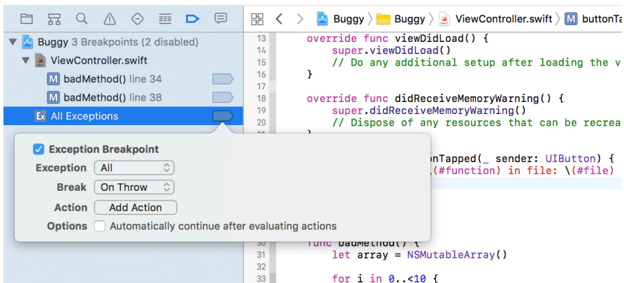
Figure 9.15 Adding an exception breakpoint
