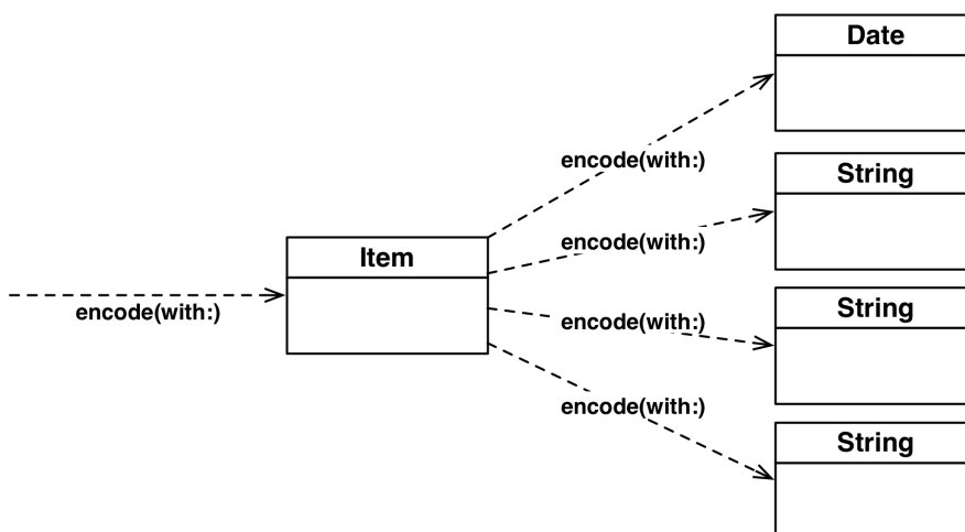
Figure 16.2 Encoding an object
