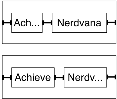
Figure 13.6 Compressed ambiguous layout
