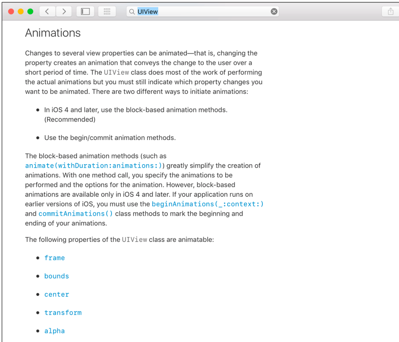
Figure 8.1 UIView animation documentation
