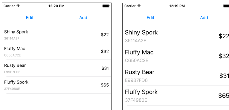
Figure 12.6 ItemCell with Dynamic Type supported
