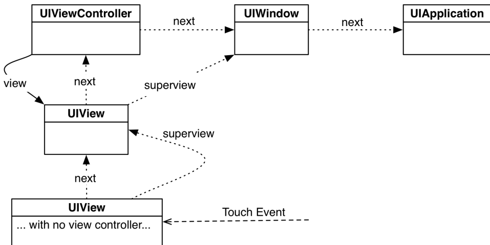
Figure 18.8 Responder chain
