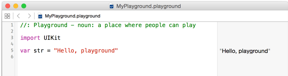
Figure 2.3 A playground
