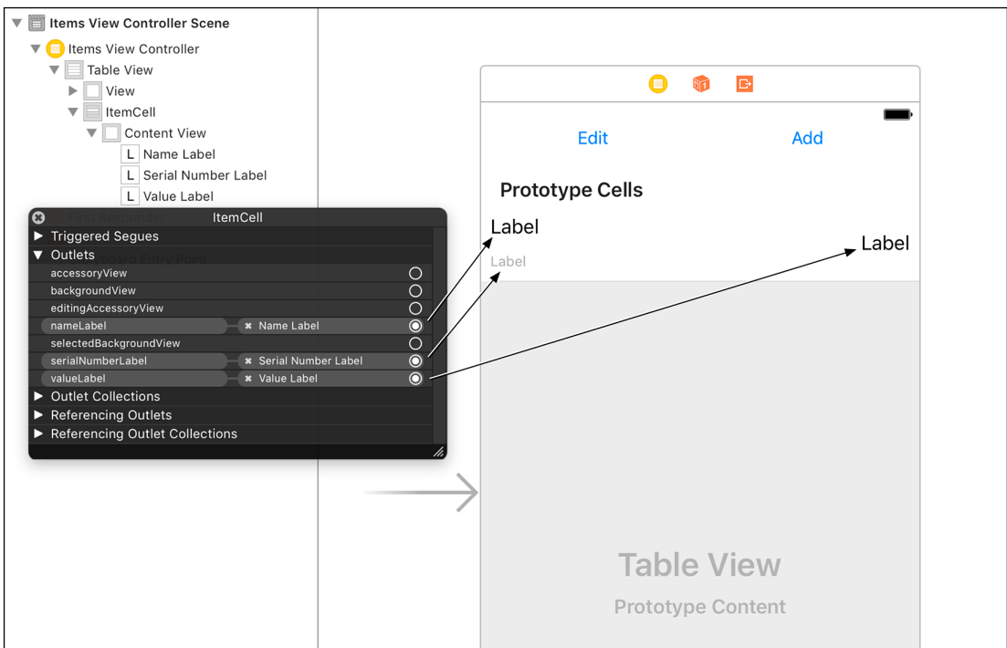
Figure 12.5 Connecting the outlets
