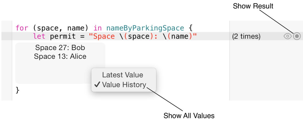
Figure 2.5 Using the Value History to see the results of string interpolation
