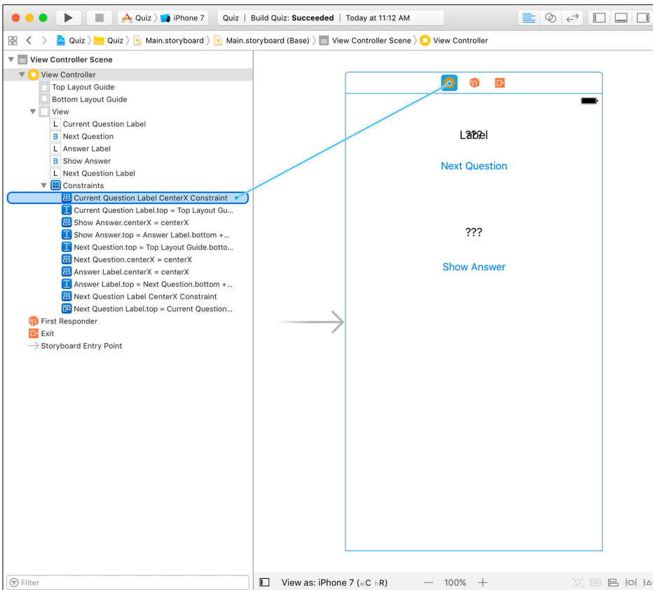
Figure 8.4 Connecting a constraint outlet
