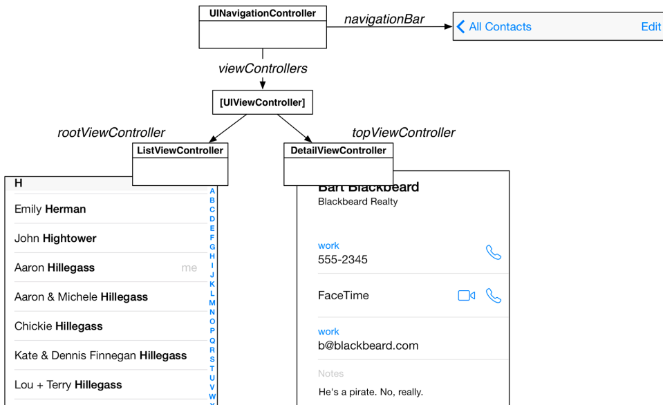
Figure 14.3 UINavigationController 's stack
