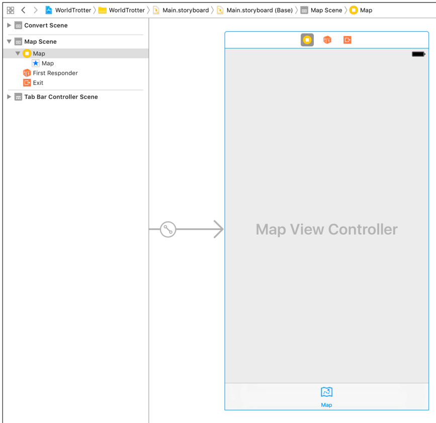
Figure 6.2 Deleting the view
