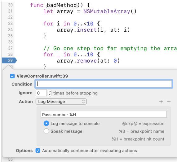
Figure 9.14 Adding a logging breakpoint
