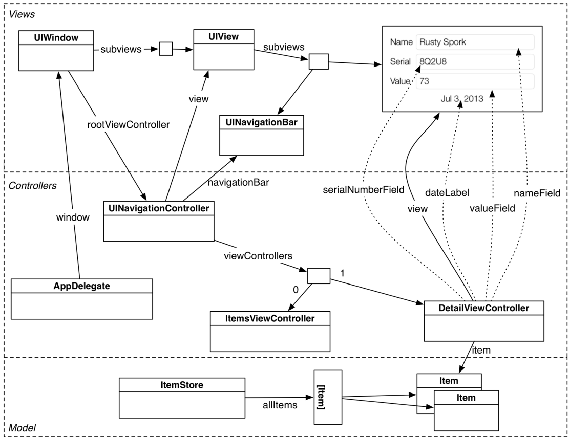
Figure 14.5 Homepwner object diagram
