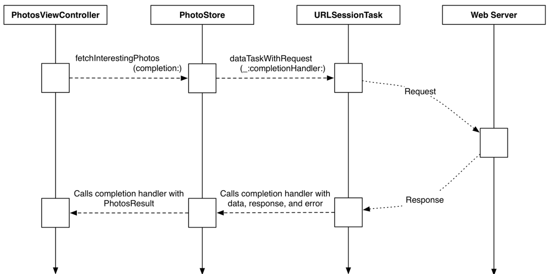
Figure 20.6 Web service request data flow
