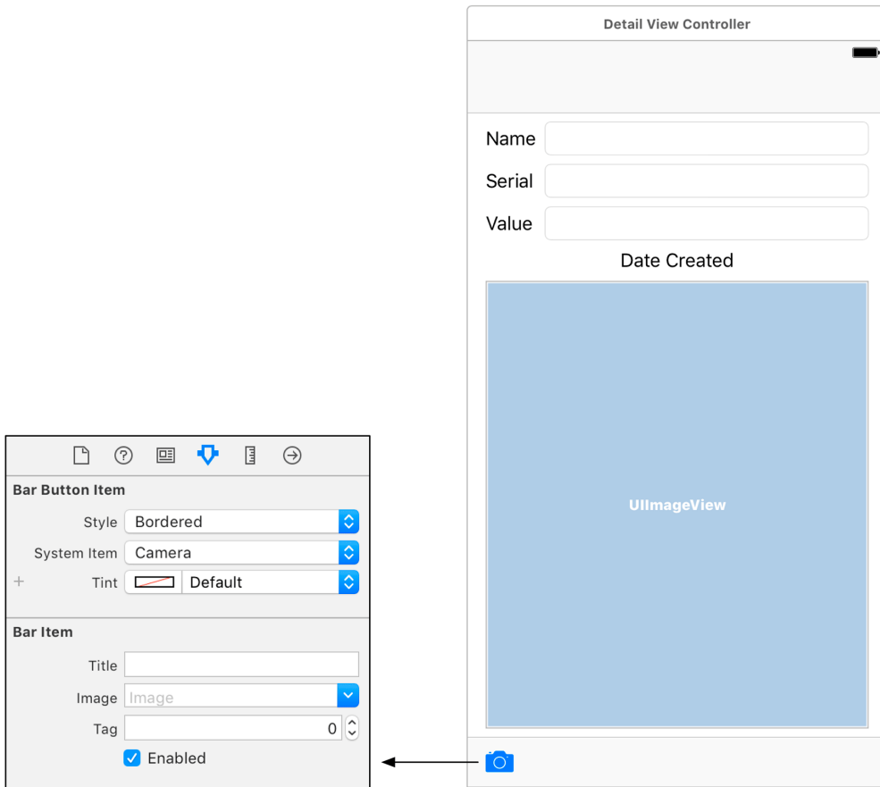
Figure 15.7 UIToolbar with camera bar button item
