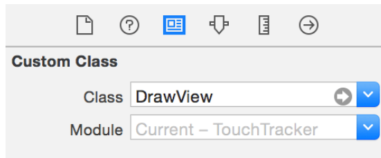
Figure 18.4 Changing the view class
