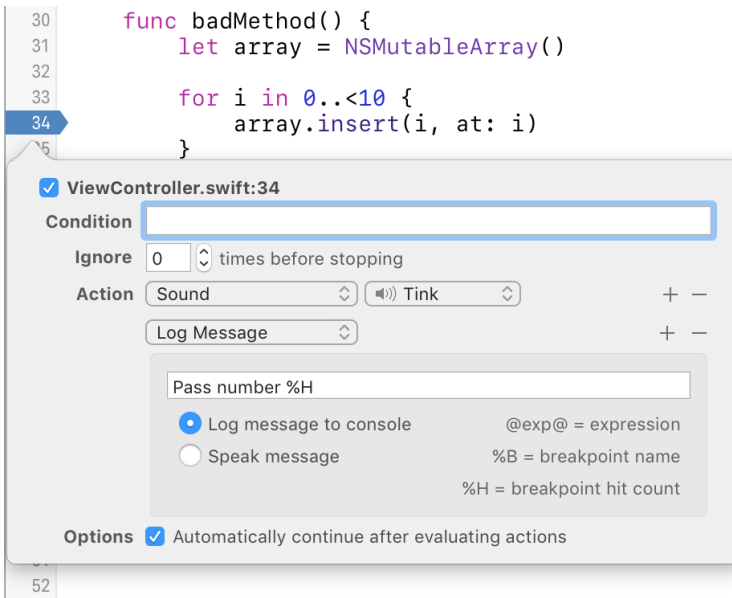
Figure 9.13 Assigning multiple actions to a breakpoint
