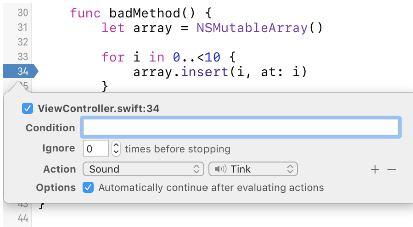
Figure 9.12 Enabling special actions
