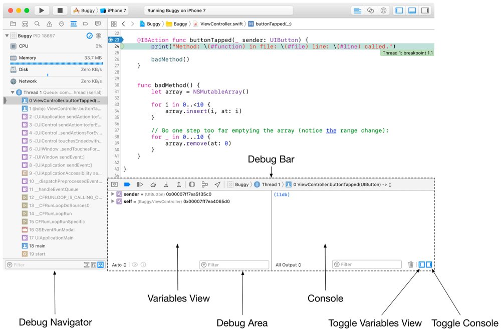
Figure 9.7 Xcode stopped at a breakpoint
