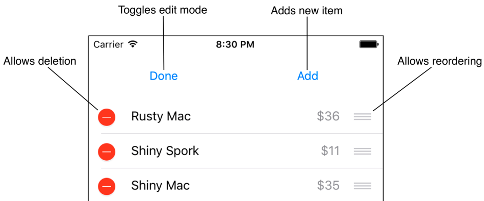
Figure 11.1 Homepwner in editing mode
