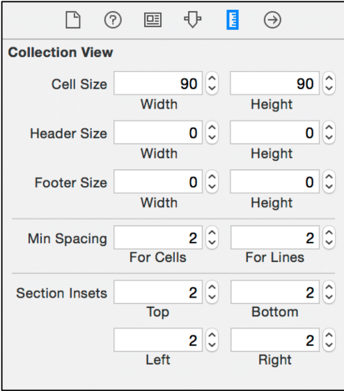
Figure 21.7 Collection view size inspector
