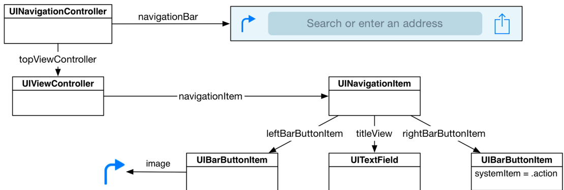
Figure 14.13 UINavigationControllerItem with everything
