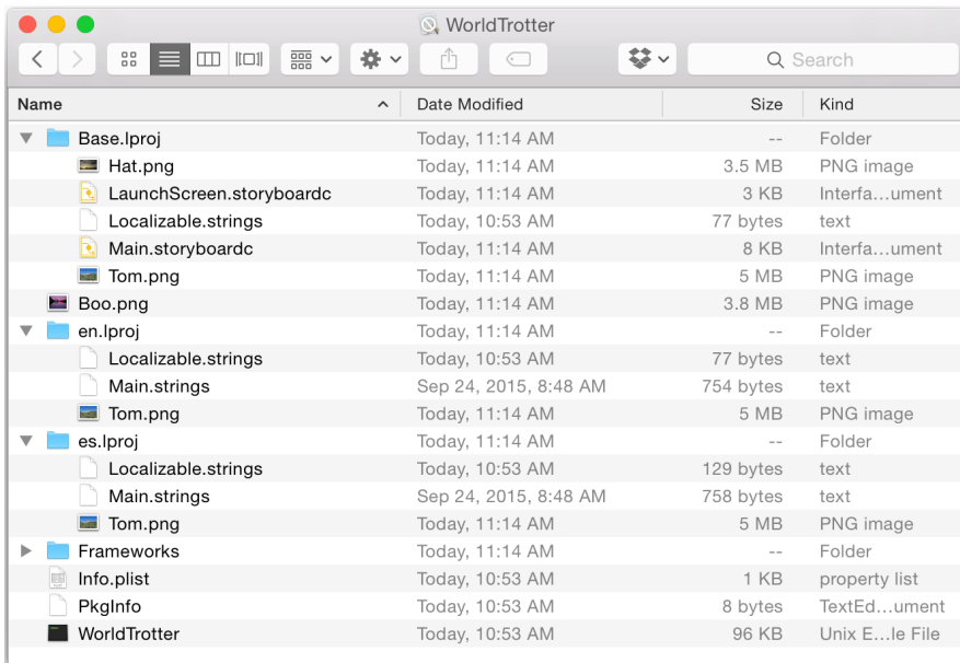
Figure 7.19 Application bundle
