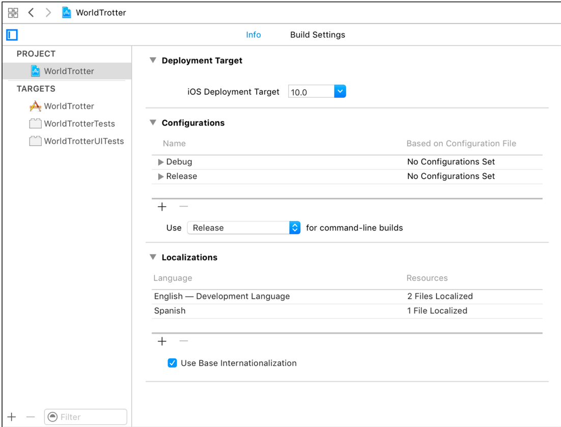
Figure 7.15 Localizations
