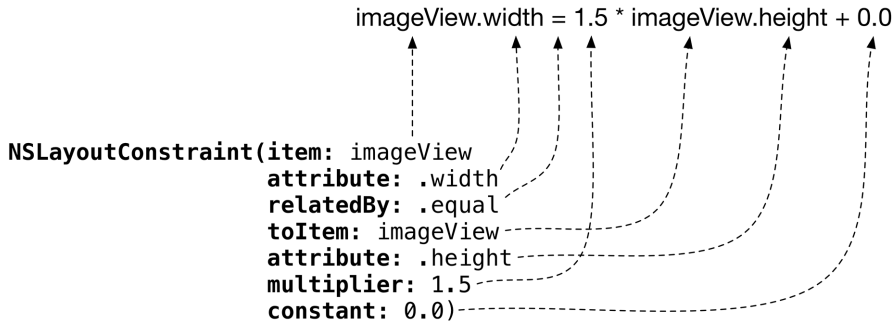
Figure 6.6 NSLayoutConstraint equation
