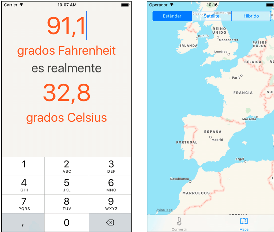
Figure 7.2 Localized WorldTrotter
