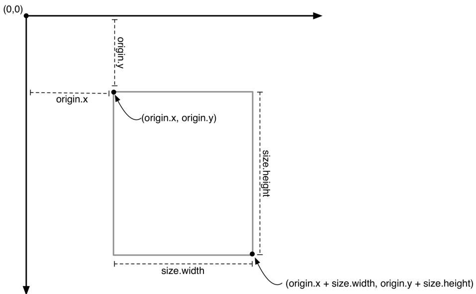
Figure 3.5 CGRect
