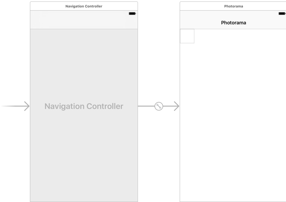
Figure 21.3 Storyboard canvas
