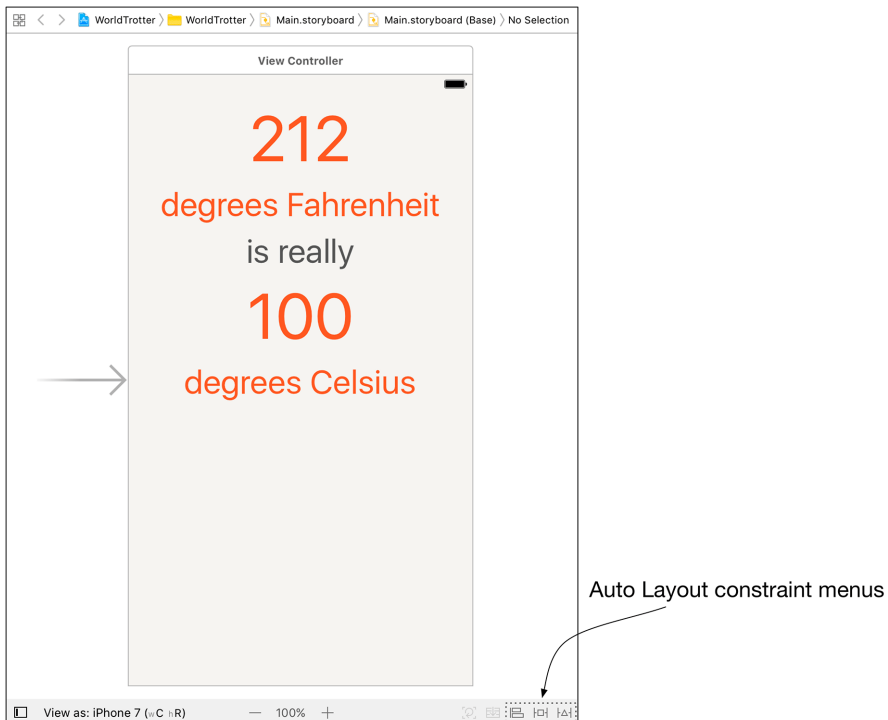
Figure 3.19 Auto Layout constraint menus
