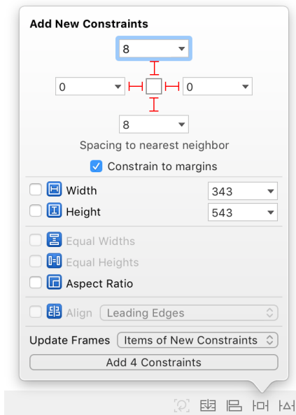
Figure 17.2 Stack view constraints
