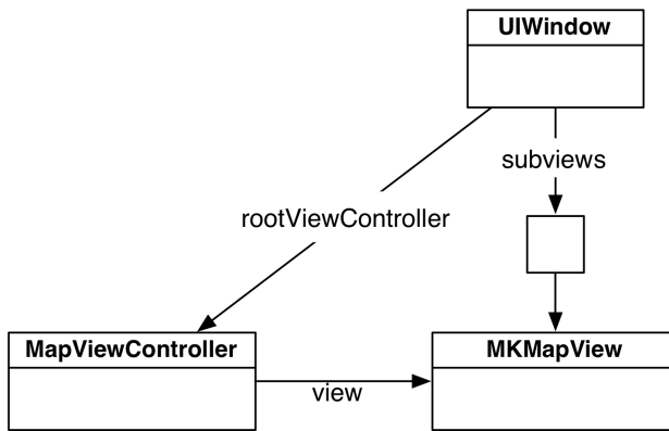
Figure 5.2 Object diagram for WorldTrotter
