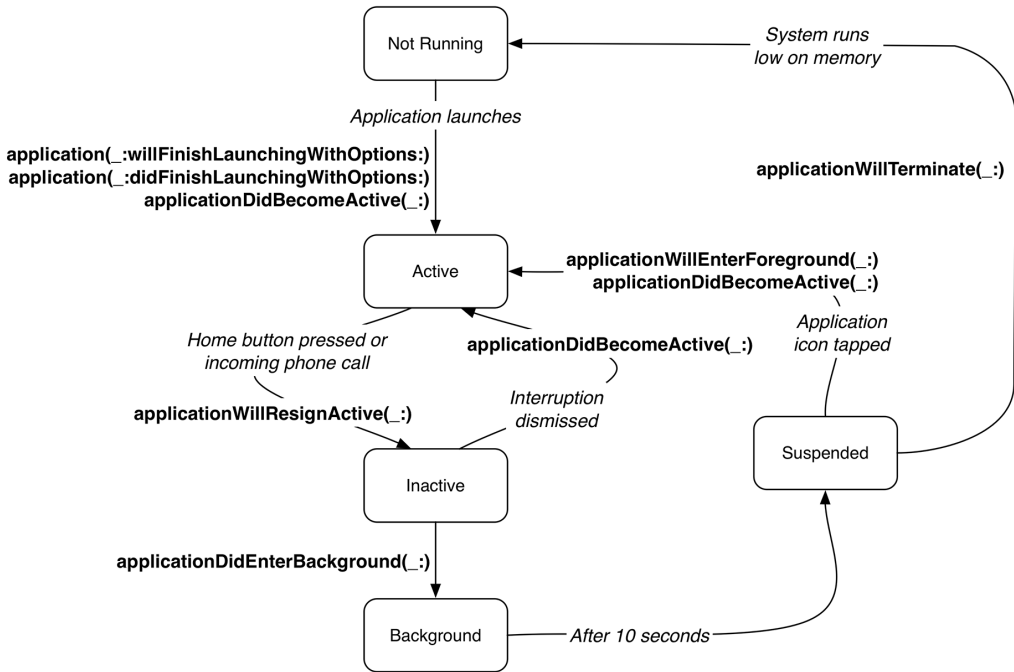
Figure 16.6 States of a typical application
