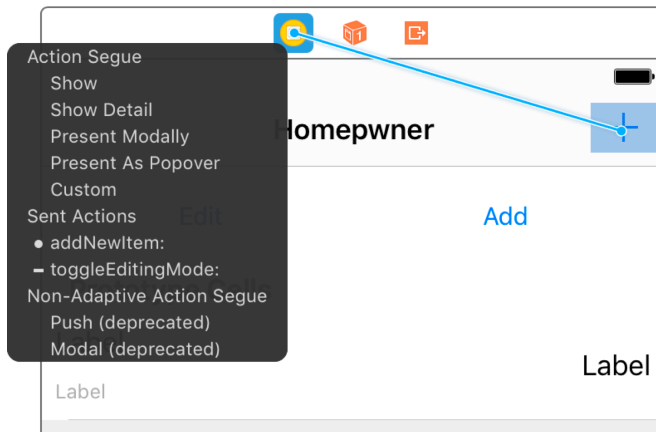
Figure 14.15 Connecting the addNewItem: action
