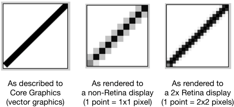
Figure 5.15 Rendering to different resolutions
