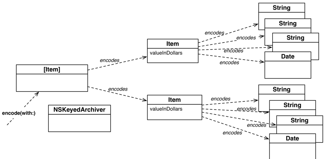
Figure 16.4 Archiving the allItems array
