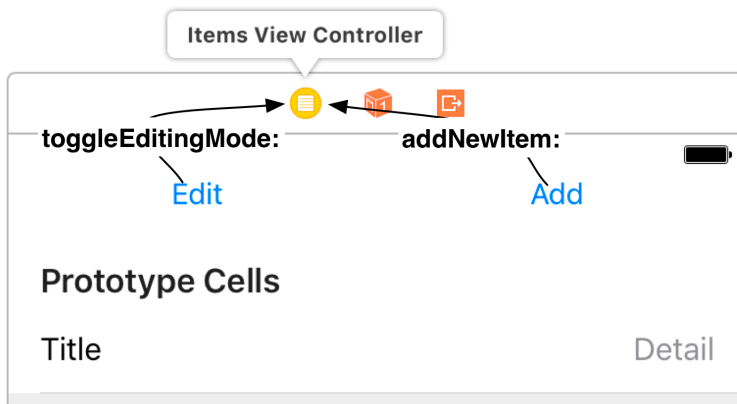
Figure 11.6 Connecting the two actions
