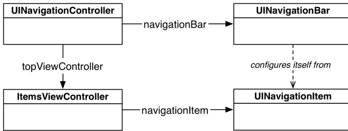
Figure 14.10 UINavigationItem
