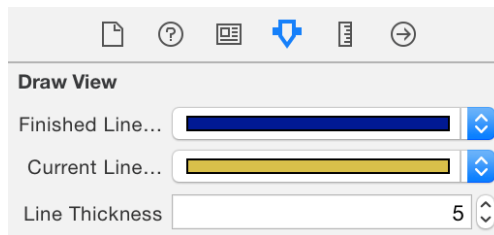
Figure 18.7 Customizing DrawView
