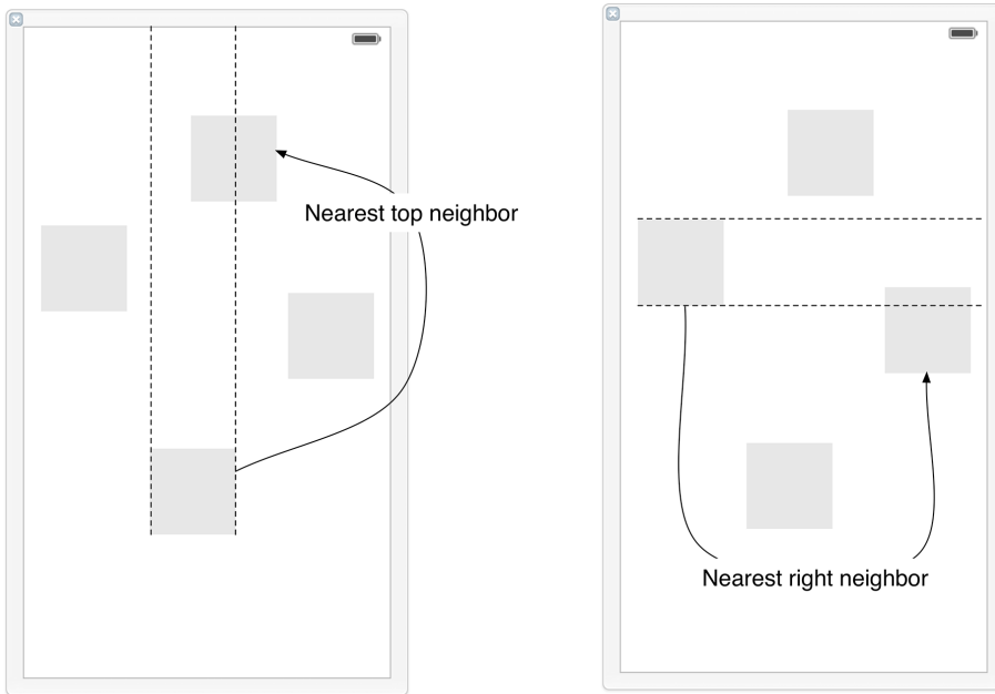
Figure 3.18 Nearest neighbor
