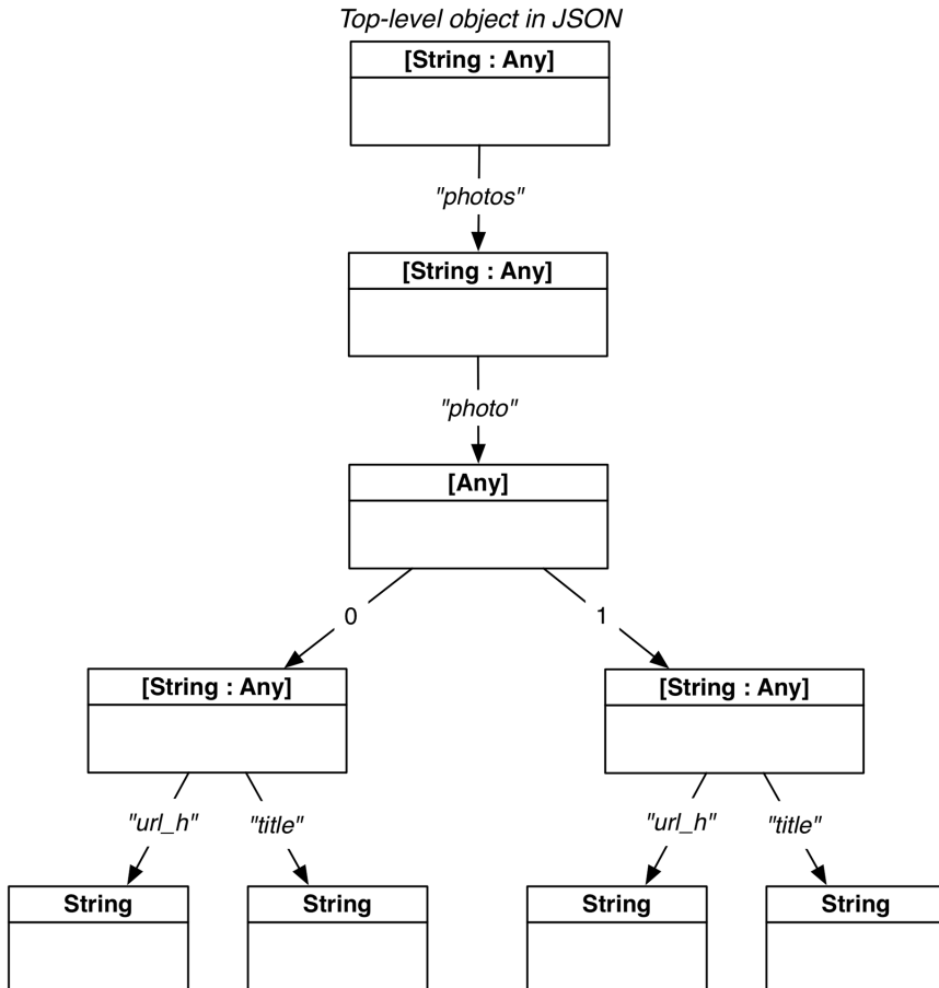
Figure 20.5 JSON objects
