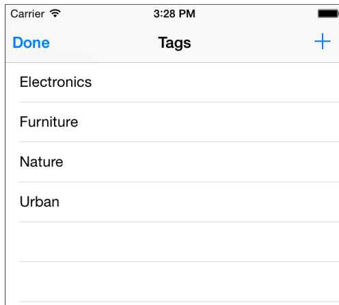
Figure 23.6 TagsViewController
