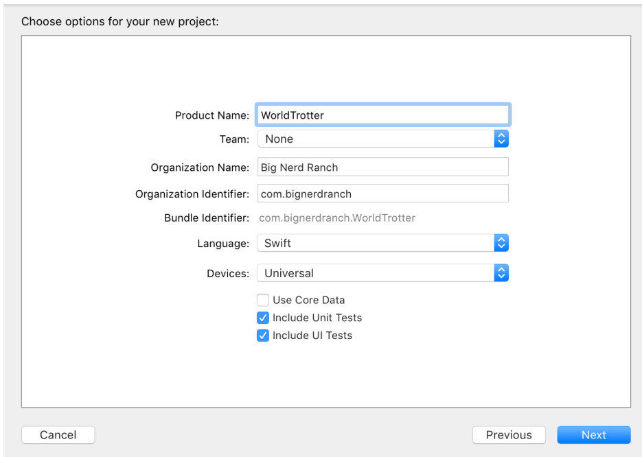
Figure 3.4 Configuring WorldTrotter
