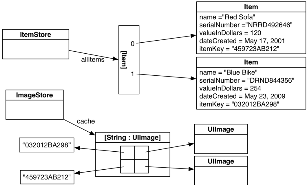
Figure 15.14 Accessing images from the cache
