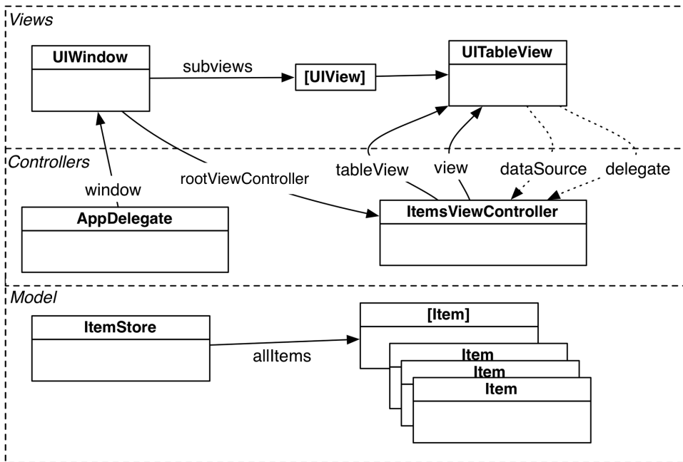
Figure 10.6 Homepwner object diagram
