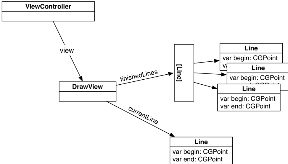
Figure 18.3 Object diagram for TouchTracker
