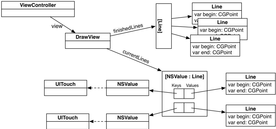
Figure 18.6 Object diagram for multitouch TouchTracker
