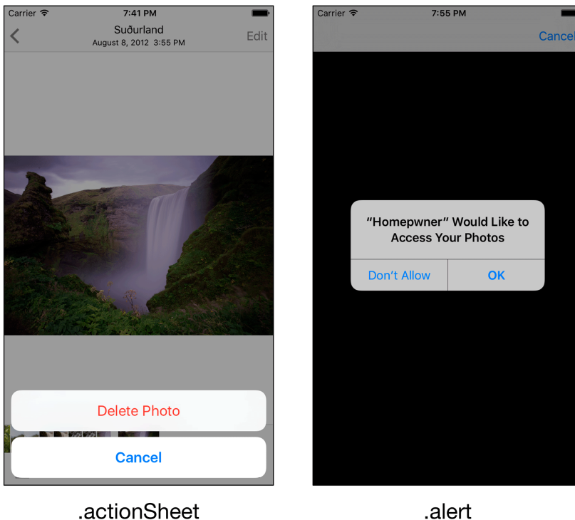
Figure 11.9 UIAlertController styles
