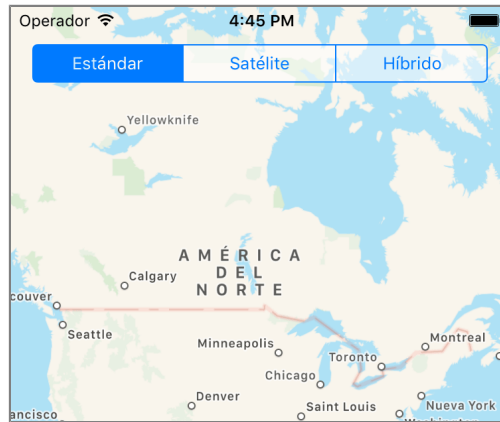
Figure 7.18 Spanish MapViewController
