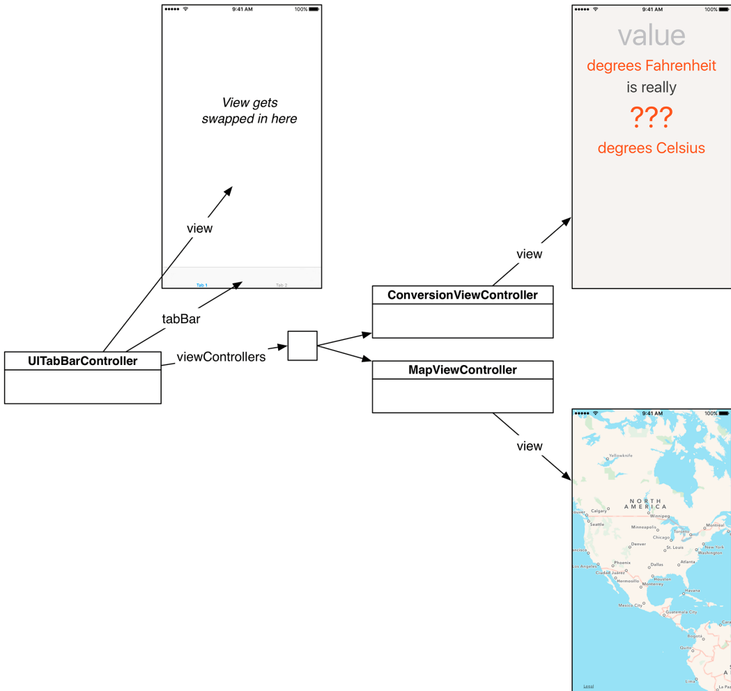
Figure 5.10 UITabBarController diagram
