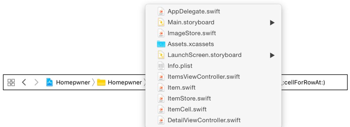
Figure 15.17 File popover
