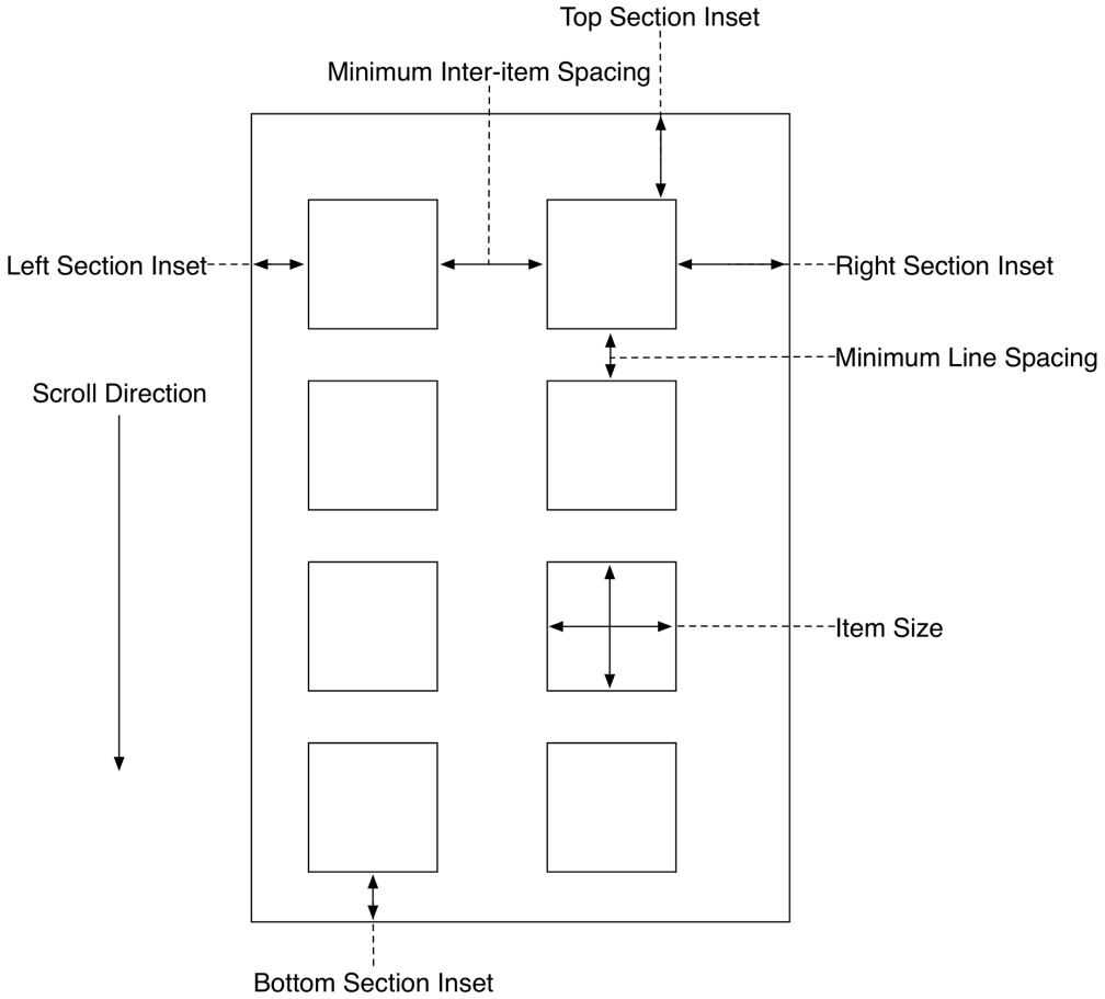
Figure 21.6 UICollectionViewFlowLayout properties
