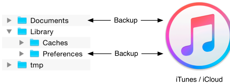
Figure 16.3 Application sandbox
