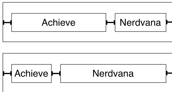
Figure 13.5 Ambiguous layout
