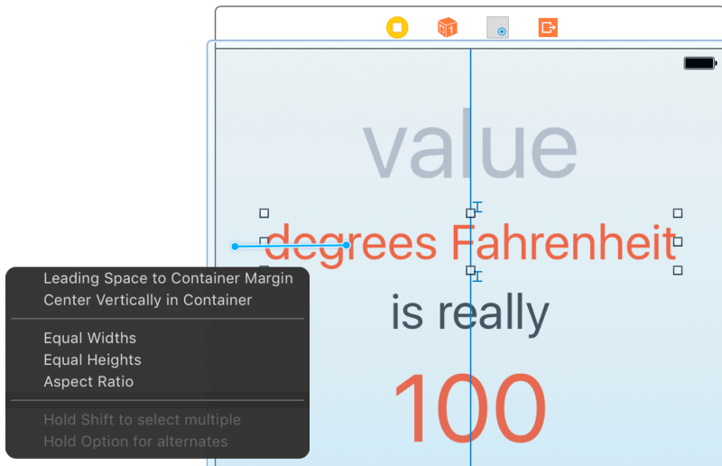
Figure 7.9 Creating constraints by Control-dragging
