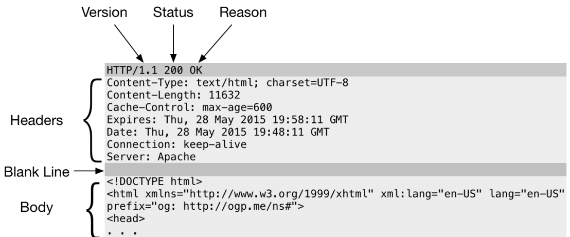
Figure 20.8 HTTP response format
