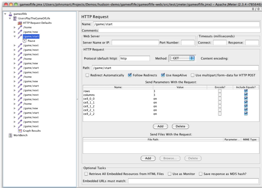
Figure 6.24. Preparing a performance test script in JMeter
