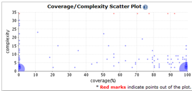
Figure 9.14. A coverage/complexity scatter plot
