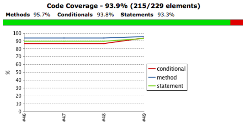
Figure 6.18. Clover code coverage trends
