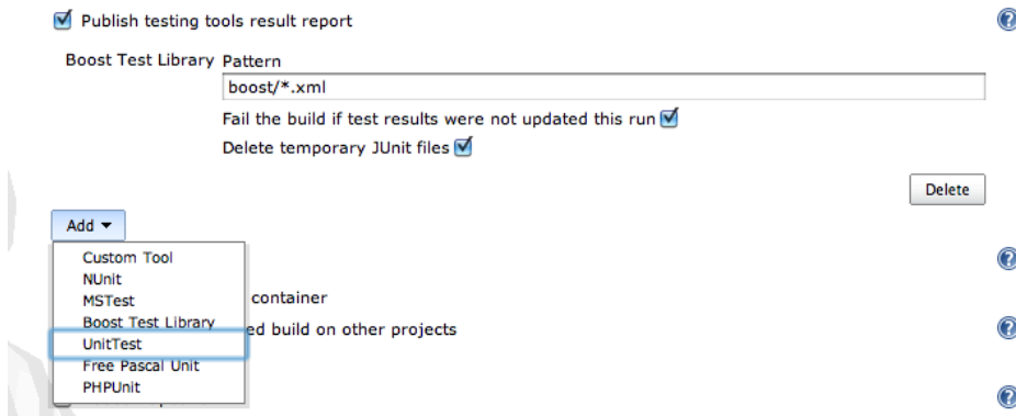
Figure 6.4. Publishing xUnit test results
