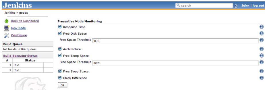
Figure 11.16. Jenkins proactively monitors your build agents
