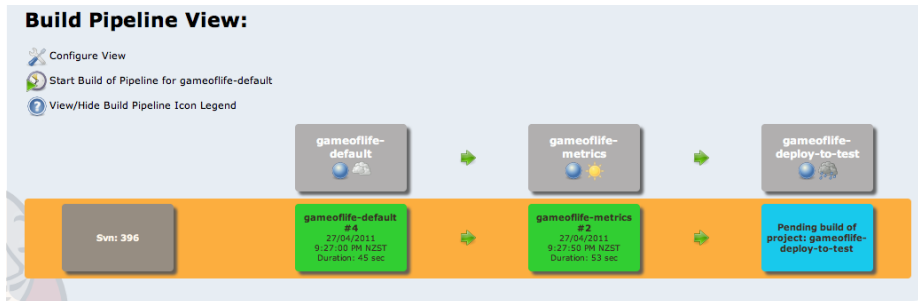
Figure 12.1. A simple automated deployment pipeline
