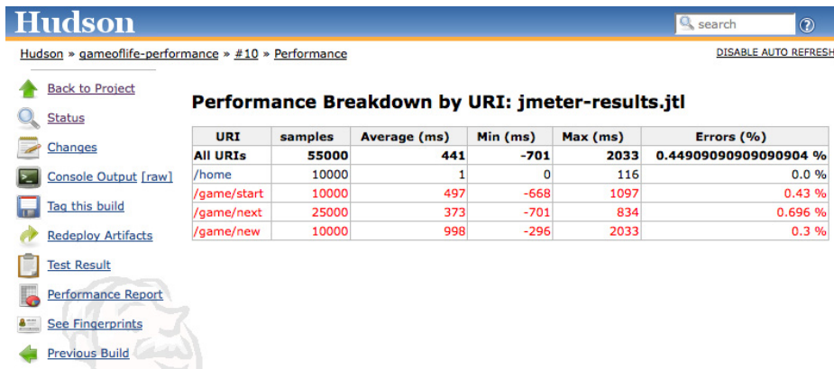
Figure 6.30. You can also view performance results per request
