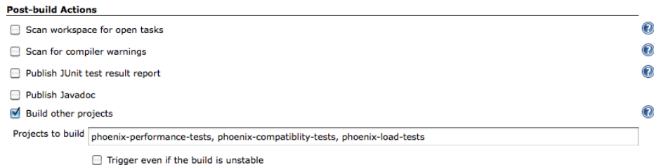
Figure 10.30. Triggering several other builds after a build job
