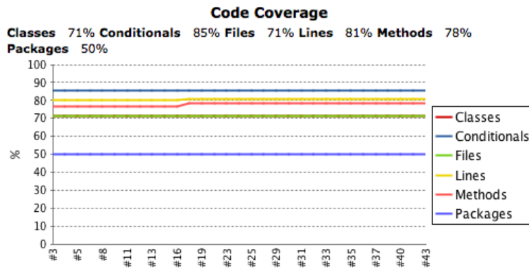
Figure 6.15. Configuring the test coverage metrics in Jenkins
