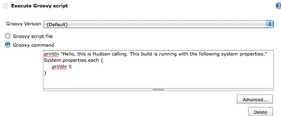
Figure 5.30. Running Groovy commands as part of a build job
