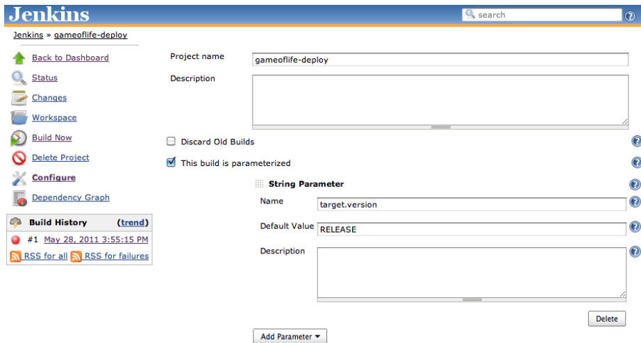
Figure 12.11. Deploying an artifact from a Maven repository
