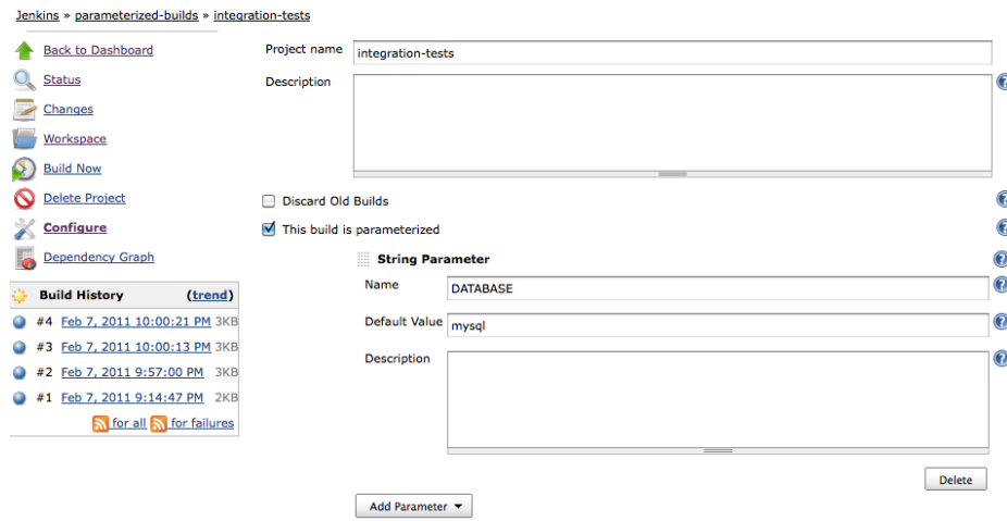
Figure 10.17. The build job you trigger must also be a parameterized build job
