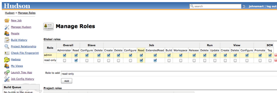
Figure 7.25. Managing global roles
