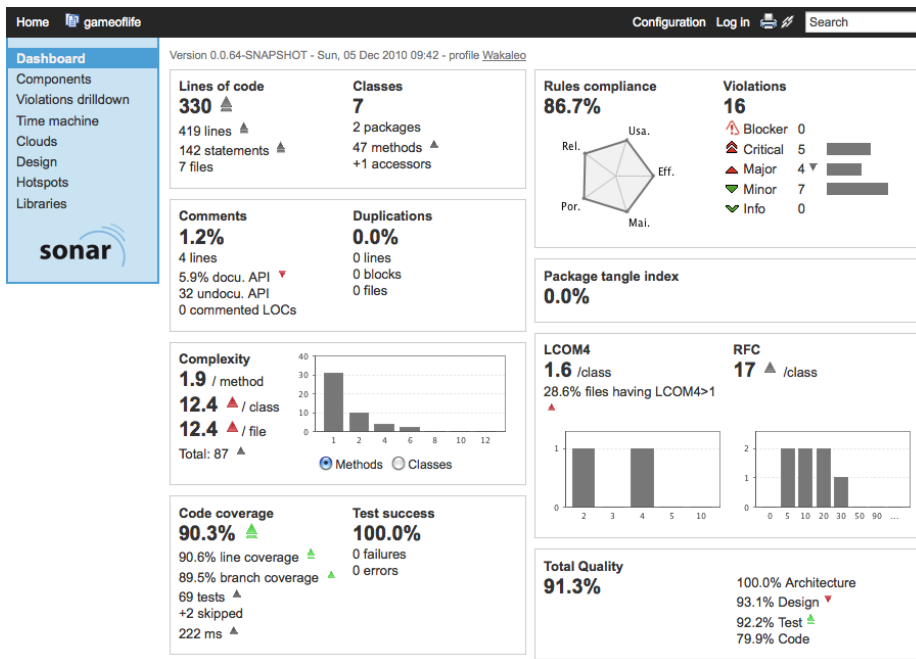
Figure 9.18. Code quality reporting by Sonar
