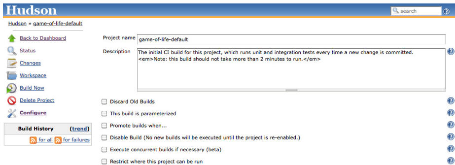
Figure 5.2. Creating a new build job
