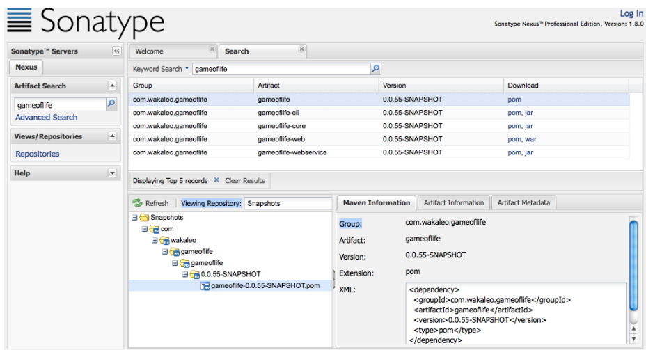
Figure 5.41. After deployment the artifact should be available on your Enterprise Repository Manager
