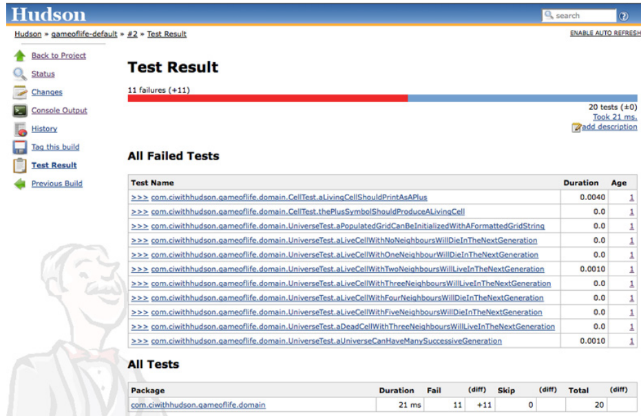
Figure 2.22. The list of all the broken tests
