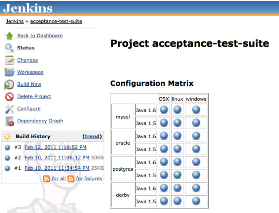
Figure 10.24. Multiconfiguration build results
