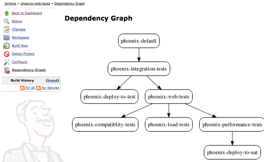
Figure 10.31. A build job dependency graph
