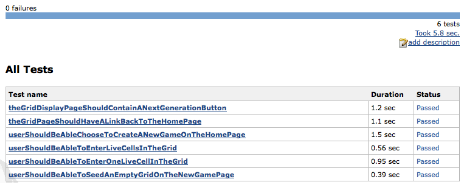
Figure 6.19. Using business-focused, behavior-driven naming conventions for JUnit tests
