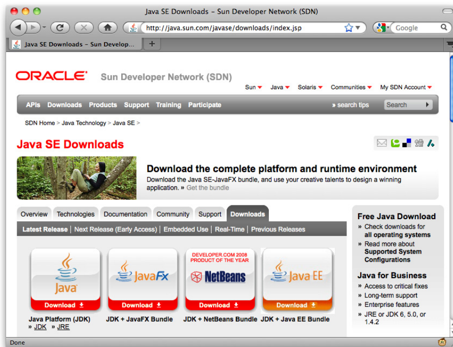
Figure 2.1. Installing Java
