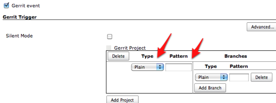
Figure 5.18. Gerrit Trigger
