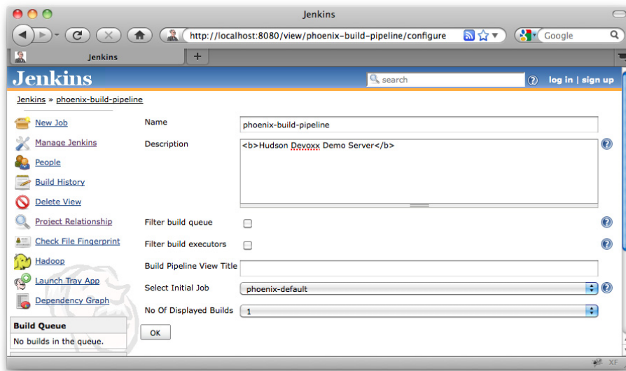
Figure 10.57. Configuring a Build Pipeline view
