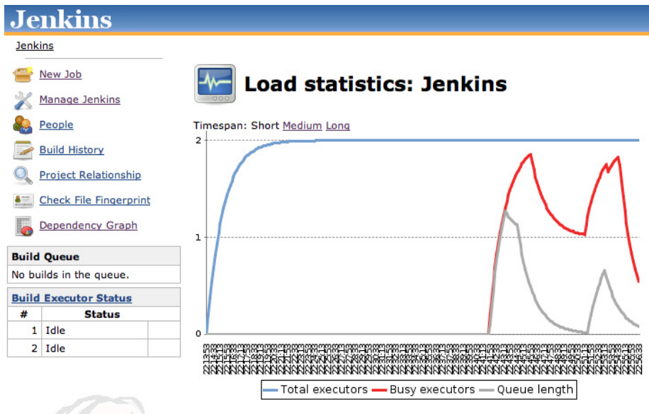
Figure 13.7. Jenkins Load Statistics
