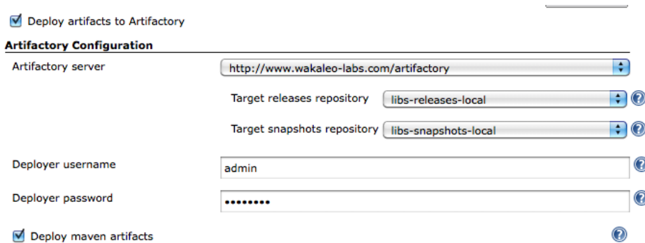
Figure 5.43. Deploying to Artifactory from Jenkins
