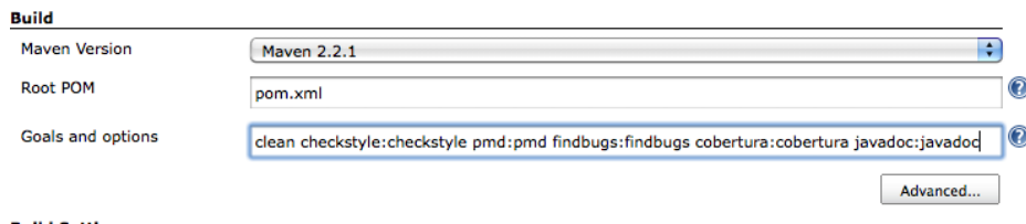
Figure 9.3. Generating code quality reports in a Maven build
