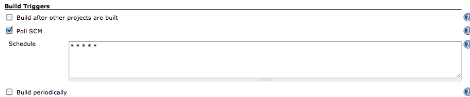
Figure 2.16. Scheduling the build jobs
