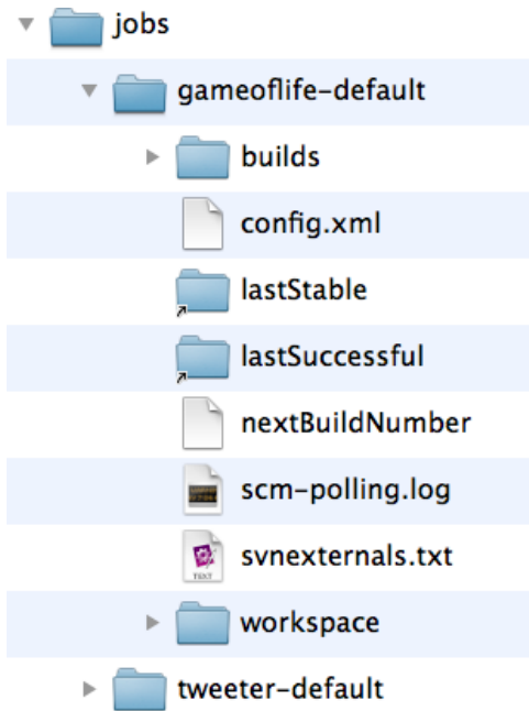
Figure 3.8. The Jenkins jobs directory
