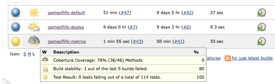
Figure 6.14. Test coverage results contribute to the project status on the dashboard
