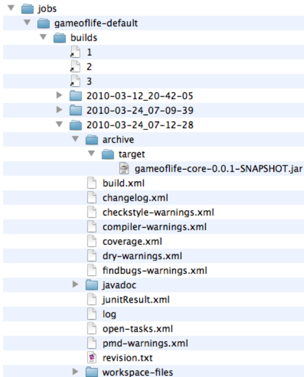
Figure 3.9. The builds directory
