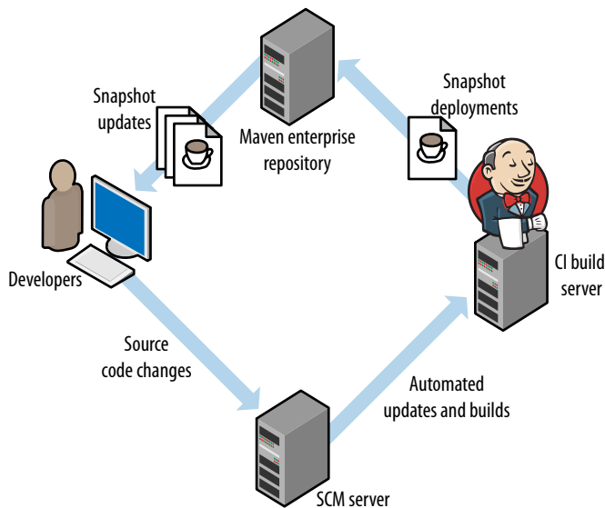
Figure 12.10. Using a Maven Enterprise Repository
