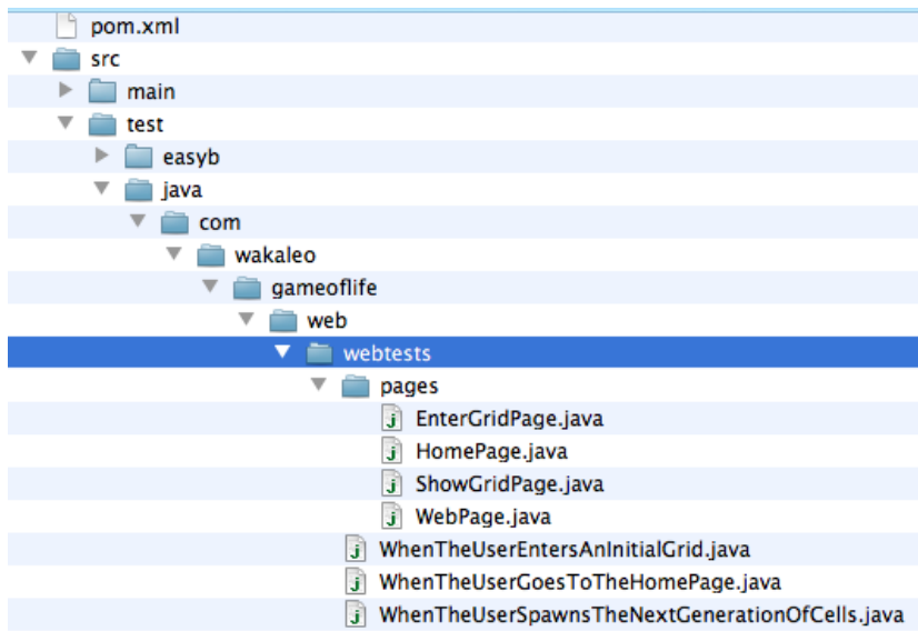
Figure A.1. A project containing freely-named test classes
