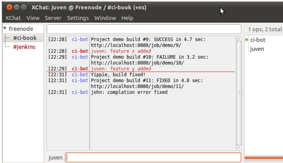
Figure 8.17. IRC notification messages in action
