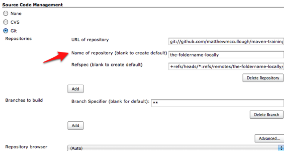
Figure 5.10. Advanced configuration of a Git repo URL
