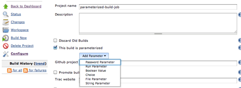
Figure 10.1. Creating a parameterized build job
