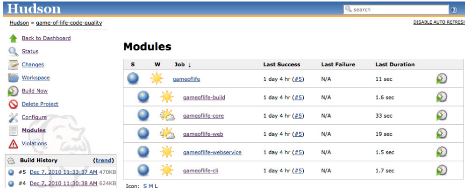
Figure 9.9. Jenkins Maven build jobs understand Maven multimodule structures
