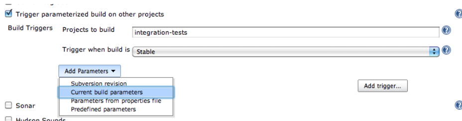
Figure 10.16. Adding a parameterized trigger to a build job
