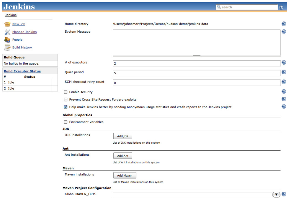
Figure 2.9. The Configure Jenkins screen
