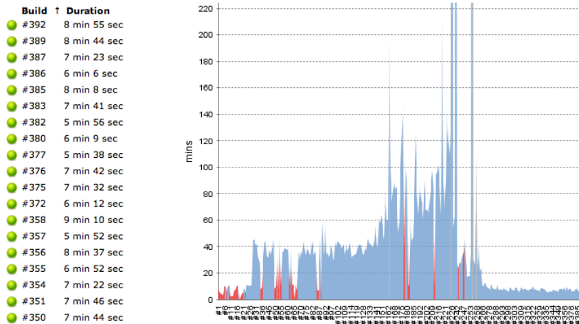
Figure 6.8. Build time trends can give you a good indicator of how fast your tests are running
