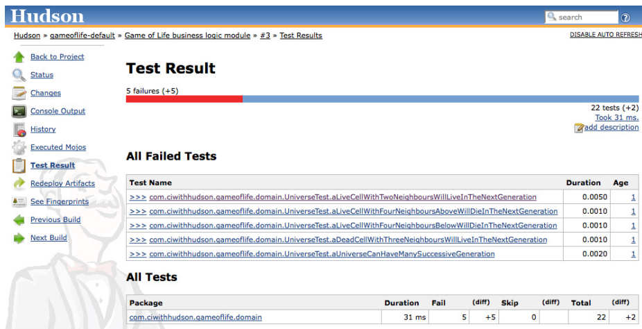
Figure 6.6. Jenkins displays a summary of the test results
