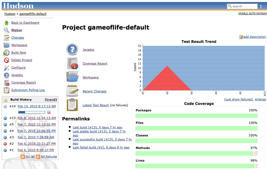
Figure 2.30. Jenkins displays code coverage metrics on the build home page
