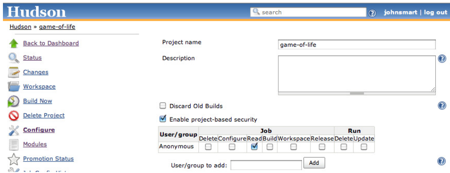
Figure 7.20. Configuring project-based security
