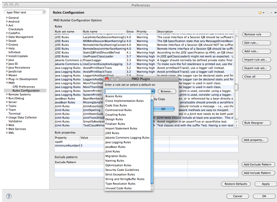
Figure 9.2. Configuring PMD rules in Eclipse
