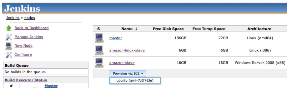
Figure 11.21. Bringing an Amazon EC2 slave online manually
